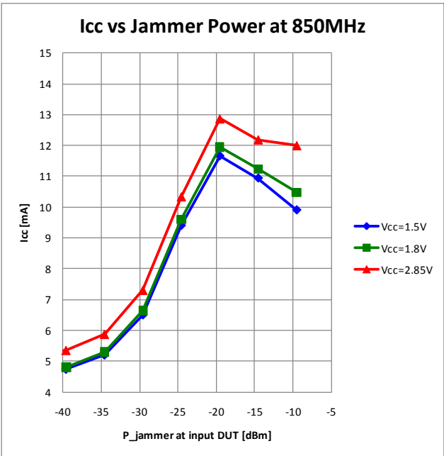
Fig 12. Icc versus jammer power
