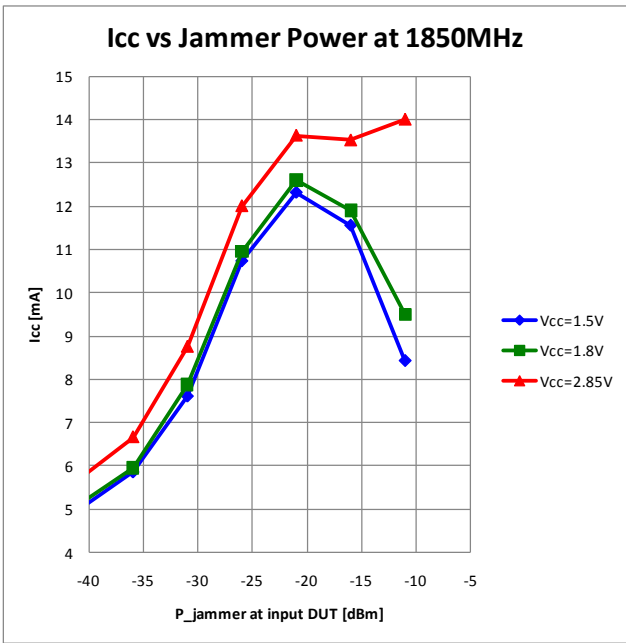
Fig 13. Icc versus jammer power
