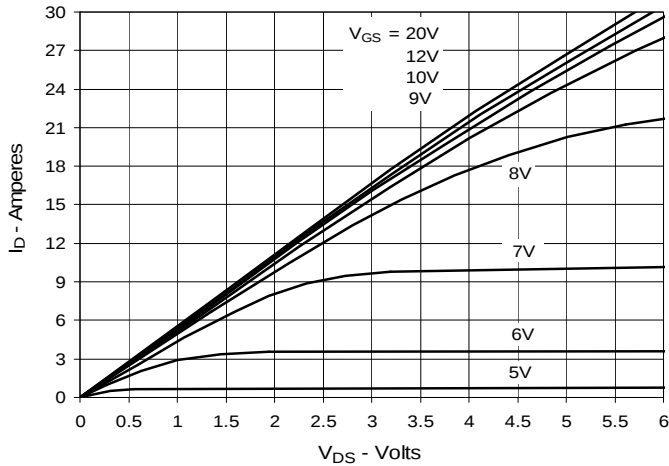
Fig. 3. Output Characteristics
