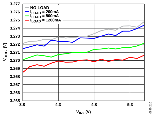
Figure 9. Buck Regulator Line Regulation, V_{OUT2} = 3.3\text{ V}
