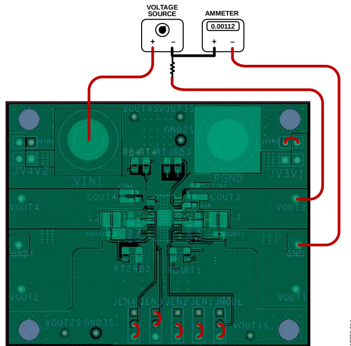
Figure 17. Ground Current Measurement
