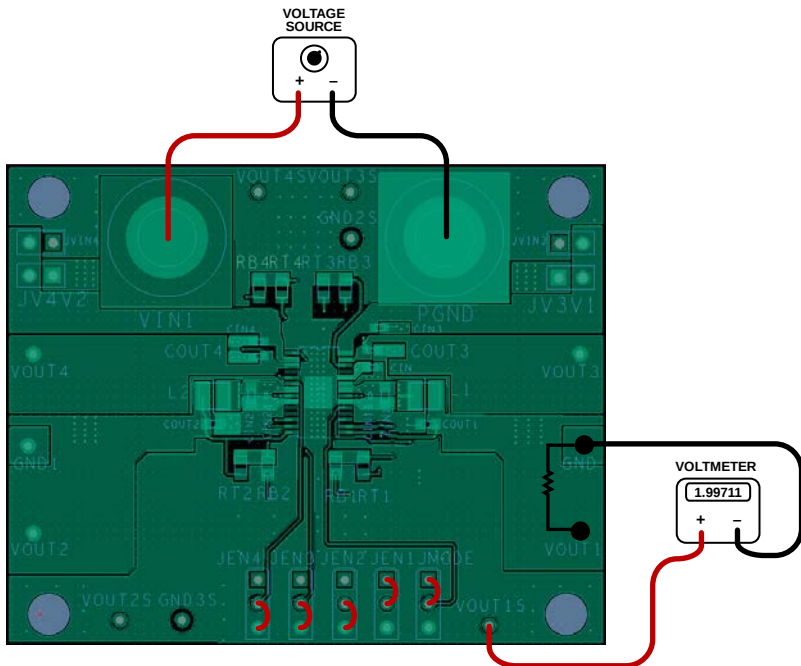
Figure 16. Output Voltage Measurement
