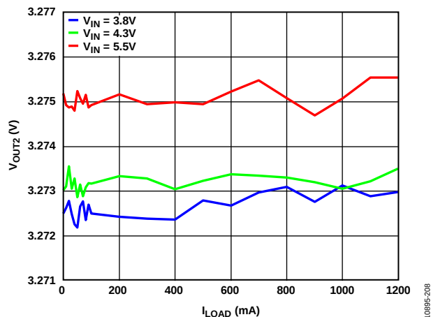
Figure 7. Buck Load Regulation, V_{OUT2} = 3.3\text{ V}
