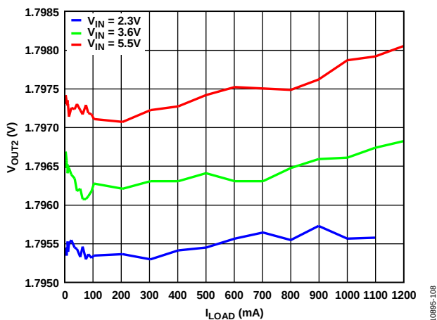
Figure 8. Buck Load Regulation, V_{OUT2} = 1.8\text{ V}
