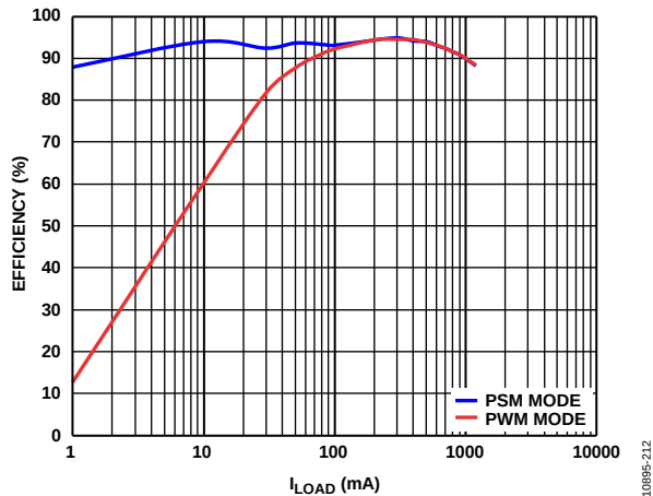
Figure 11. Buck Regulator Efficiency, V_{IN2} = 4.2\text{ V} , V_{OUT2} = 3.3\text{ V}
