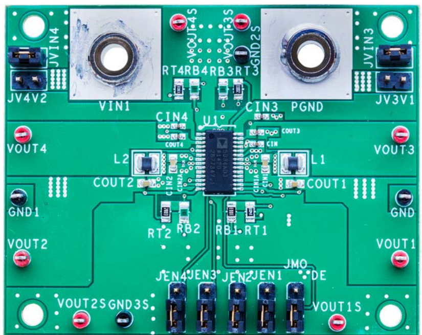
Figure 19. Evaluation Board of the ADP5034 TSSOP
