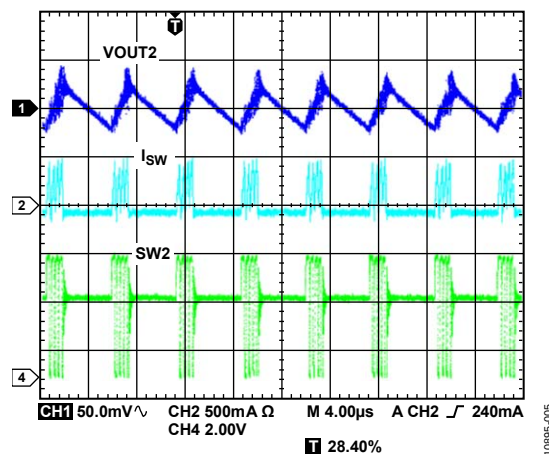
Figure 5. Typical Waveforms, V OUT2 = 3.3 V, I OUT2 = 30 mA, PSM Mode
