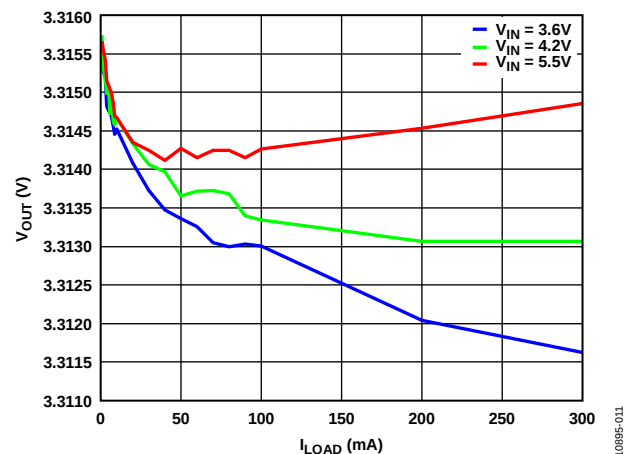
Figure 14. V_{OUT} vs. I_{LOAD} LDO Load Regulation
