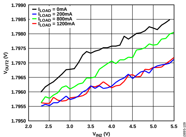
Figure 10. Buck Regulator Line Regulation, V_{OUT2} = 1.8\text{ V}
