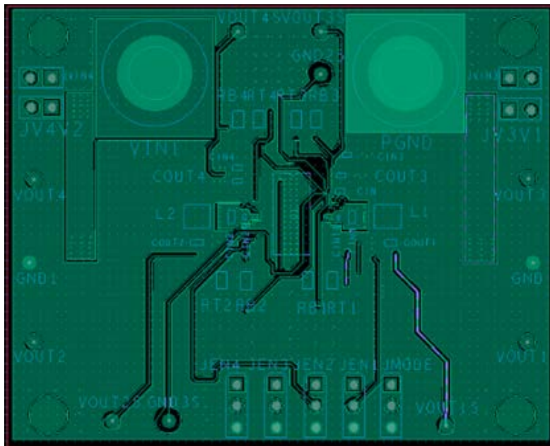
Figure 21. Bottom Layer, Recommended Layout for ADP5034 TSSOP
