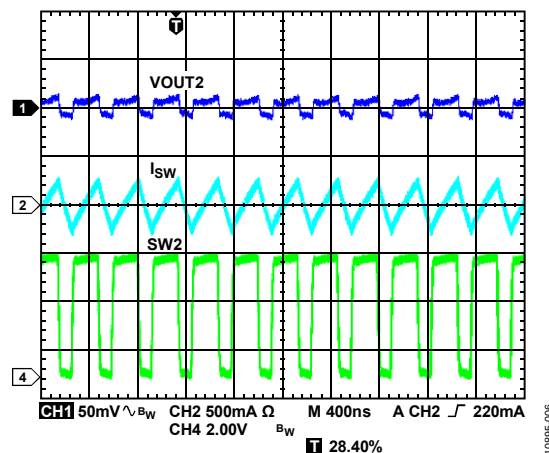
Figure 6. Typical Waveforms, V OUT2 = 3.3 V, I OUT2 = 30 mA, PWM Mode
