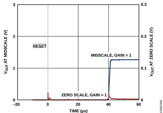
Figure 38. Hardware Reset
