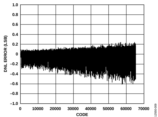
Figure 7. DNL Error vs. Code
