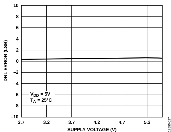
Figure 13. DNL Error vs. Supply Voltage
