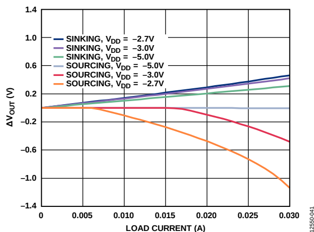
Figure 20. Headroom/Footroom ( \Delta V_{out} ) vs. Load Current
