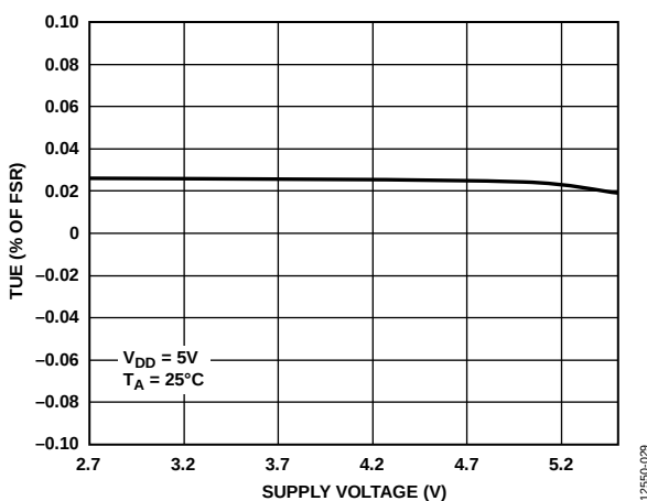
Figure 14. TUE vs. Supply Voltage
