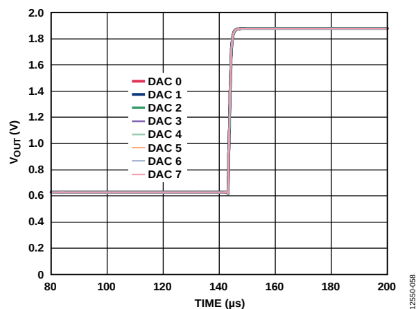
Figure 37. Settling Time, 5.5 V
