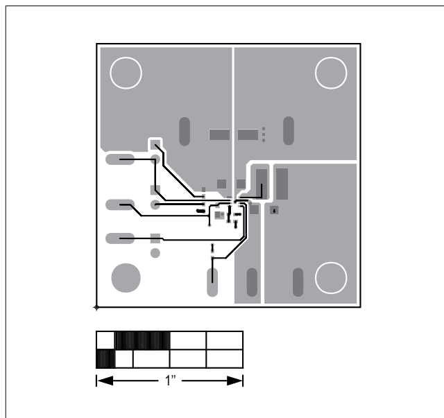
Figure 2. MAX15462C 12V EV Kit PCB Layout—Component Side
