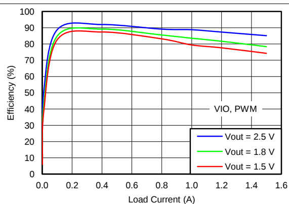
Figure 9. VIO Efficiency vs Load Current, 25°C, V_{OUT} = 2.5 V, V_{IN} = 4 V, PWM
