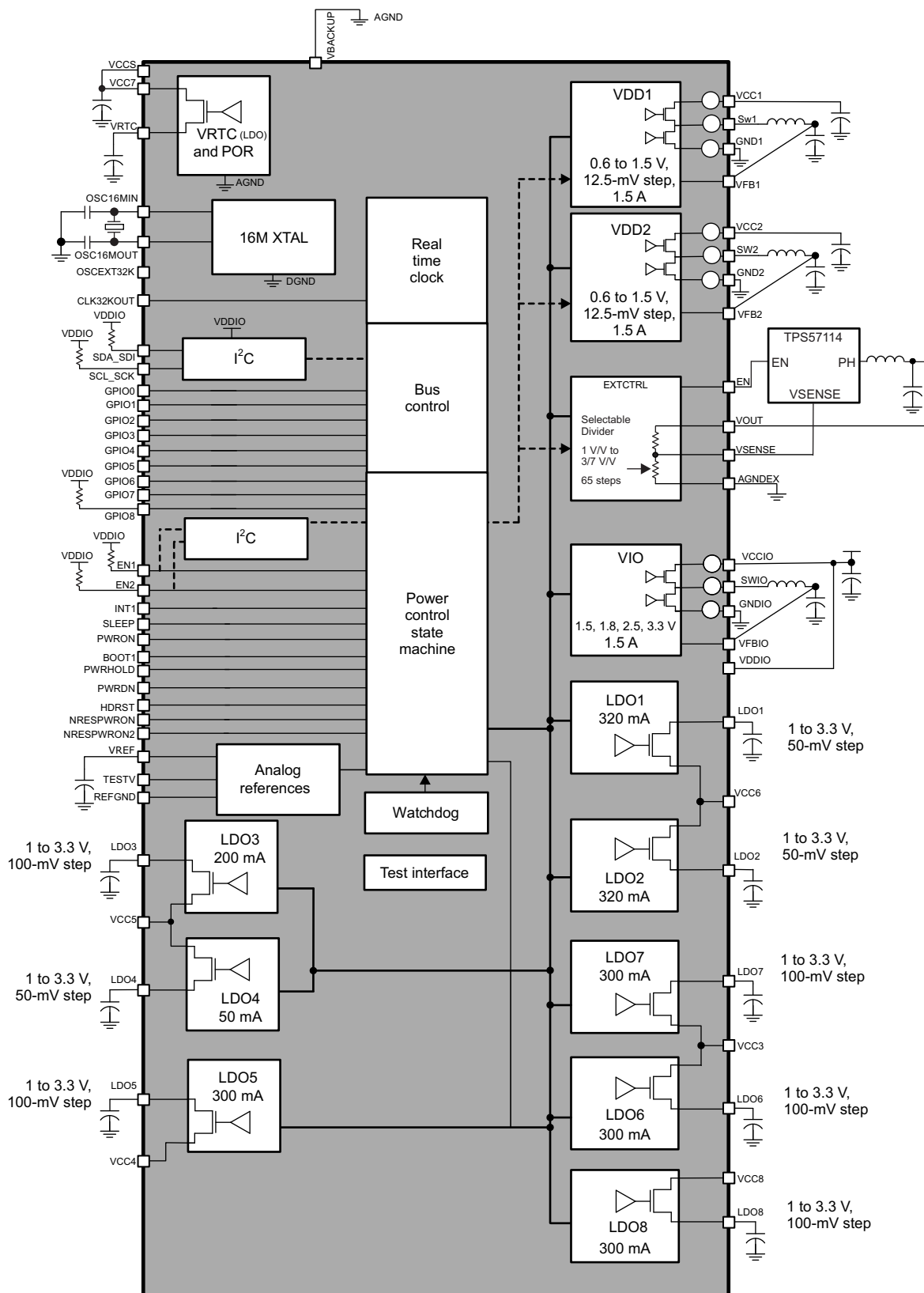
Figure 14. Top-Level Diagram
