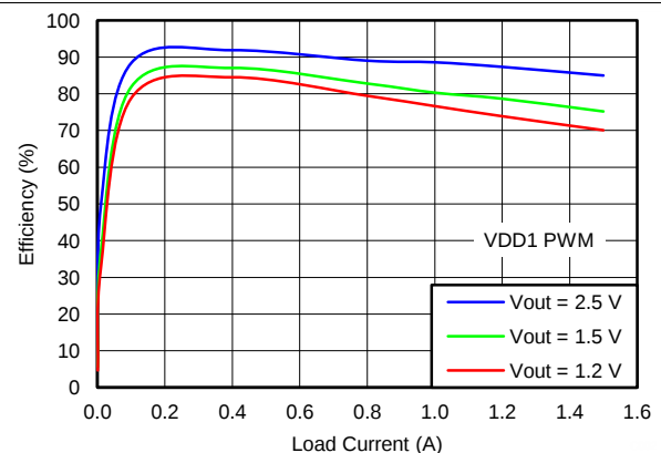
Figure 29. VDD1 Efficiency vs Load Current, 25°C, V_{IN} = 4 V, PWM
