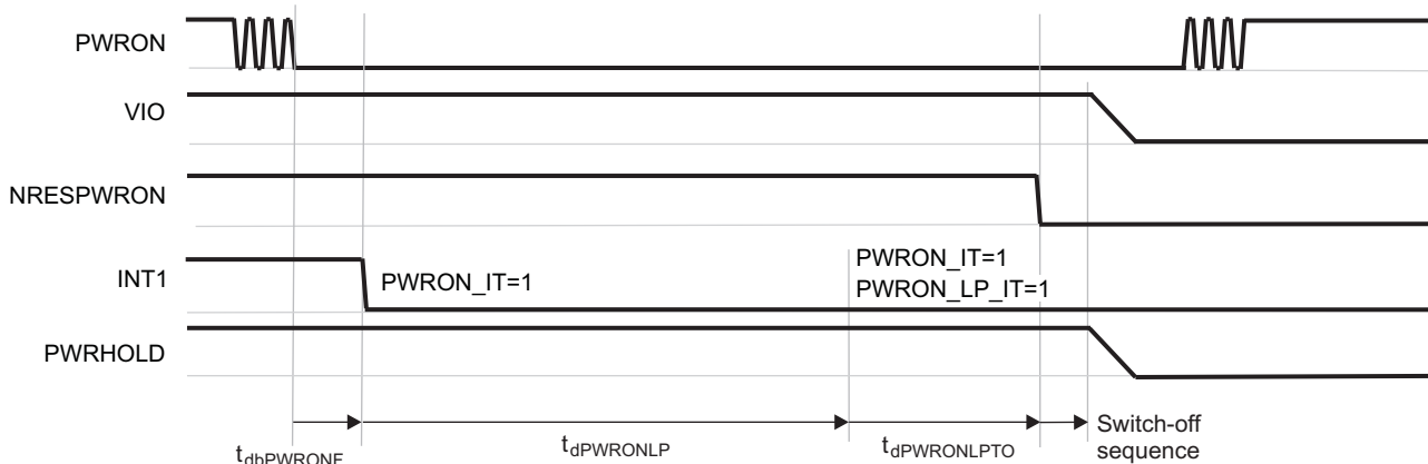
Figure 3. PWRON Long-Press Turn-Off
