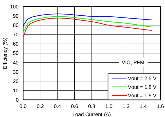
Figure 8. VIO Efficiency vs Load Current, 25°C, V_{IN} = 4 V, PFM
