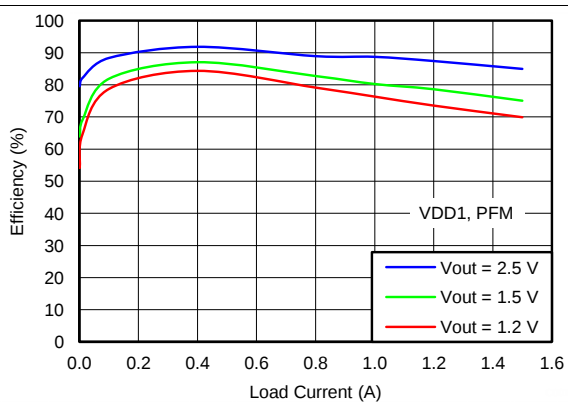
Figure 10. VDD1 Efficiency vs Load Current, 25°C, V_{IN} = 4 V, PFM
