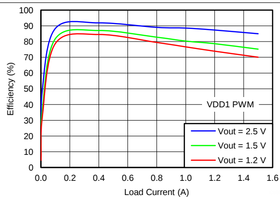
Figure 11. VDD1 Efficiency vs Load Current, 25°C, V_{IN} = 4 V, PWM
