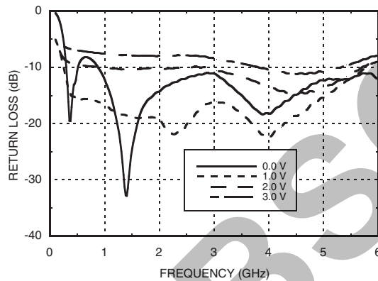
Output Return Loss Over Vctl [1]
