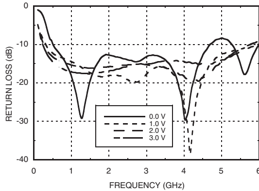
Input Return Loss Over Vctl [1]
