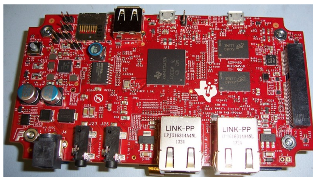
Figure 2. AM437x StarterKit EVM Bottom View
