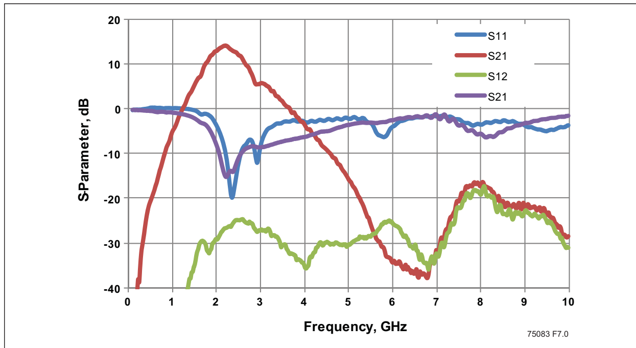
FIGURE 6-7: RECEIVER S-PARAMETER
