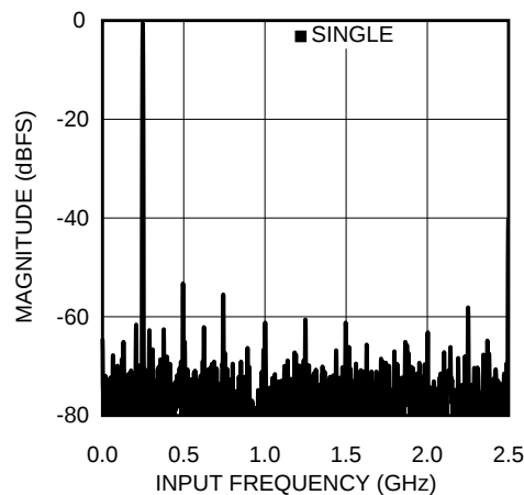
Spectral Response at F_{IN} = 248\text{ MHz}
