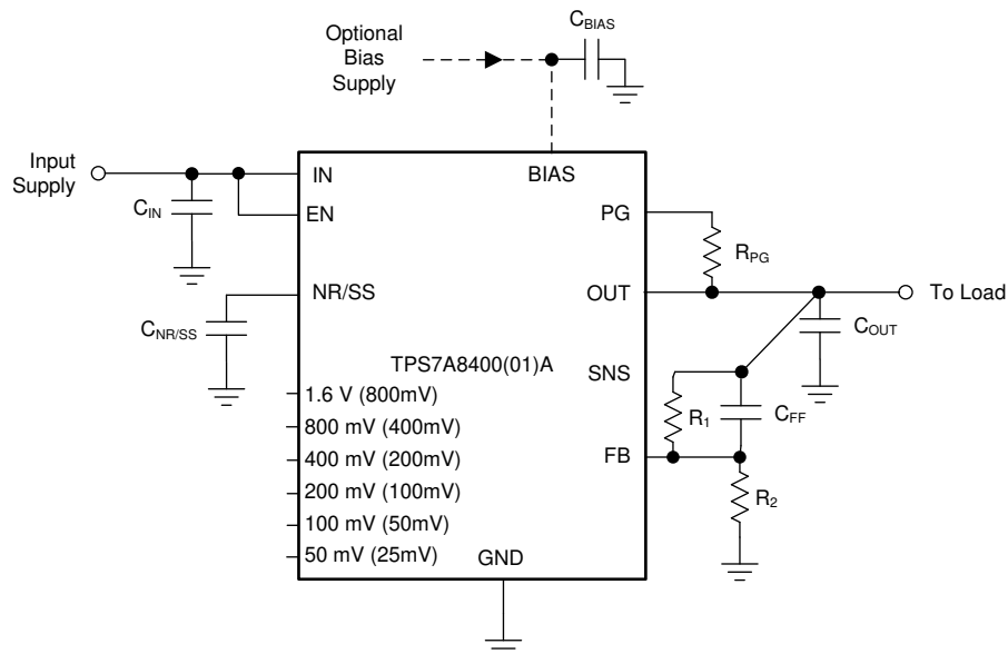
Figure 95. Adjustable Operation
