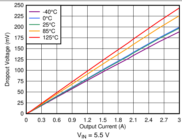
Figure 24. Dropout Voltage vs I_{OUT} (High V_{IN} )
