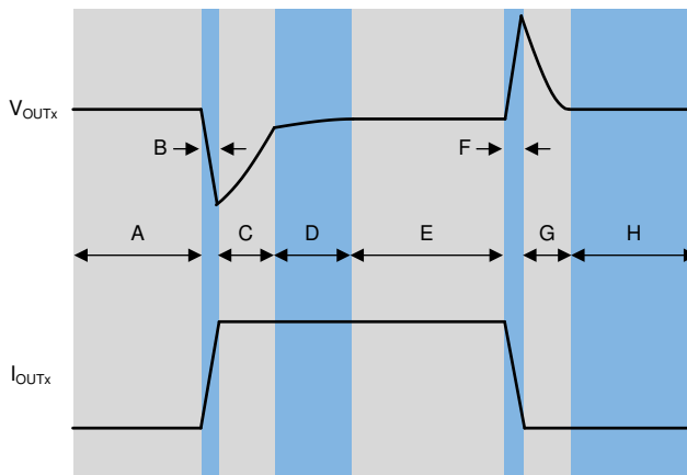
Figure 103. Load Transient Waveform
