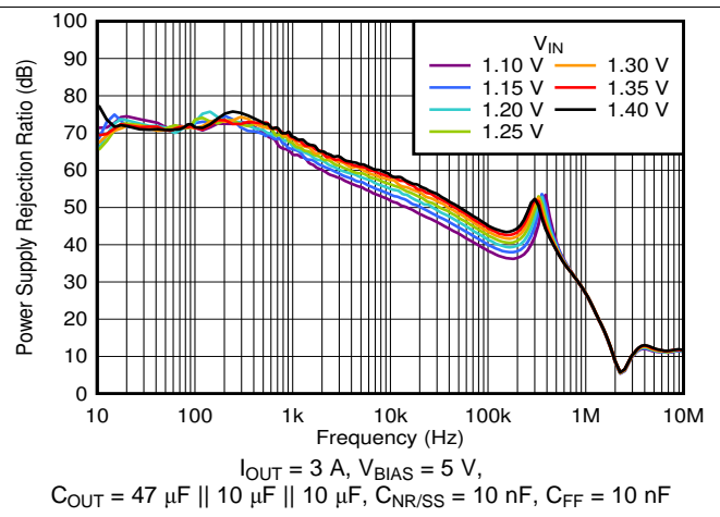
Figure 44. PSRR vs Frequency and V_{IN} With Bias
