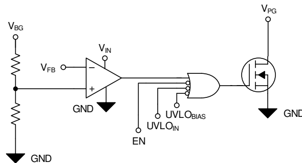
Figure 94. Simplified PG Circuit
