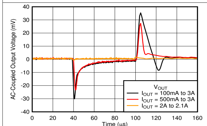
Figure 63. Load Transient vs Time and V_{OUT} Without Bias
