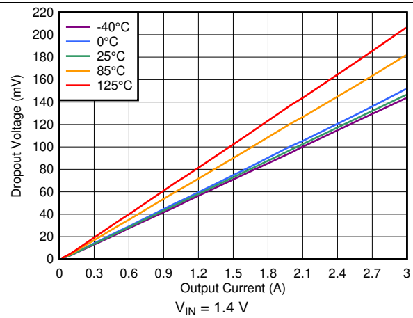
Figure 22. Dropout Voltage vs I_{OUT} Without Bias
