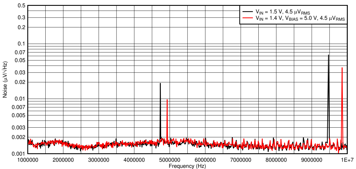
Figure 102. Charge Pump Noise
