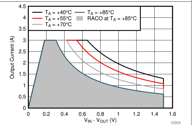
Figure 112. Recommended Area for Continuous Operation for V_{OUT} = 2.5\text{ V}
