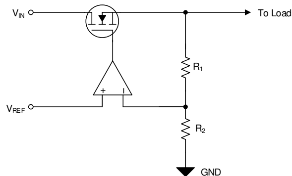
Figure 91. Simplified Regulation Circuit
