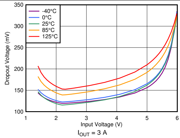
Figure 20. Dropout Voltage vs V_{IN} Without Bias
