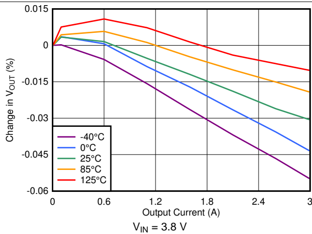
Figure 27. Load Regulation vs I_{OUT} (3.3-V Output)
