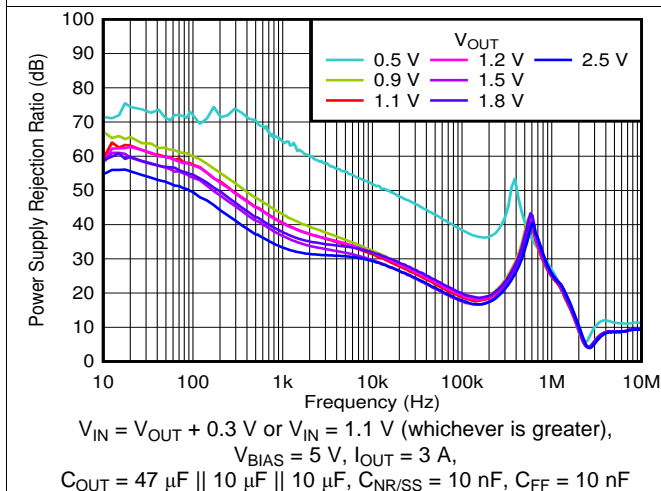
Figure 47. PSRR vs Frequency and V_{OUT} With Bias
