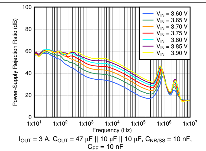
Figure 6. PSRR vs Frequency and V_{IN} ( V_{OUT} = 3.3\text{ V} )
