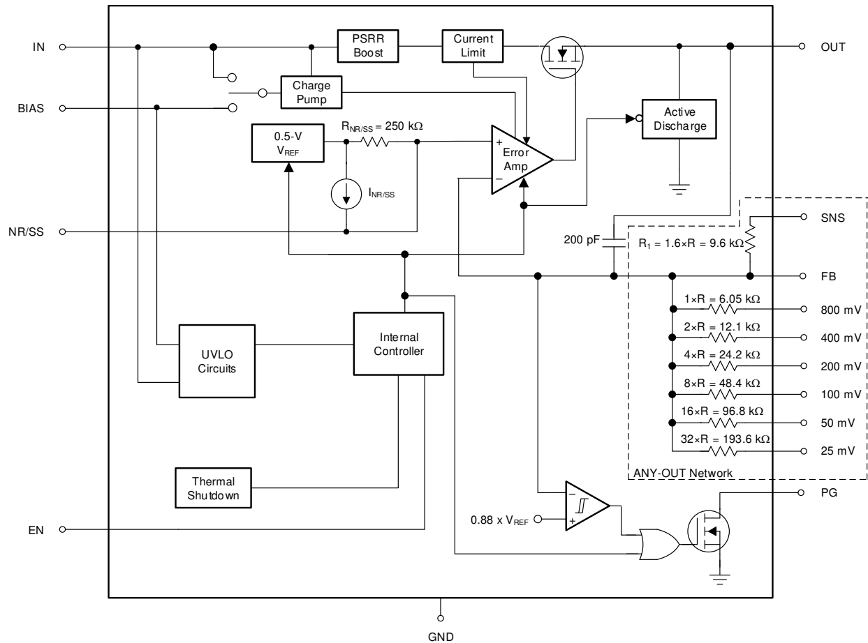
Figure 90. TPS7A8401A Block Diagram
