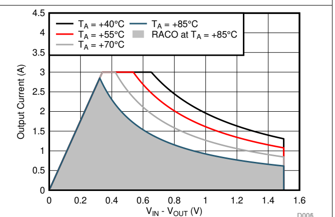
Figure 114. Recommended Area for Continuous Operation for V_{OUT} = 5\text{ V}
