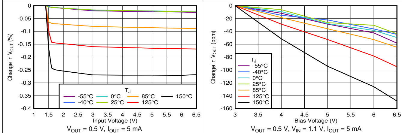
Figure 75. Line Regulation vs V_{IN}
