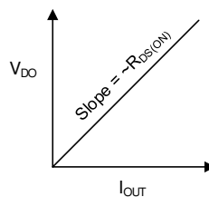
Figure 105. Dropout Voltage versus Output Current
