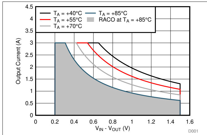
Figure 109. Recommended Area for Continuous Operation for V_{OUT} = 0.9\text{ V}
