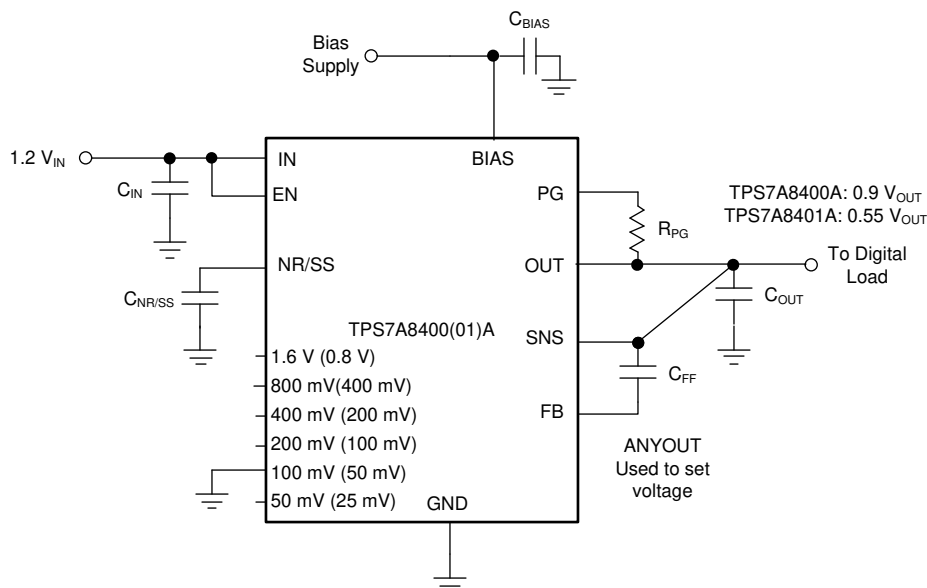
Figure 97. ANY-OUT Configuration Circuit (0.9-V, 0.55-V Output with Bias)
