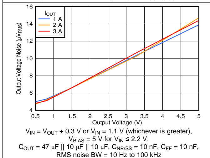
Figure 53. Output Voltage Noise vs V_{OUT}
