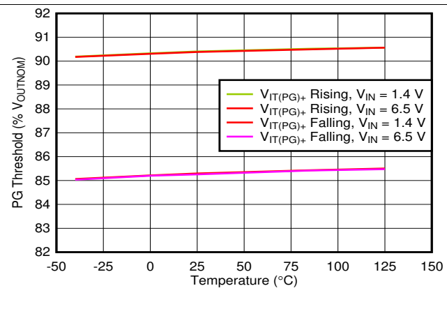
Figure 88. PG Threshold vs Temperature
