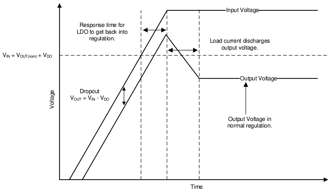
Figure 106. Start-Up Into Dropout
