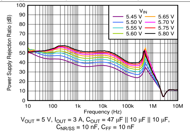
Figure 50. PSRR vs Frequency and V_{IN} ( V_{OUT} = 5\text{ V} )
