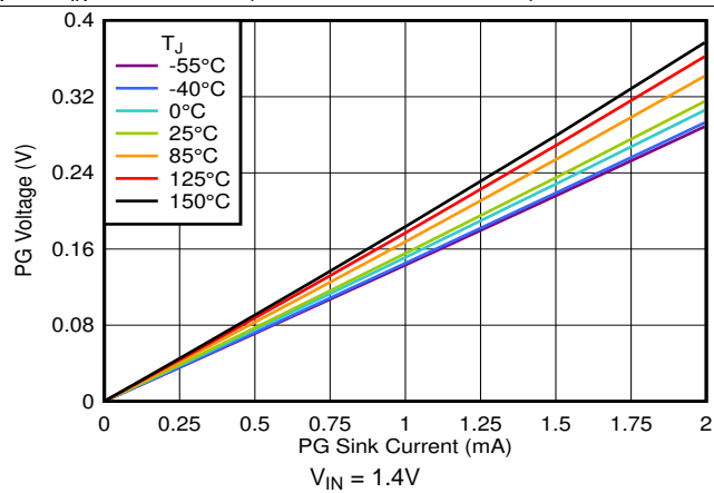
Figure 86. PG Voltage vs PG Current Sink
