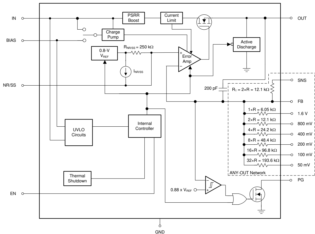
Figure 89. TPS7A8400A Block Diagram
