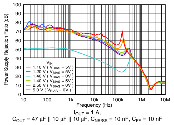
Figure 46. PSRR vs Frequency and V_{IN}
