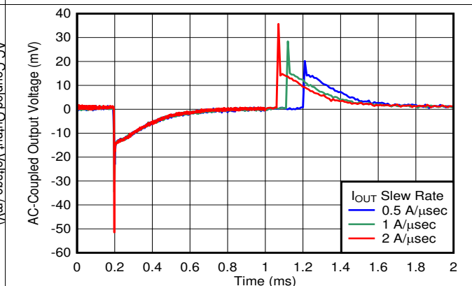
Figure 62. Load Transient vs Time and V_{OUT} Without Bias
