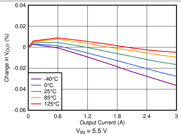
Figure 28. Load Regulation vs I_{OUT} (5-V Output)
