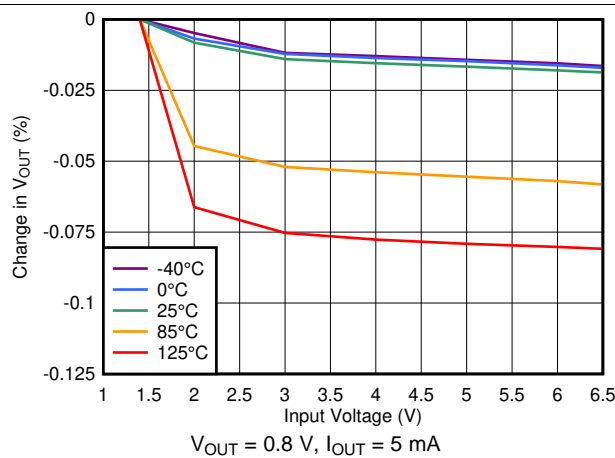
Figure 29. Line Regulation vs V_{IN}
