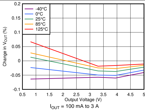
Figure 25. Load Regulation vs V_{OUT}
