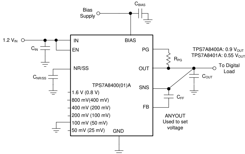
Figure 115. TPS7A84A Typical Application
