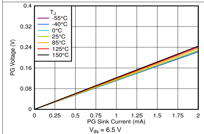
Figure 87. PG Voltage vs PG Current Sink
