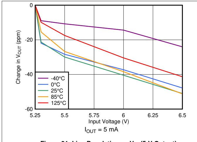
Figure 31. Line Regulation vs V_{IN} (5-V Output)
