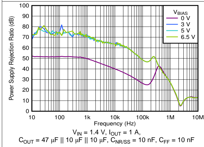
Figure 45. PSRR vs Frequency and V_{BIAS}
