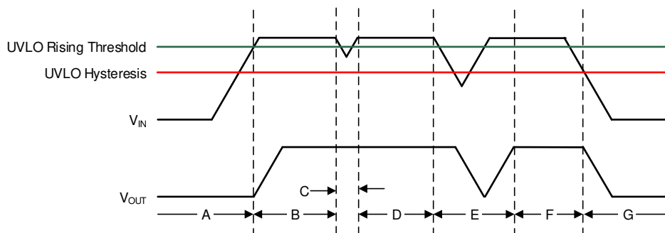
Figure 98. Typical UVLO Operation
