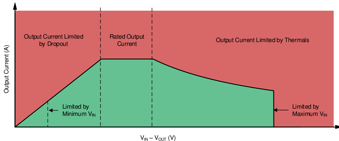
Figure 108. Continuous Operation Slope Region Description
