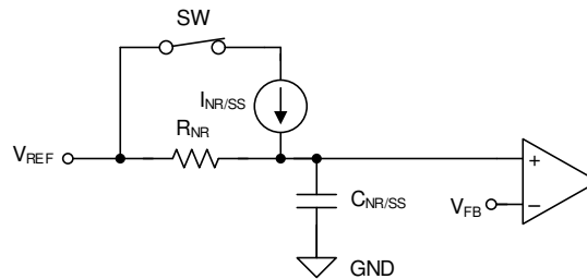
Figure 92. Simplified Soft-Start Circuit
