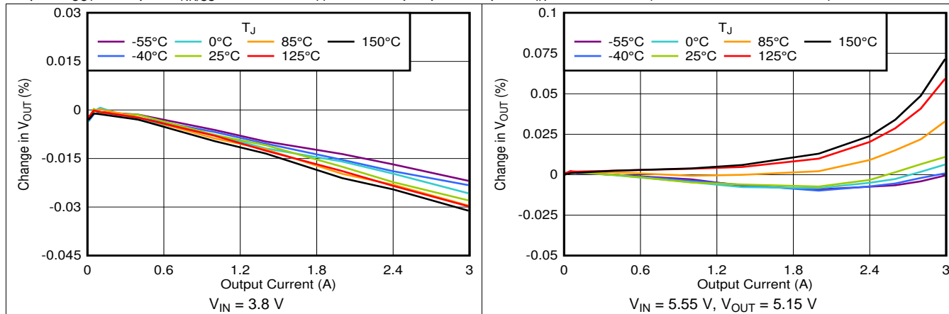
Figure 73. Load Regulation vs I_{OUT} (3.3-V Output)
