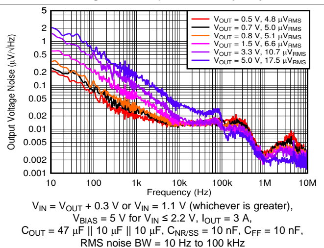
Figure 54. Output Noise vs Frequency and V_{OUT}
