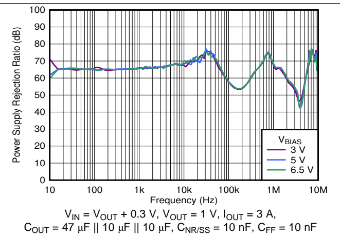
Figure 52. V_{BIAS} PSRR vs Frequency
