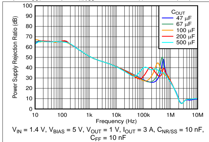
Figure 49. PSRR vs Frequency and C_{OUT}
