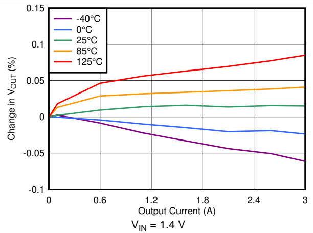
Figure 26. Load Regulation vs I_{OUT}
