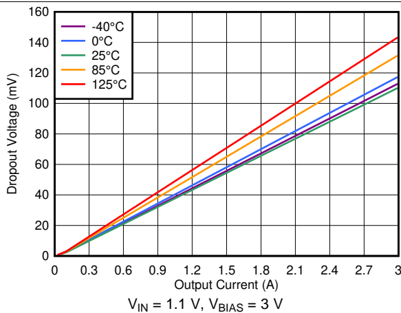
Figure 23. Dropout Voltage vs I_{OUT} With Bias
