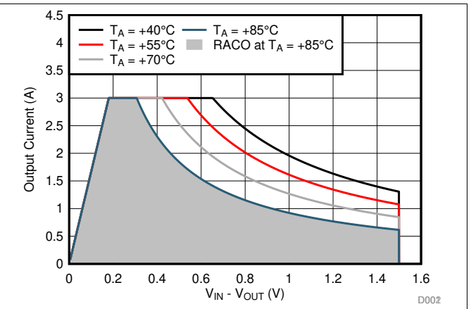
Figure 110. Recommended Area for Continuous Operation for V_{OUT} = 1.2\text{ V}
