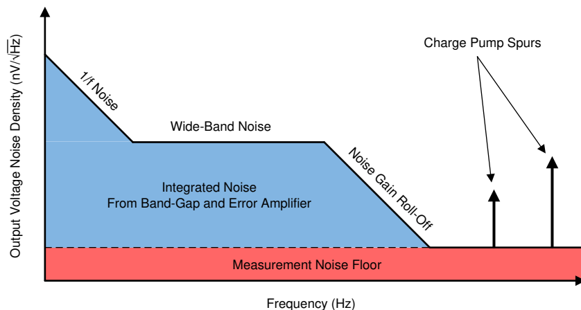
Figure 101. Output Voltage Noise Diagram
