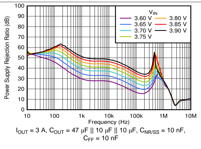
Figure 48. PSRR vs Frequency and V_{IN} ( V_{OUT} = 3.3\text{ V} )
