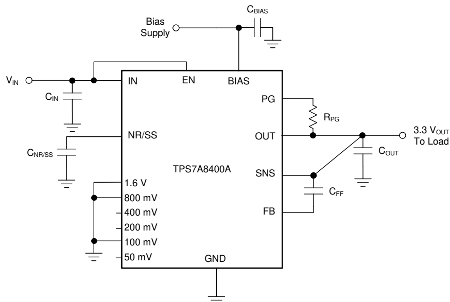
Figure 96. ANY-OUT Configuration Circuit (TPS7A8400A) (3.3-V Output, No External Bias)
