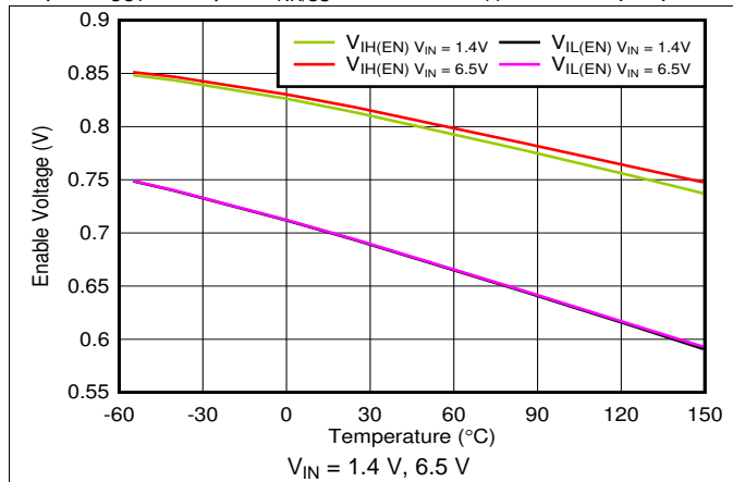
Figure 85. Enable Threshold vs Temperature
