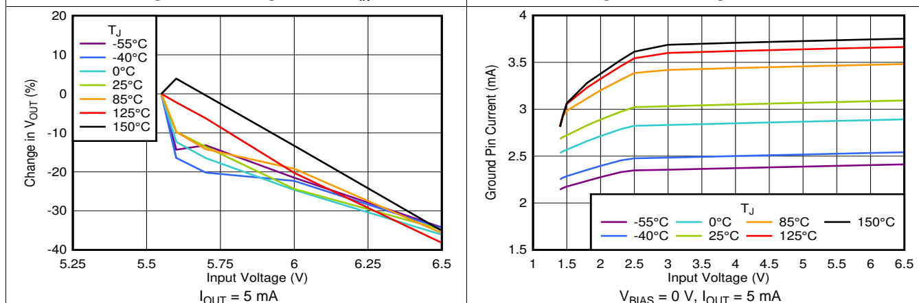
Figure 77. Line Regulation vs V_{IN} (5.15-V Output)
