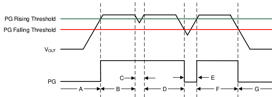
Figure 99. Typical PG Operation
