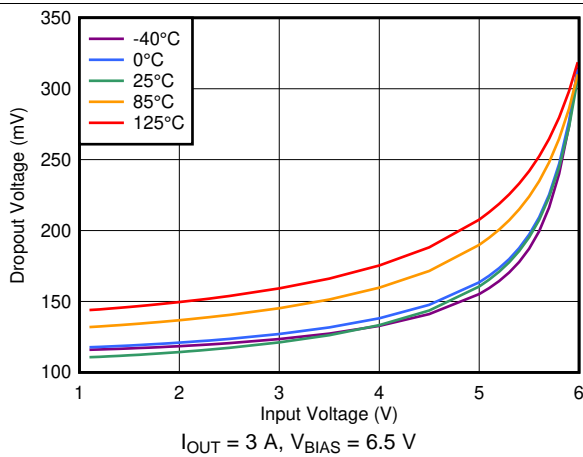
Figure 21. Dropout Voltage vs V_{IN} With Bias
