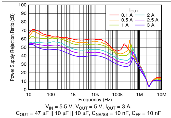
Figure 51. PSRR vs Frequency and I_{OUT} ( V_{OUT} = 5\text{ V} )
