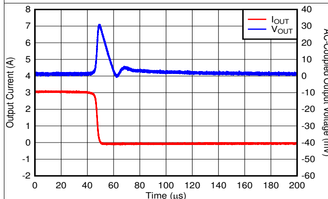
Figure 61. Load Transient vs Time and V_{OUT} With Bias
