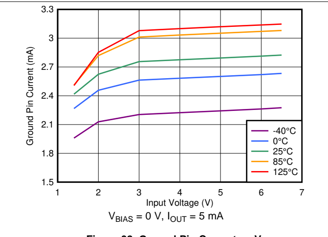
Figure 32. Ground Pin Current vs V_{IN}
