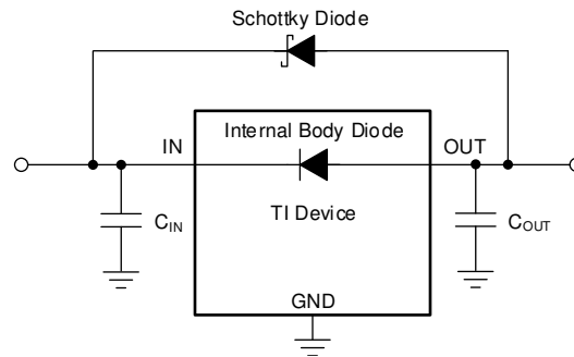
Figure 107. Example Circuit for Reverse Current Protection Using a Schottky Diode
