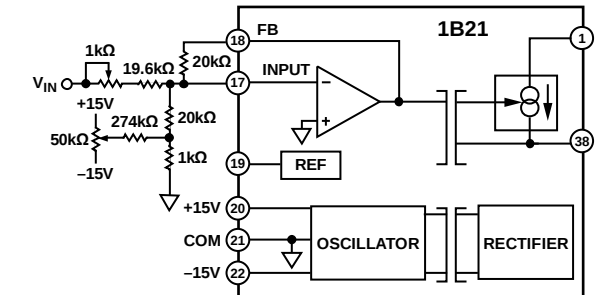
Figure 5. Offset and Span Adjustment
