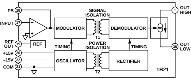
Figure 3. 1B21 Functional Block Diagram
