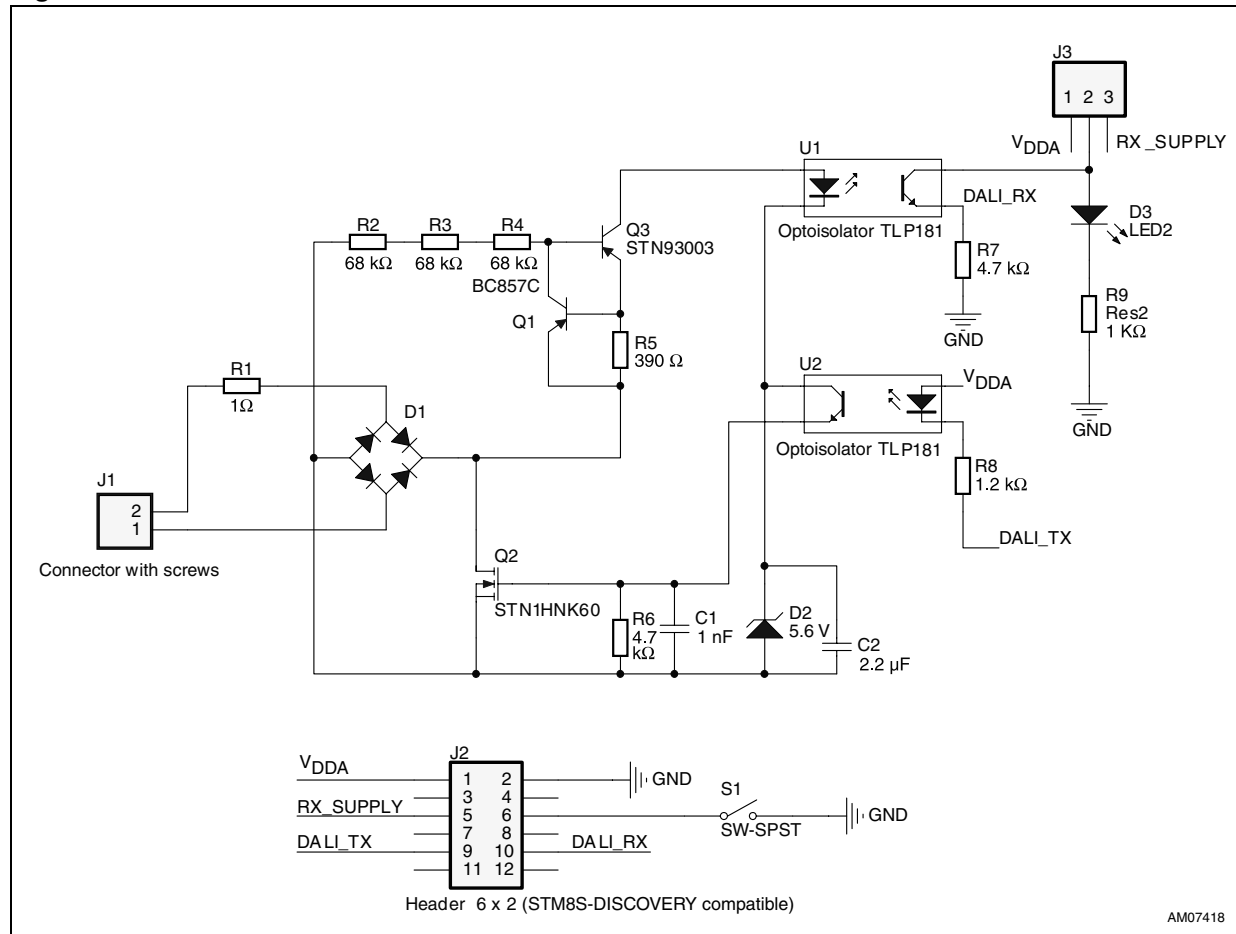
Figure 1. Circuit schematic
