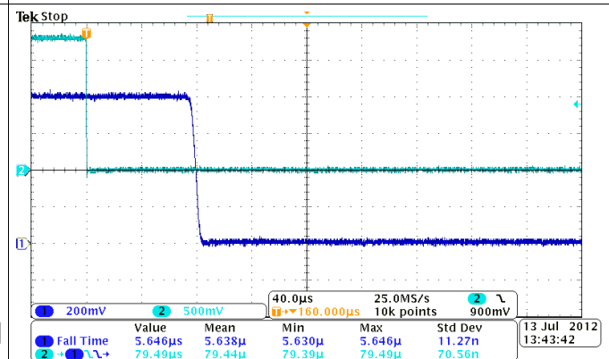
Figure 28. Turnoff Response Time (V_{IN} = 0.8\text{ V}, V_{BIAS} = 5\text{ V}, C_{IN} = 1\text{ }\mu\text{F}, C_L = 0.1\text{ }\mu\text{F}, R_L = 10\text{ }\Omega) CH1: VOUT, CH2: ON
