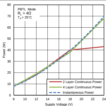
Figure 33. Output Power vs Supply Voltage (PBTL Mode)
