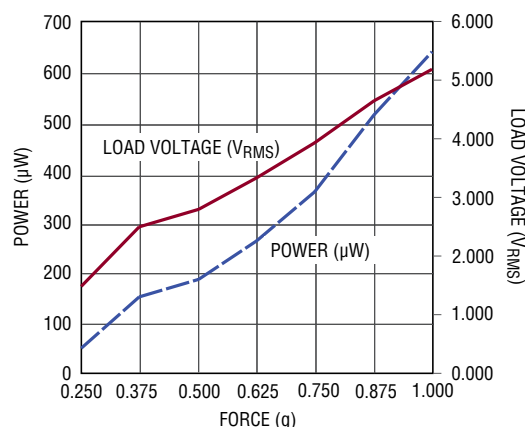
Figure 7. MIDE V25W Output Power into a 42.2kΩ Load with 1grms, 60Hz Acceleration Applied the MIDE V25W Piezoelectric Transducer, [\sqrt{2} \cdot \sin(2\pi \cdot 60\text{Hz} \cdot t)]
