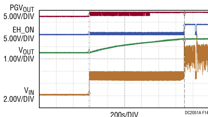
Figure 14. MIDE 25W Charging Output Supercapacitor from 2.5V to 3.6 V with DUST Mote Attached
