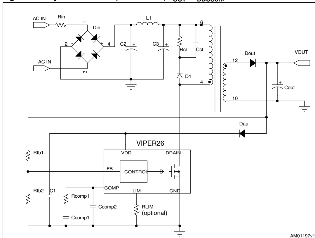
Figure 21. Flyback converter (non isolated, V_{OUT} \approx V_{DDCSon} )
