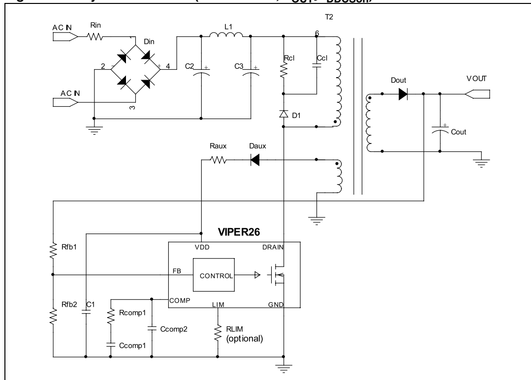
Figure 21. Flyback converter (non isolated, V_{OUT} \approx V_{DDCSon} )
