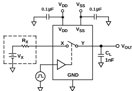
Figure 29. Charge Injection
