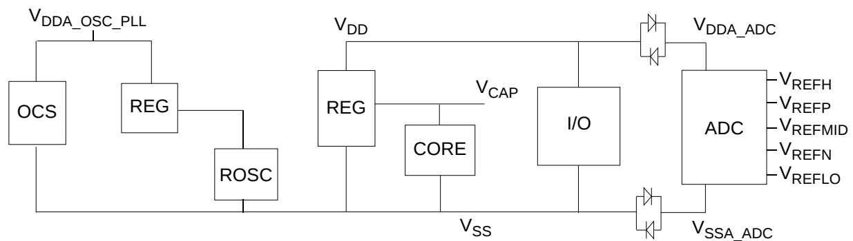
Figure 12-1 Power Management
