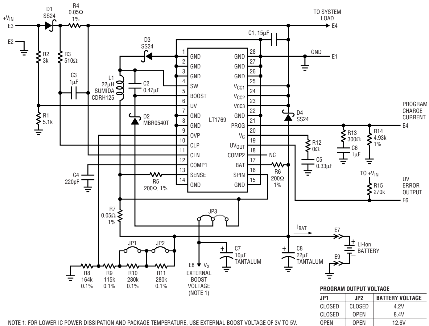
Figure 1. Constant-Voltage/Constant-Current Lithium-Ion Battery Charger with Input Current Limiting
