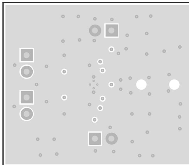
Figure 5. TPA6120A2RGY EVM Bottom Layer
