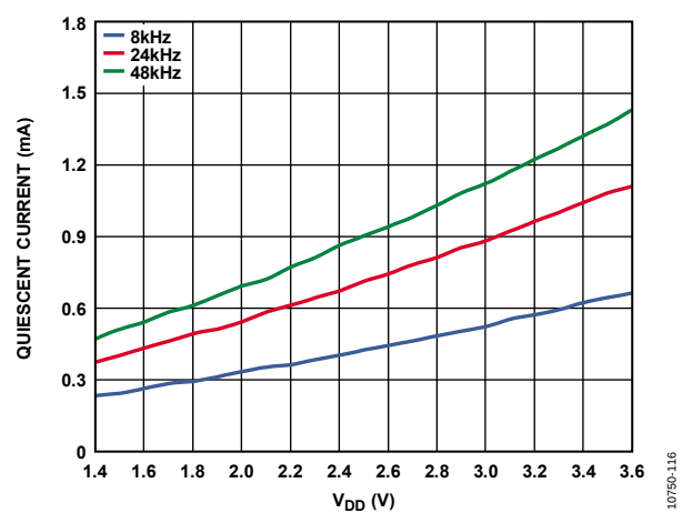
Figure 16. Quiescent Current vs. Supply Voltage V_{DD}
