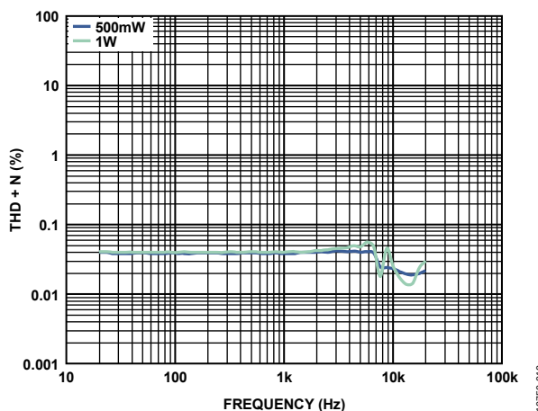
Figure 10. THD + N vs. Frequency into 4 \Omega , PV_{DD} = 5.0 V
