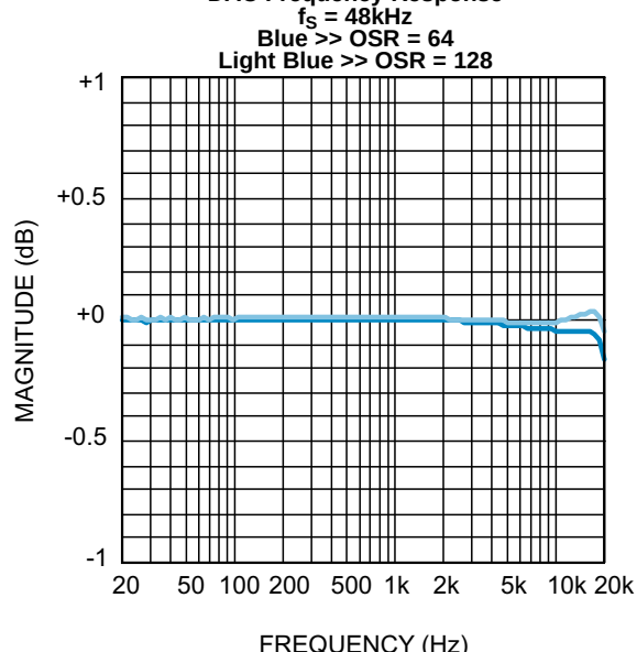
DAC Frequency Response
