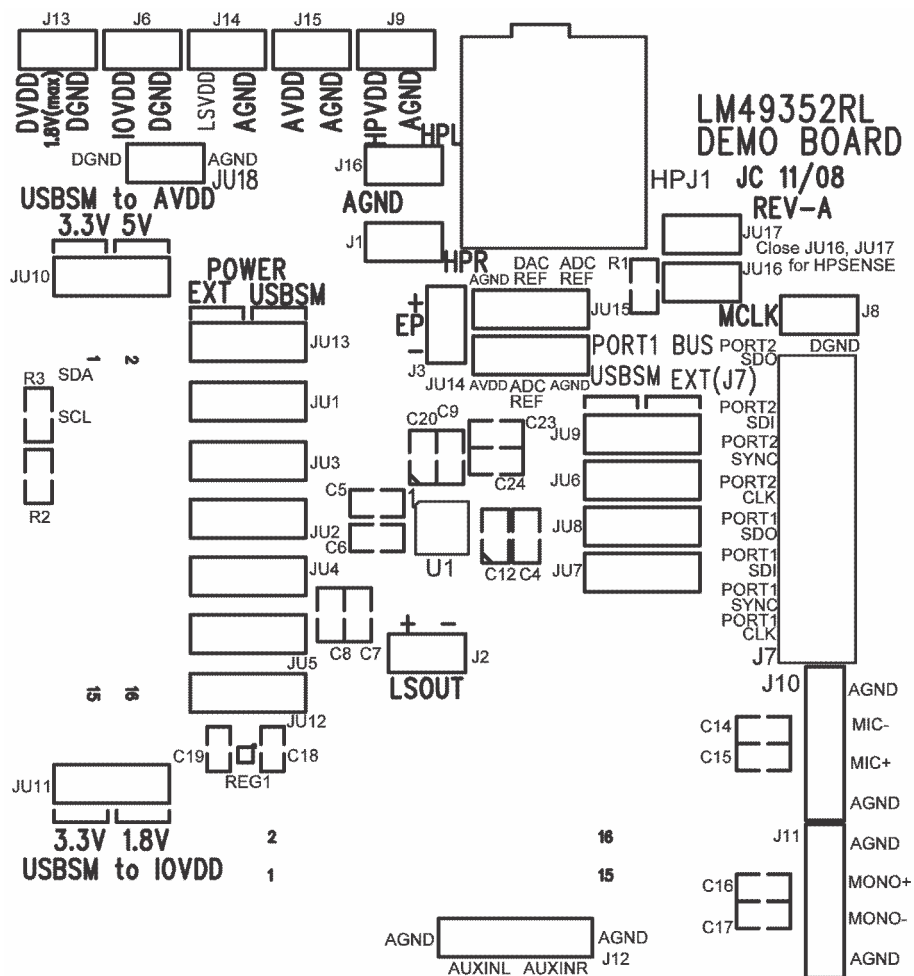
Figure 73. Top Silkscreen
