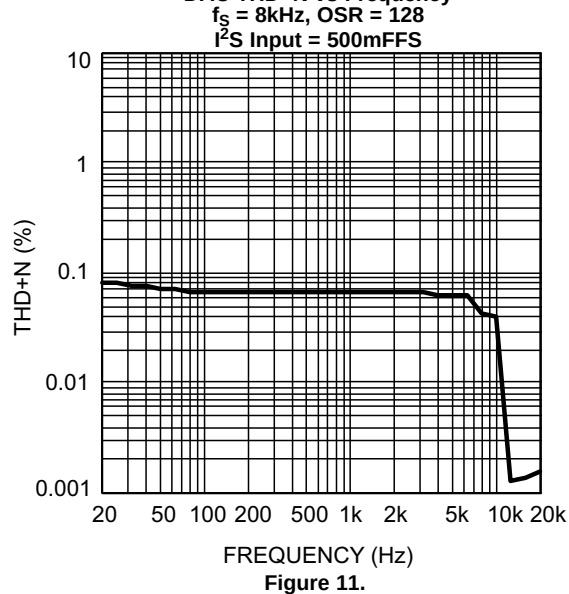
DAC THD+N vs Frequency
