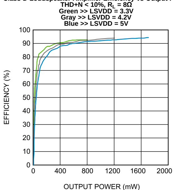
Class D Loudspeaker Amplifier Efficiency vs Output Power
