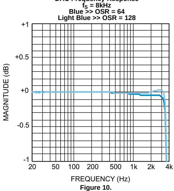
DAC Frequency Response
