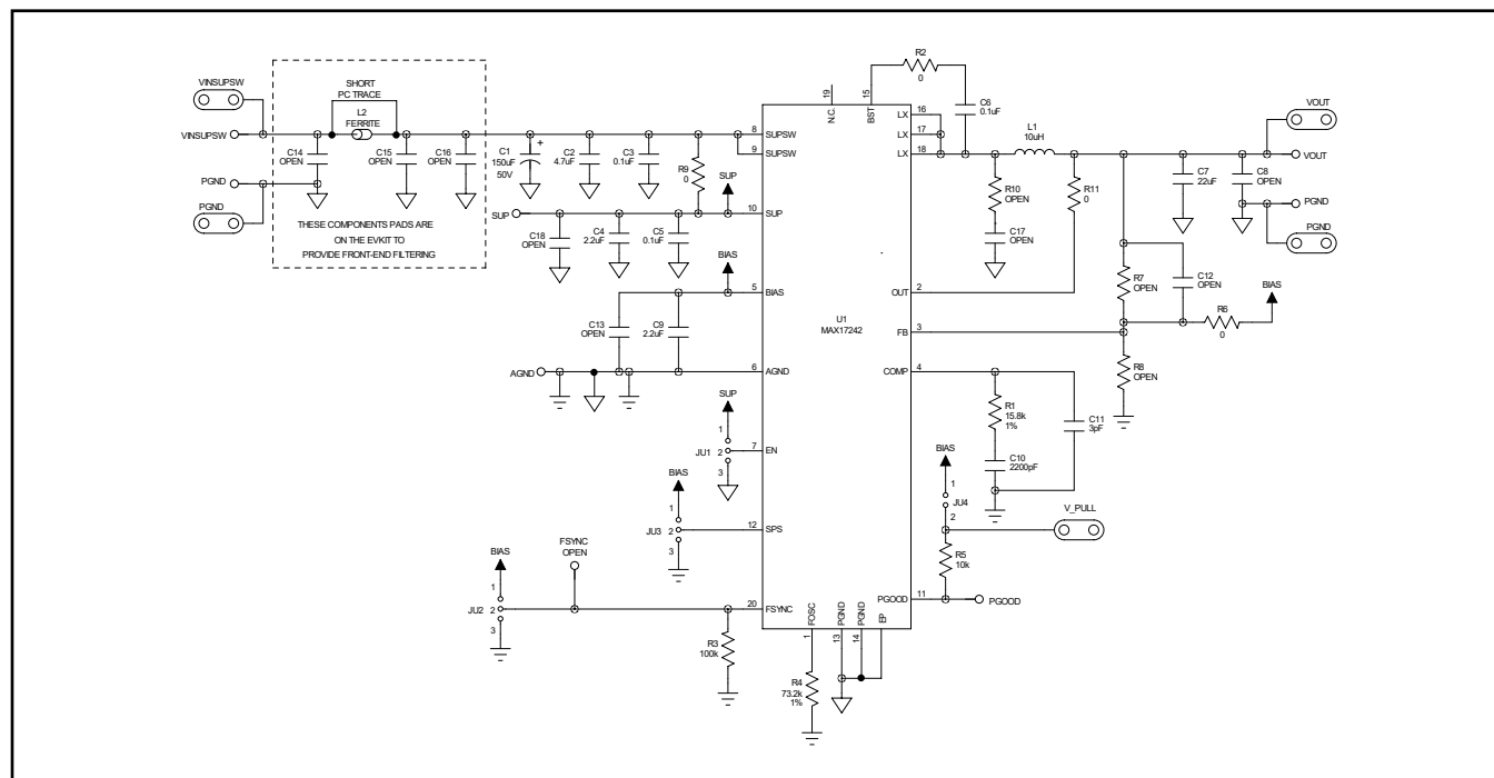
MAX17242 EV Schematic
