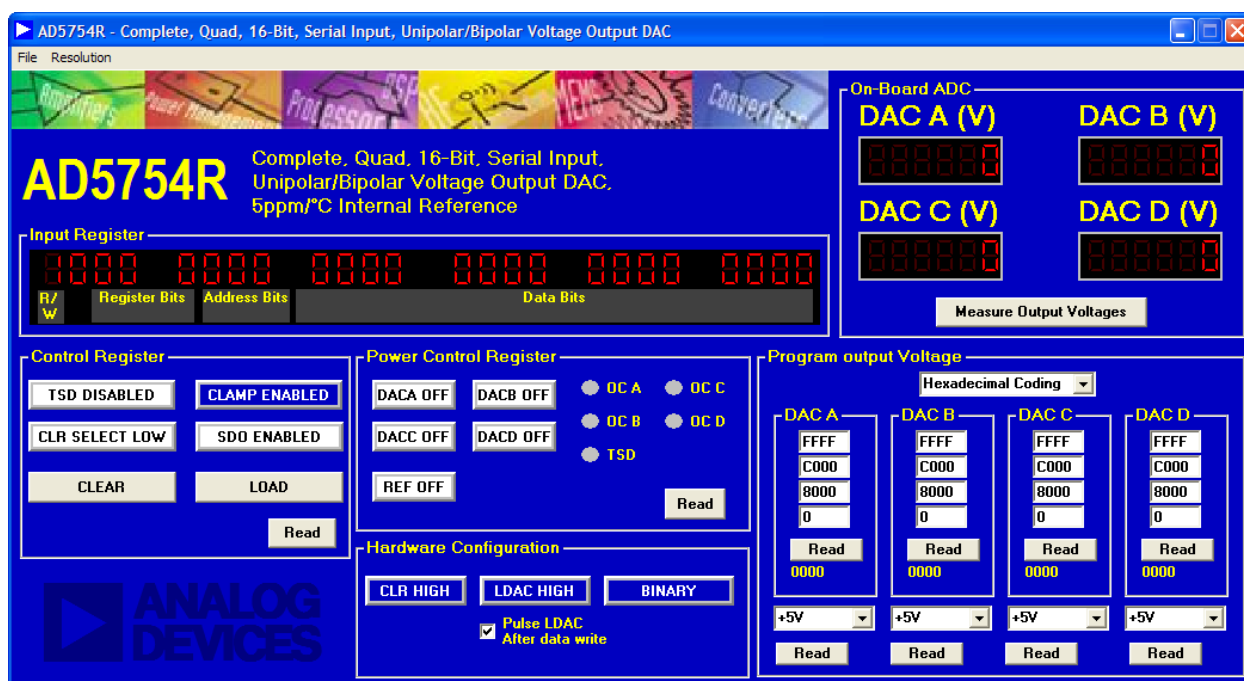
Figure 2. Main Window
