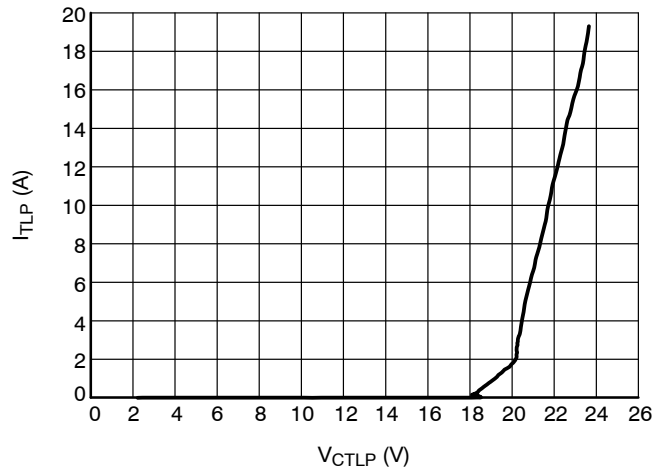
Figure 4. Pin 2 to Pin 1 TLP I-V Curve
