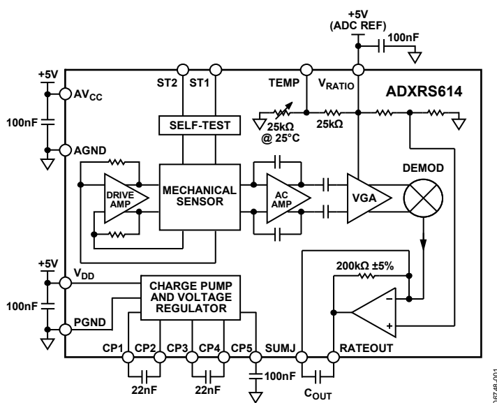
Figure 1. ADXRS614 Block Diagram
