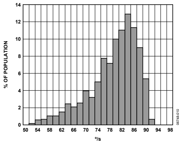
Figure 10. Measurement Range
