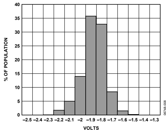
Figure 8. ST1 Output Change at 25°C ( V_{RATIO} = 5\text{ V} )
