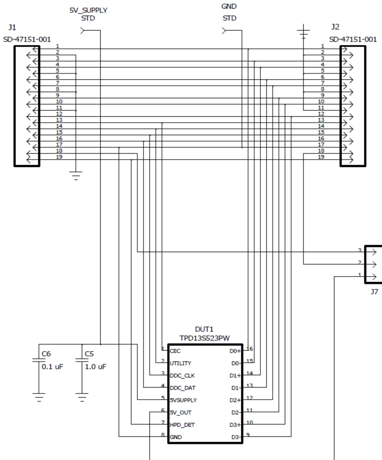
Figure 1. Schematic Drawing
