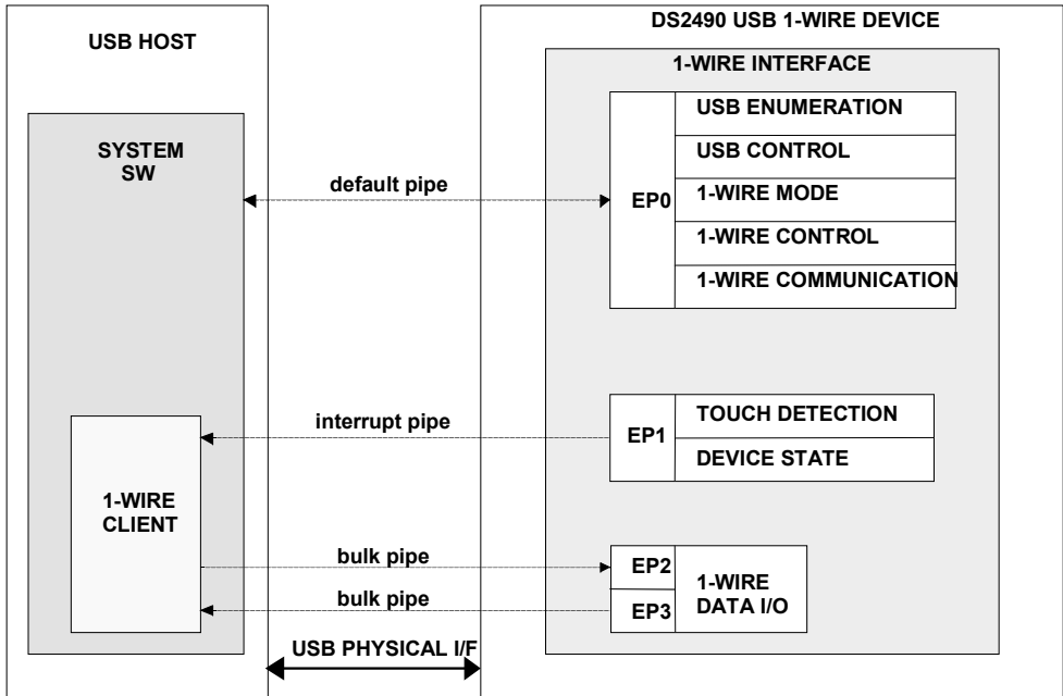
USB CONFIGURATION Figure 9
