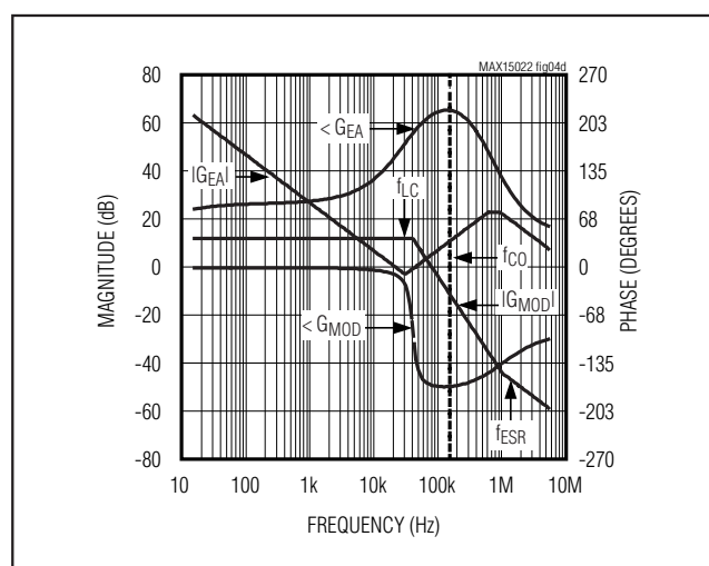
Figure 4d. Power Modulator and Type III Compensator Gain and Phase Response with Low Parasitic Capacitors (MLCCs)
