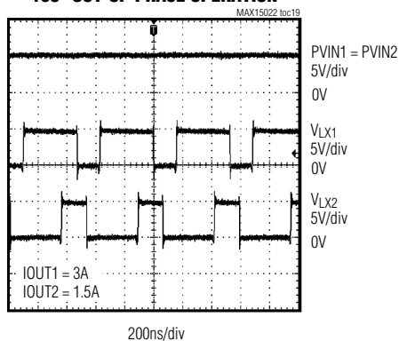
180° OUT-OF-PHASE OPERATION
