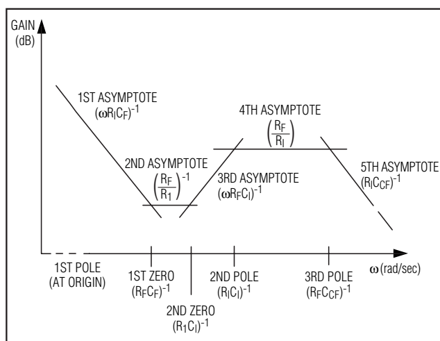
Figure 6b. Type III Compensation Network Response
