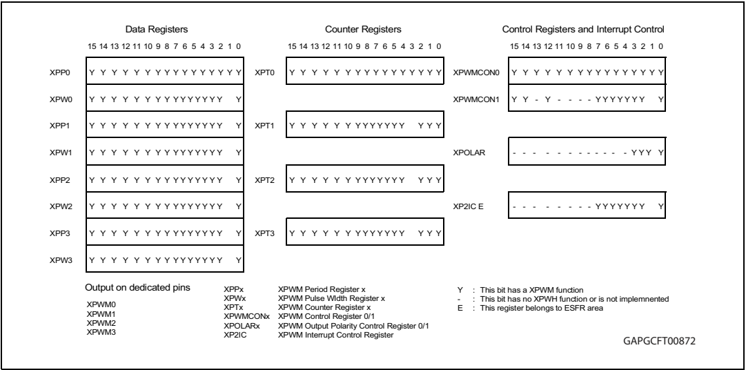
Figure 18. SFRs and port pins associated with the XPWM module
