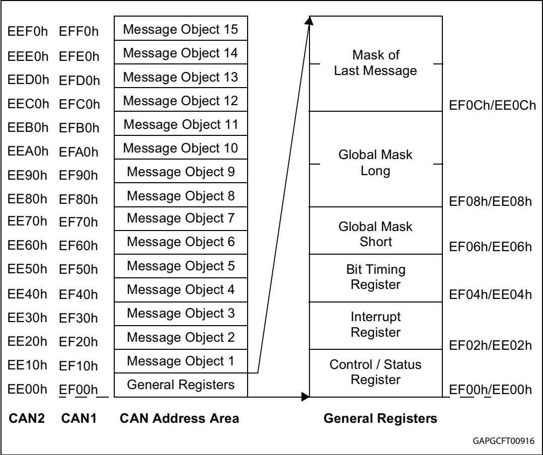
Figure 62. CAN module address map
