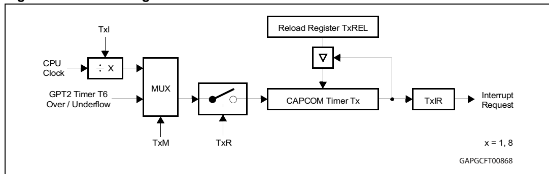
Figure 14. Block diagram of CAPCOM timers T1 and T8
