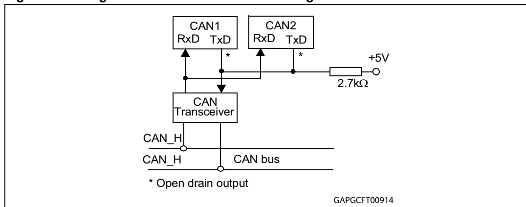
Figure 60. Single CAN bus dual interfaces - single transceiver
