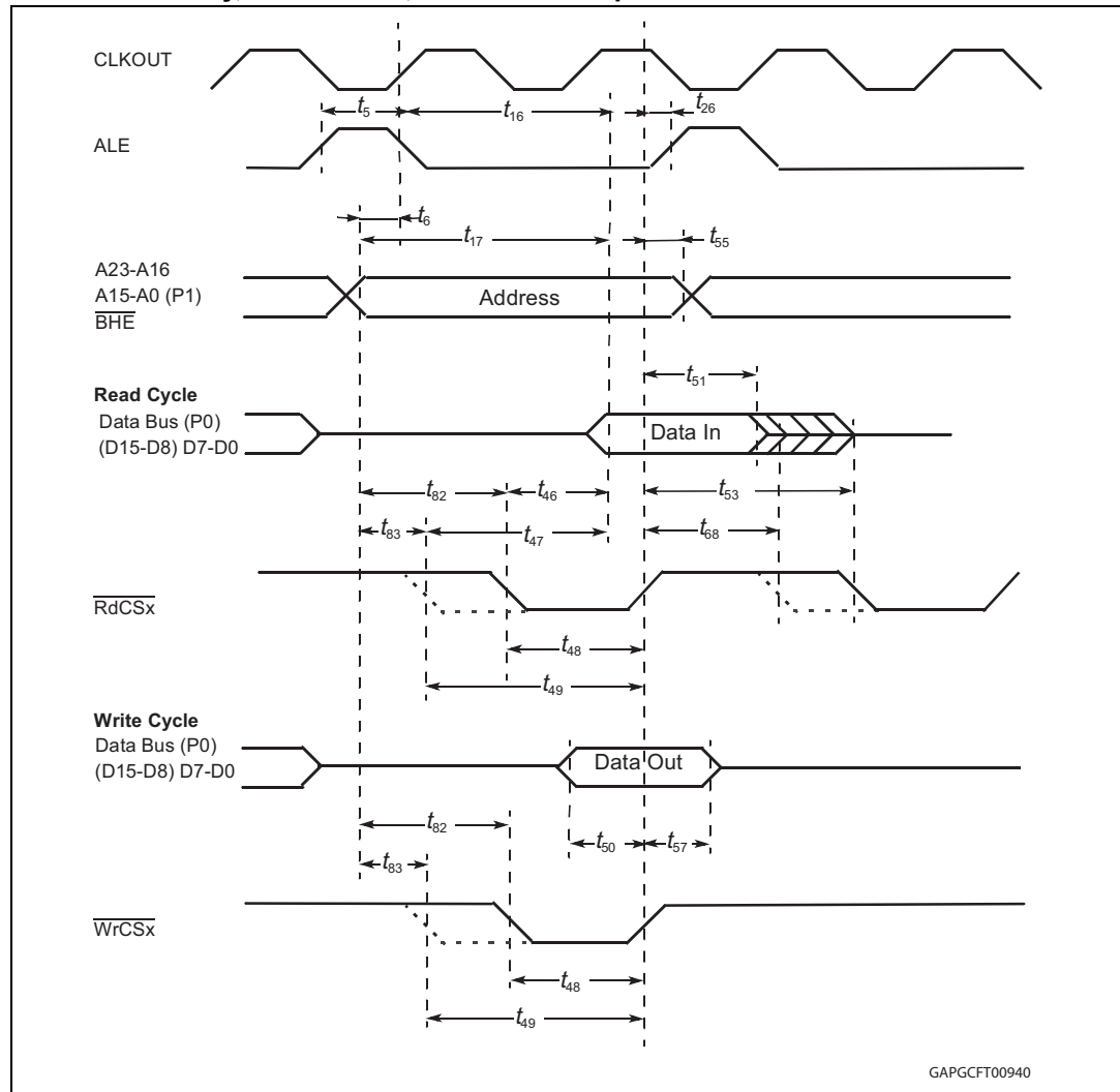
Figure 86. External memory cycle: demultiplexed bus, with / without read / write delay, normal ALE, read / write chip select
