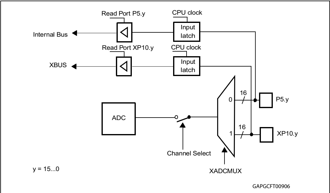
Figure 52. Block diagram
