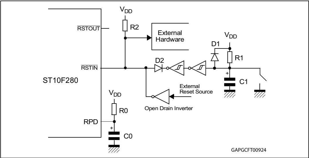
Figure 70. External reset hardware circuitry
