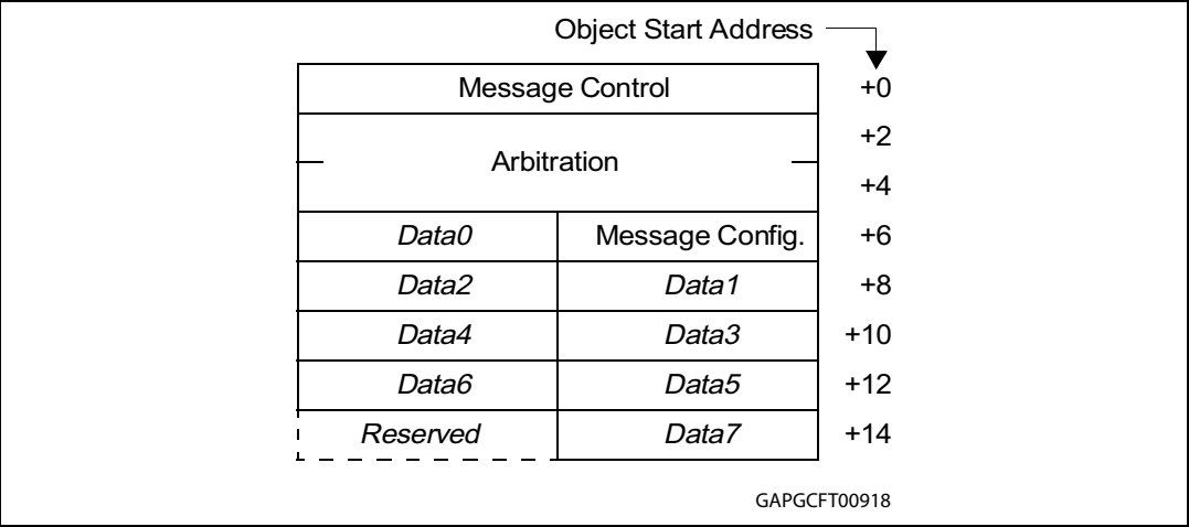
Figure 64. Message object address map
