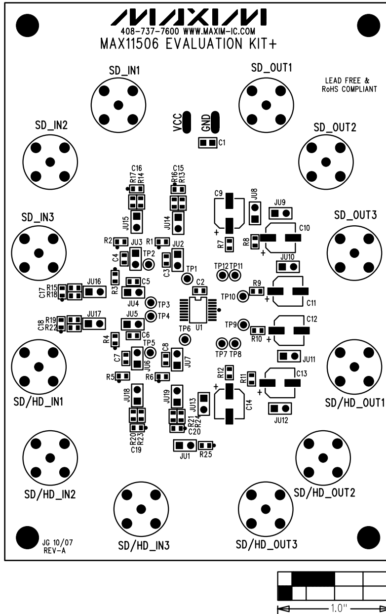
Figure 2. MAX11506 EV Kit Component Placement Guide—Top Silkscreen
