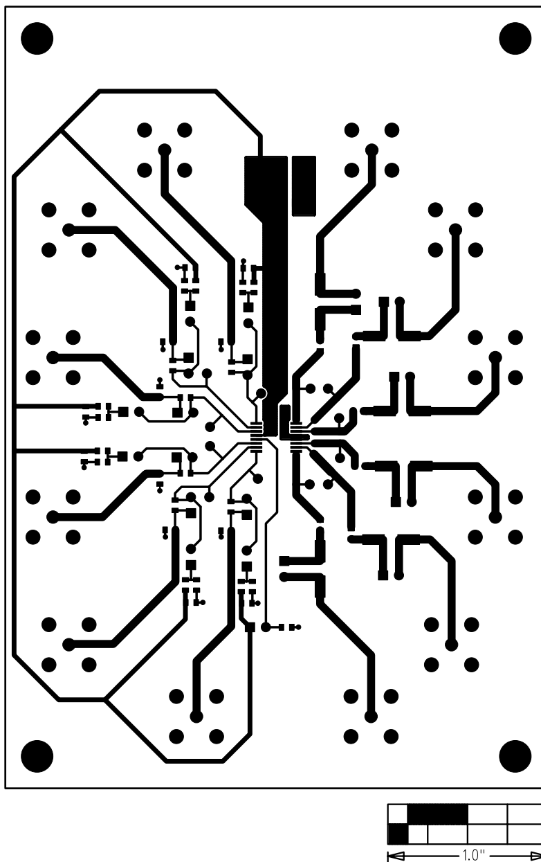
Figure 3. MAX11506 EV Kit PCB Layout—Component Side
