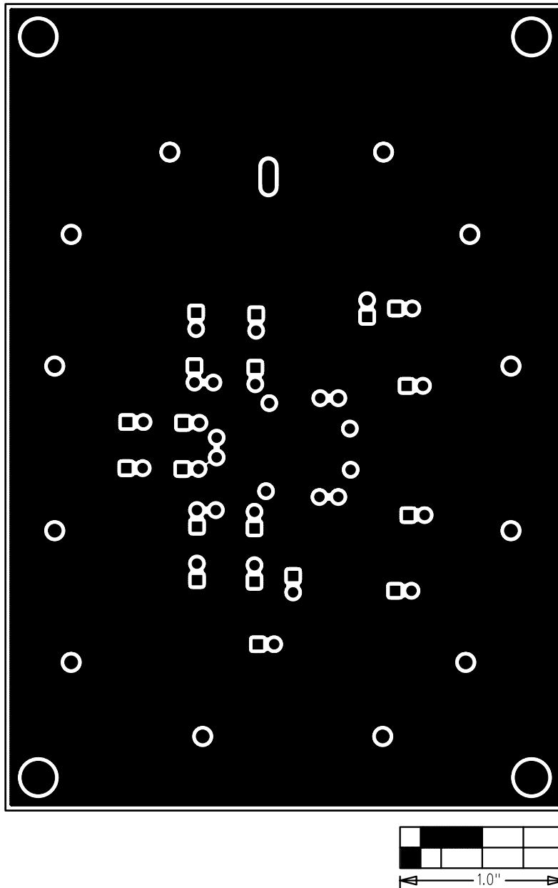
Figure 4. MAX11506 EV Kit PCB Layout—Solder Side
