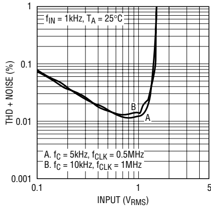
THD + Noise vs Input Voltage; V_S = \text{Single } 5V, AGND = 2V
