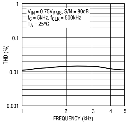
THD vs Frequency; V_S = \text{Single } 5V, AGND = 2V
