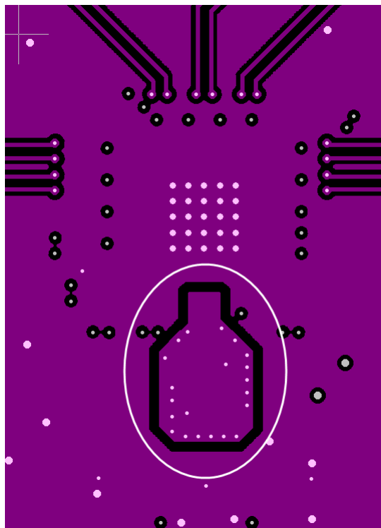
Figure 11.2. 56-lead Si5383/84 Crystal Layout Recommendations 2nd Layer with Ground Shield (Layer 2)
