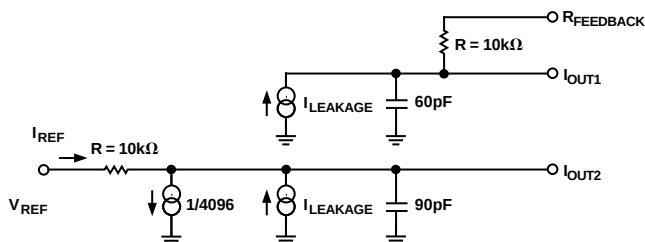
Figure 12. Equivalent Circuit (All Inputs LOW)
