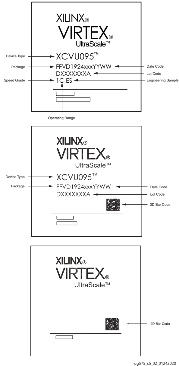
Figure 5-2: Virtex UltraScale Device Package Marking
