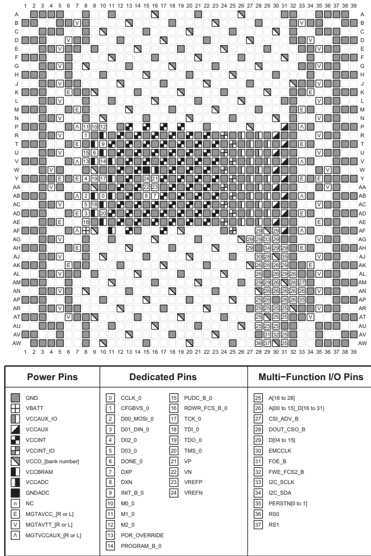
Figure 3-22: FFVC1517 Package—XCKU095 Configuration/Power Diagram
