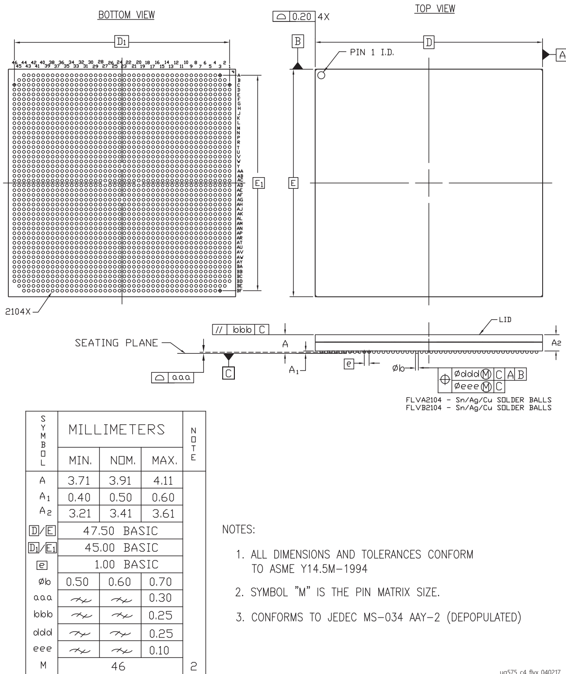
Figure 4-35: Package Dimensions for FLVA2104 (XCVU5P and XCVU7P) and FLVB2104 (XCVU5P and XCVU7P)
