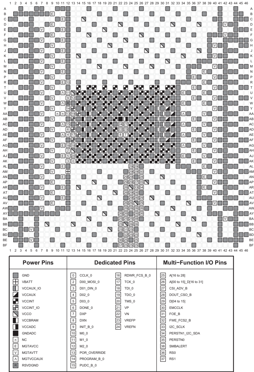
Figure 3-132: FSGD2104 Package—XCVU9P Configuration/Power Diagram
