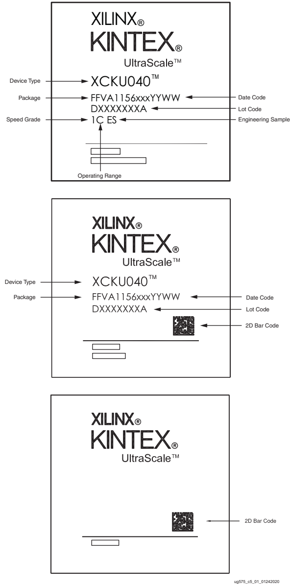
Figure 5-1: Kintex UltraScale Device Package Marking
