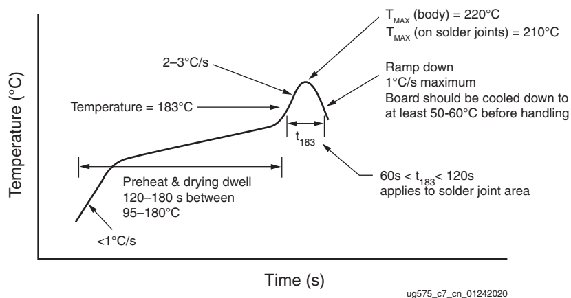
Figure 7-2: CN Package Soldering Guidelines
