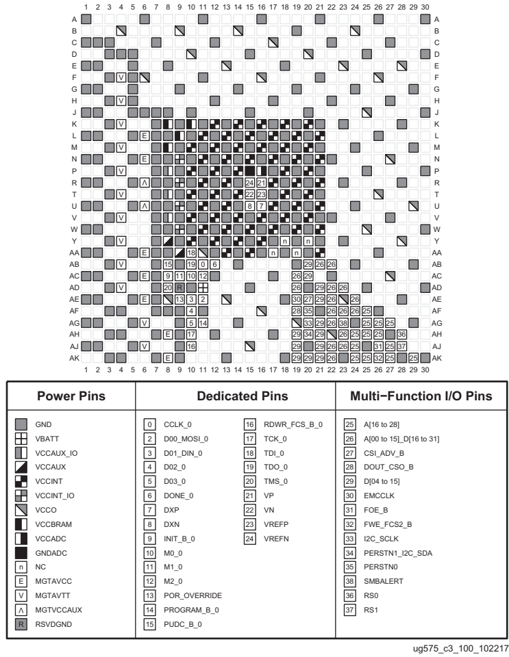
Figure 3-86: FFVD900 Package—XCKU11P Configuration/Power Diagram
