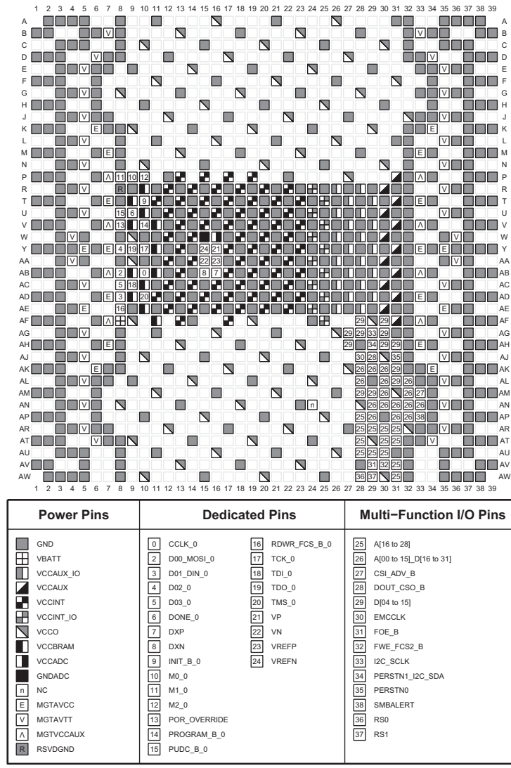
Figure 3-104: FFVC1517 Package—XCVU3P and FFRC1517 Package—XQVU3P Configuration/Power Diagram
