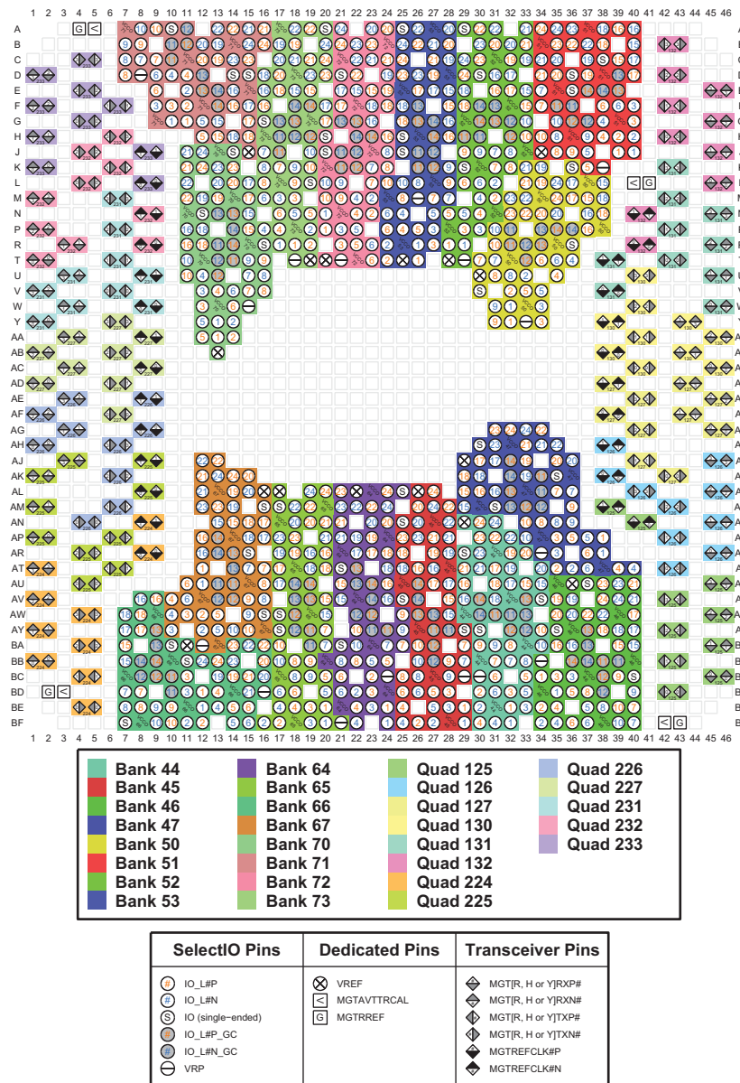
Figure 3-109: FLVA2104 Package—XCVU5P and XCVU7P and FLRA2104 Package—XQVU7P I/O Bank Diagram
