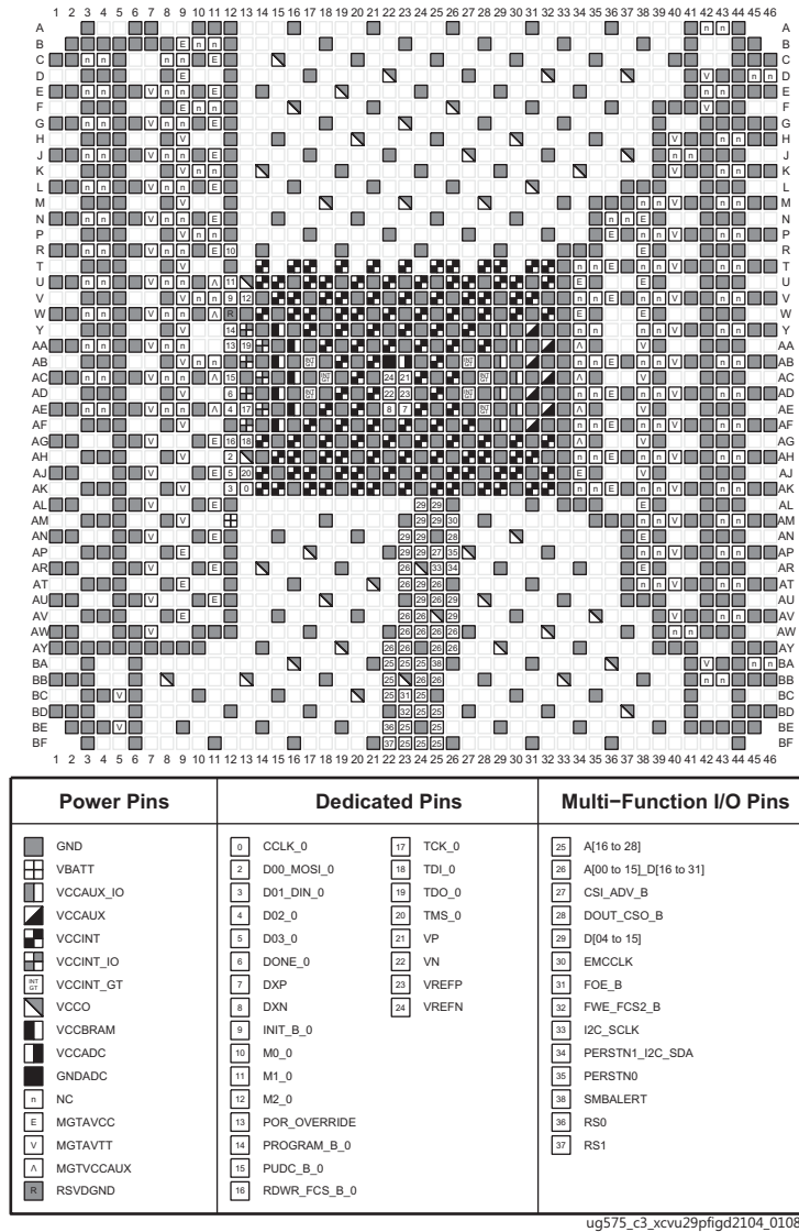
Figure 3-140: FIGD2104 Package—XCVU29P Configuration/Power Diagram
