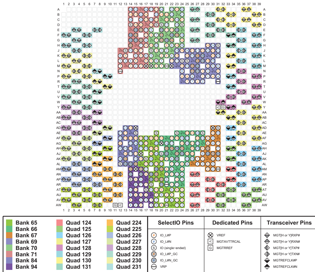
Figure 3-47: FFVD1517 Package—XCVU080 and XCVU095 I/O Bank Diagram
