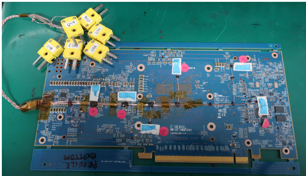
Figure 7-5: Thermocouple Bottom
