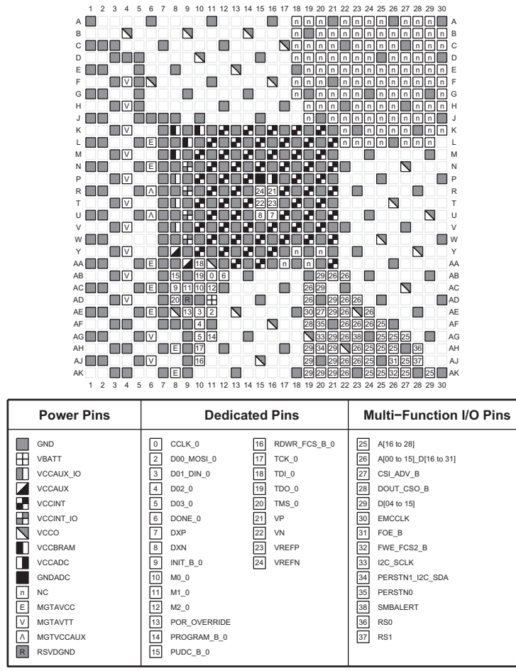
Figure 3-84: FFVD900 Package—XCKU3P and XCKU5P Configuration/Power Diagram
