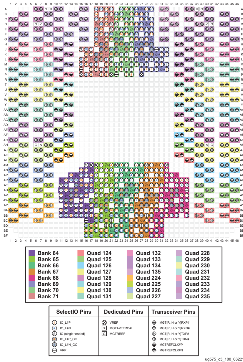
Figure 3-127: FLGC2104 Package—XCVU11P and FLRC2104 Package—XQVU11P I/O Bank Diagram
