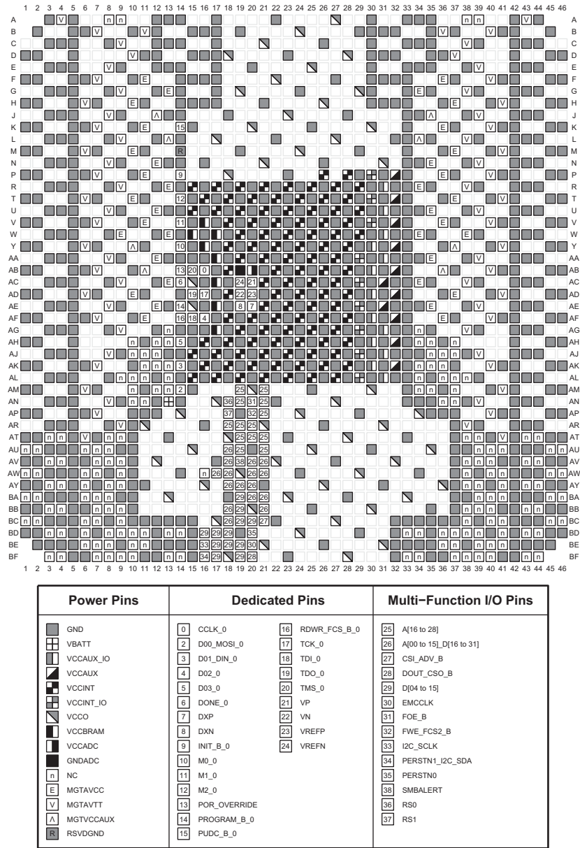
Figure 3-124: FLVC2104 Package—XCVU5P and XCVU7P Configuration/Power Diagram
