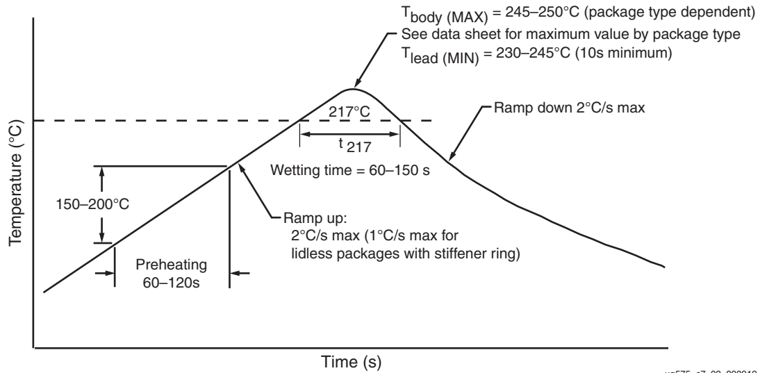
Figure 7-3: Typical Conditions for Pb-Free Reflow Soldering
