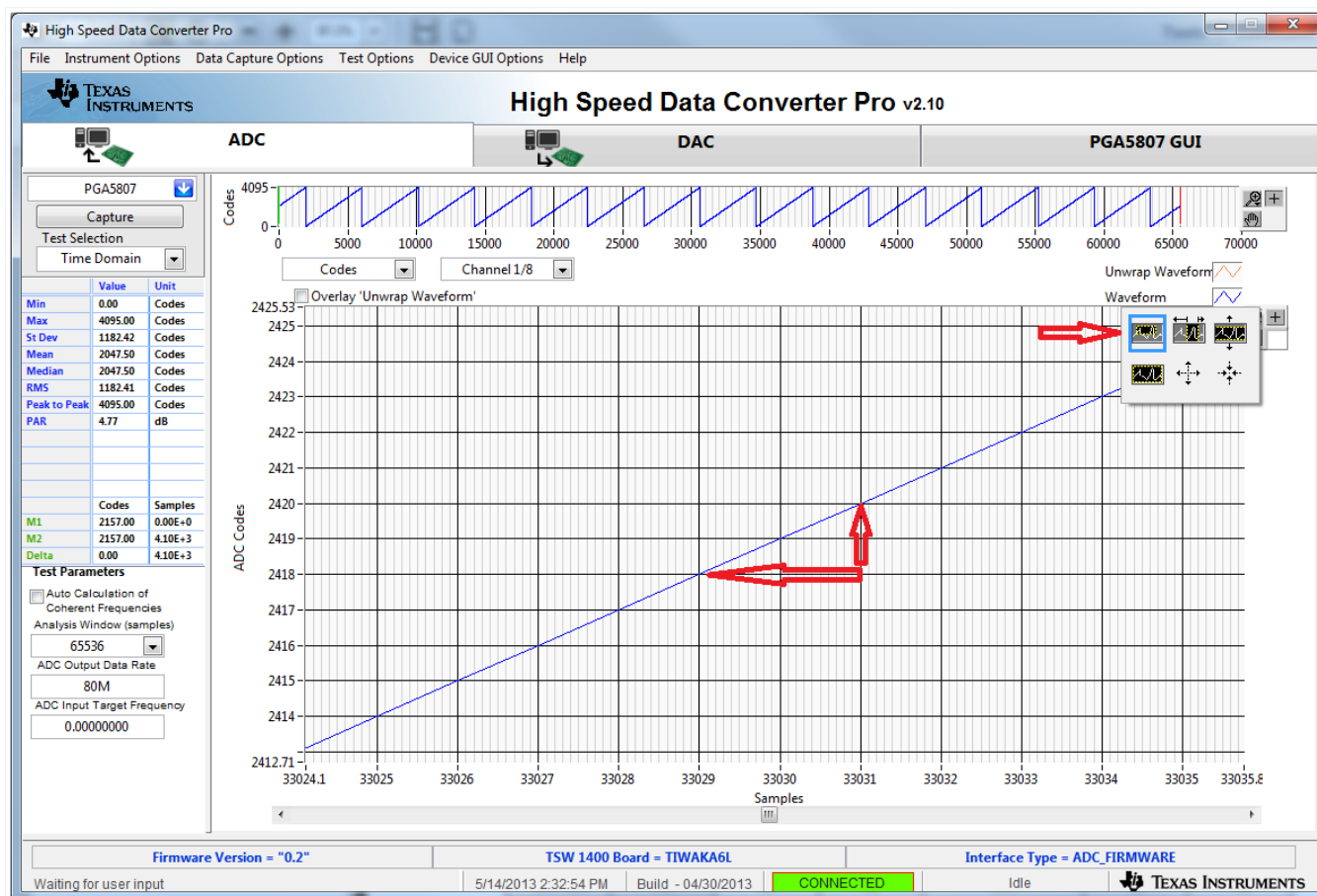
Figure 36. Zoom on RAMP Capture
