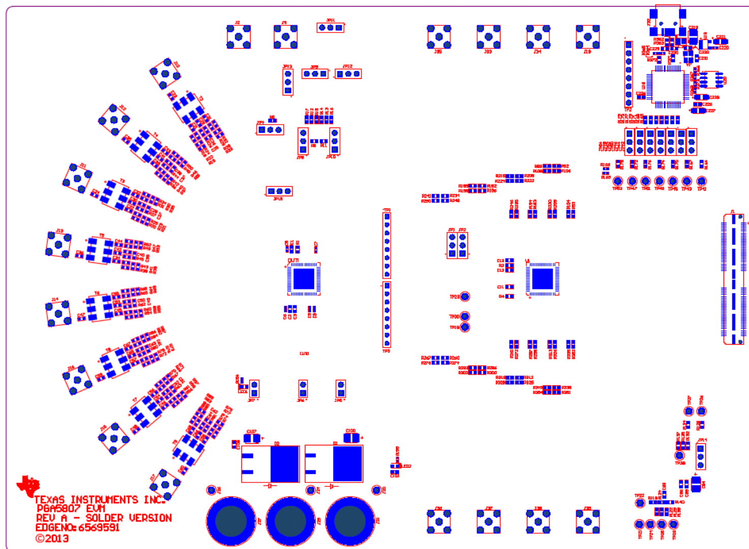
Figure 79. PGA5807 EVM Top Layer Assembly Drawing – Top View
