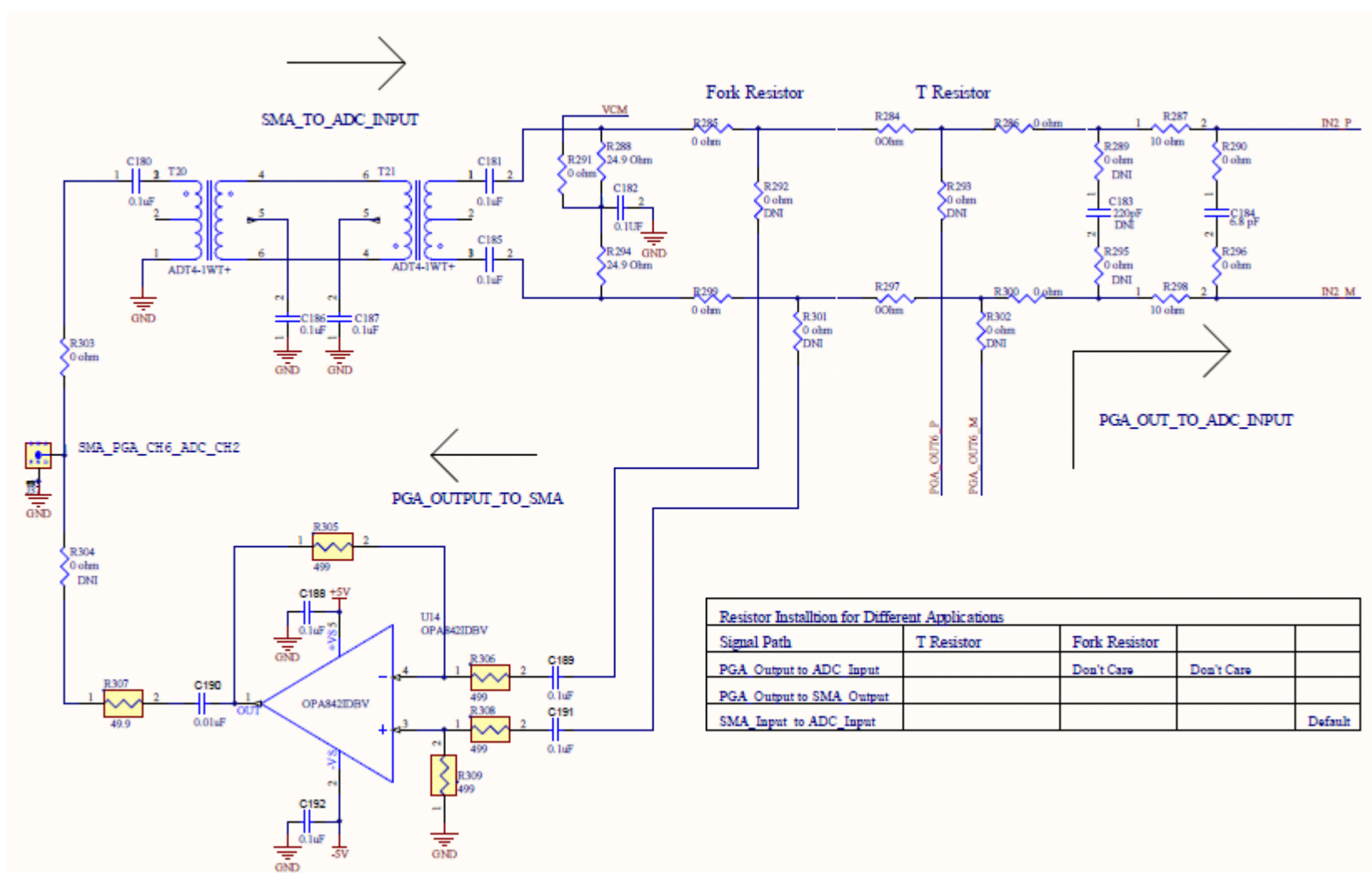
Figure 73. PGA5807 Schematic, (Sh. 11 of 16), PGA_CH6, ADC_CH2
