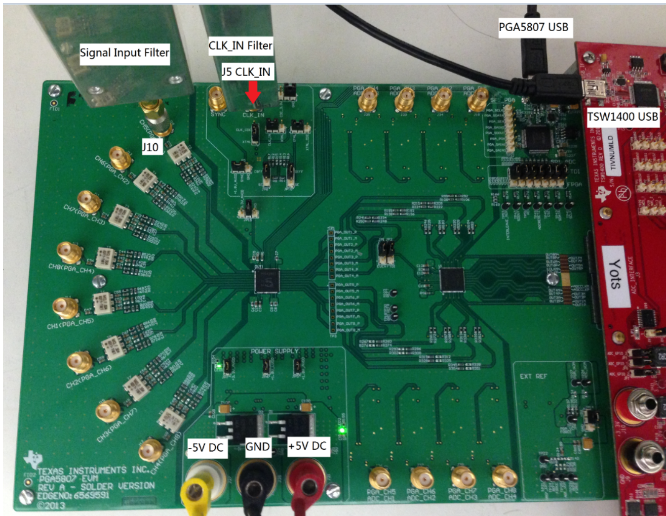
Figure 43. PGA5807 + ADS5296 Gain Test Setup
