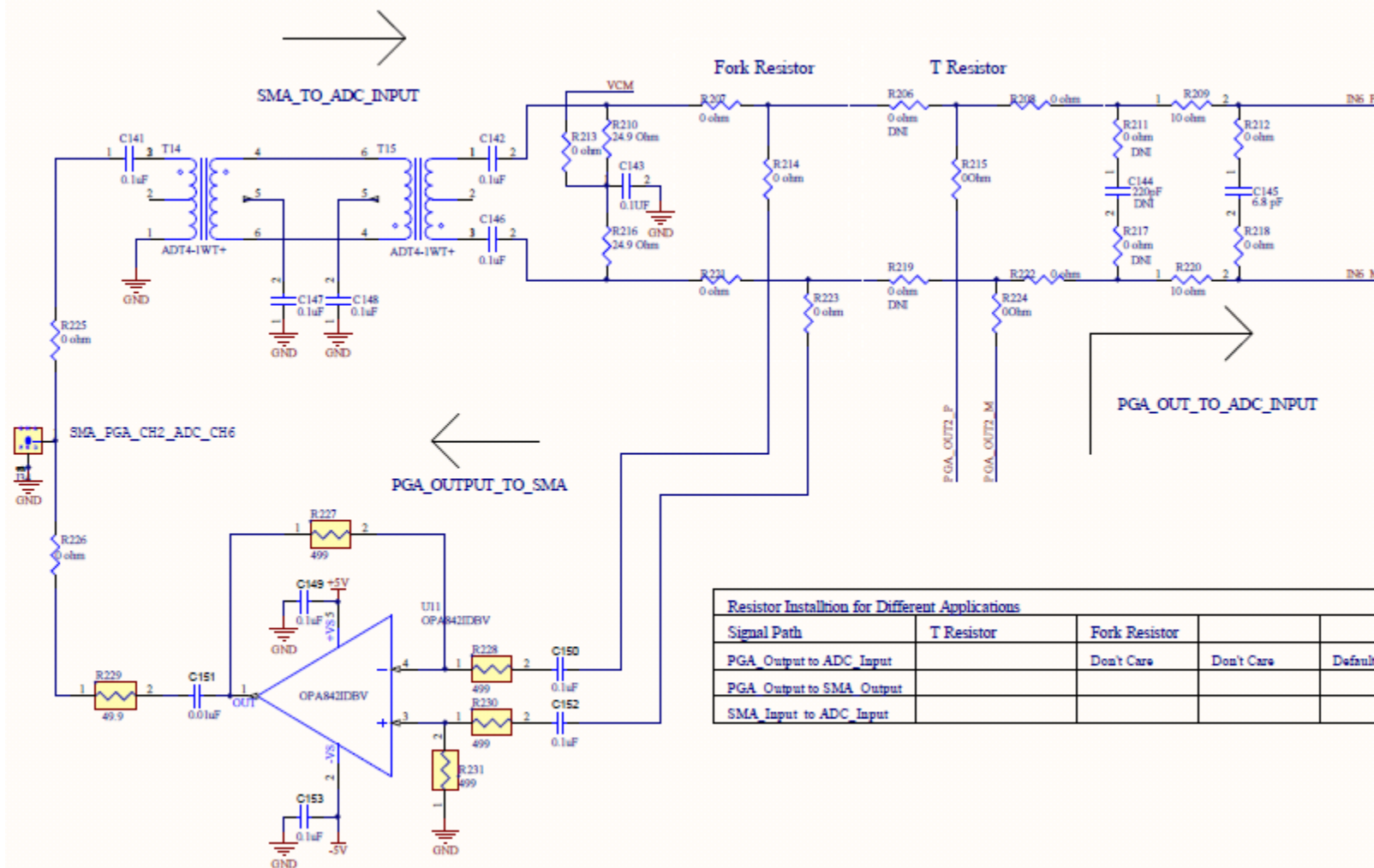
Figure 69. PGA5807 Schematic, (Sh. 7 of 16), PGA_CH2, ADC_CH6
