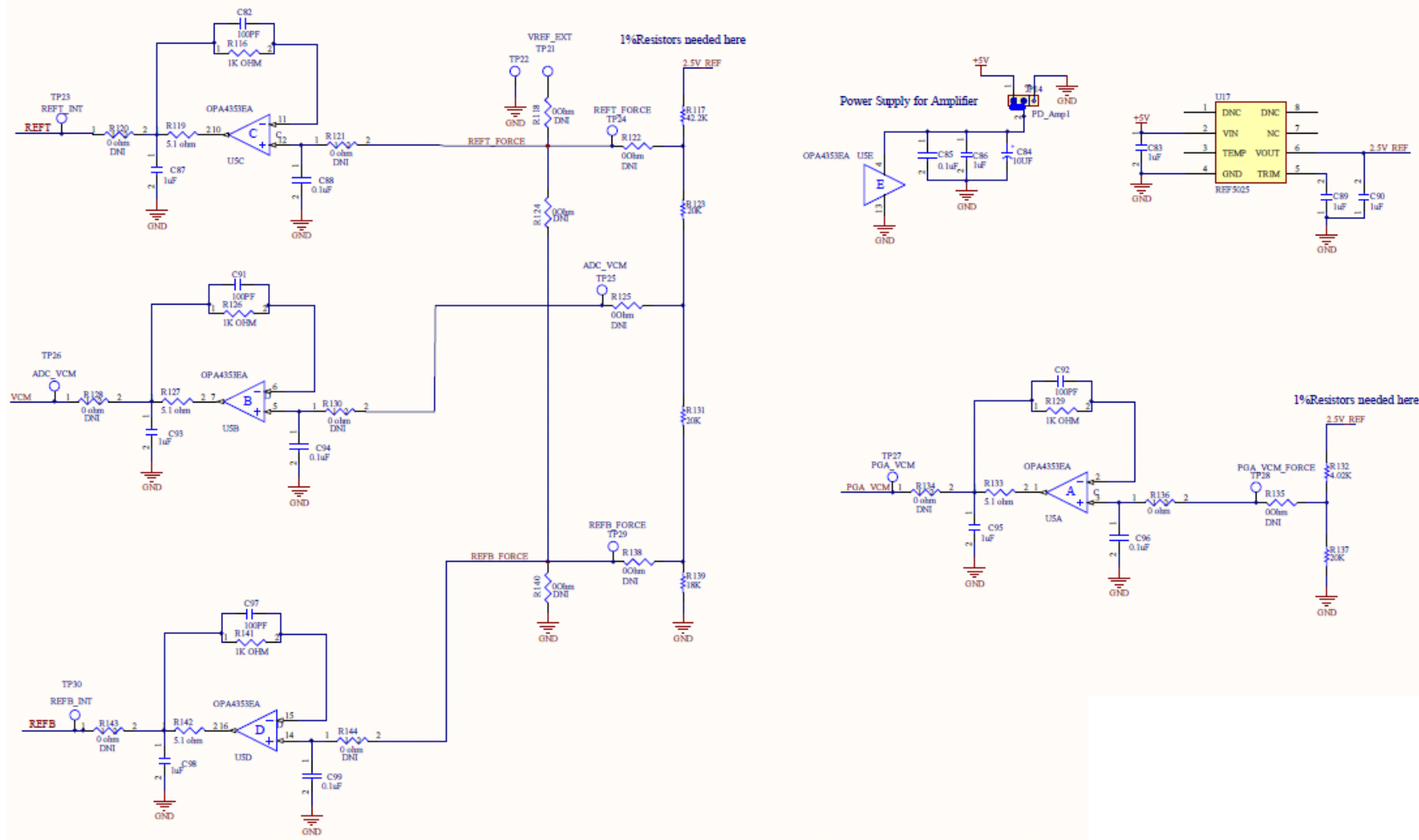
Figure 77. PGA5807 Schematic, (Sh. 15 of 16), ADS5296 External Reference
