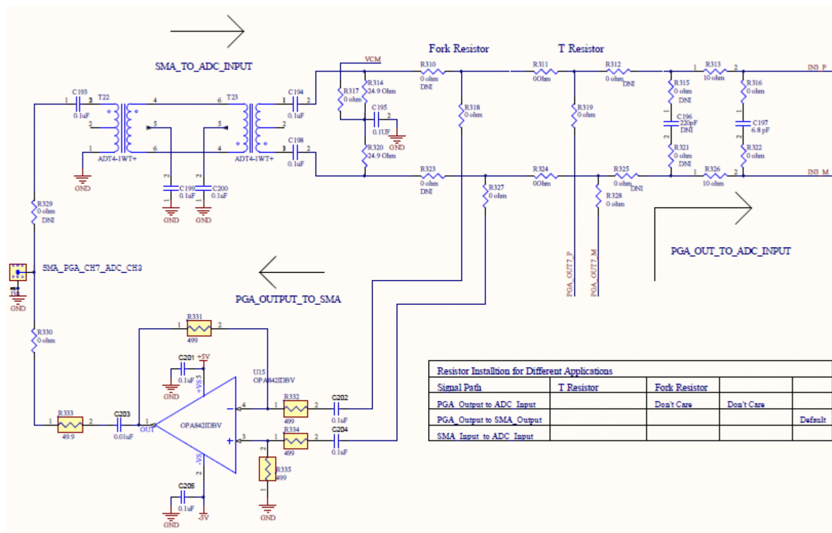
Figure 74. PGA5807 Schematic, (Sh. 12 of 16), PGA_CH7, ADC_CH3
