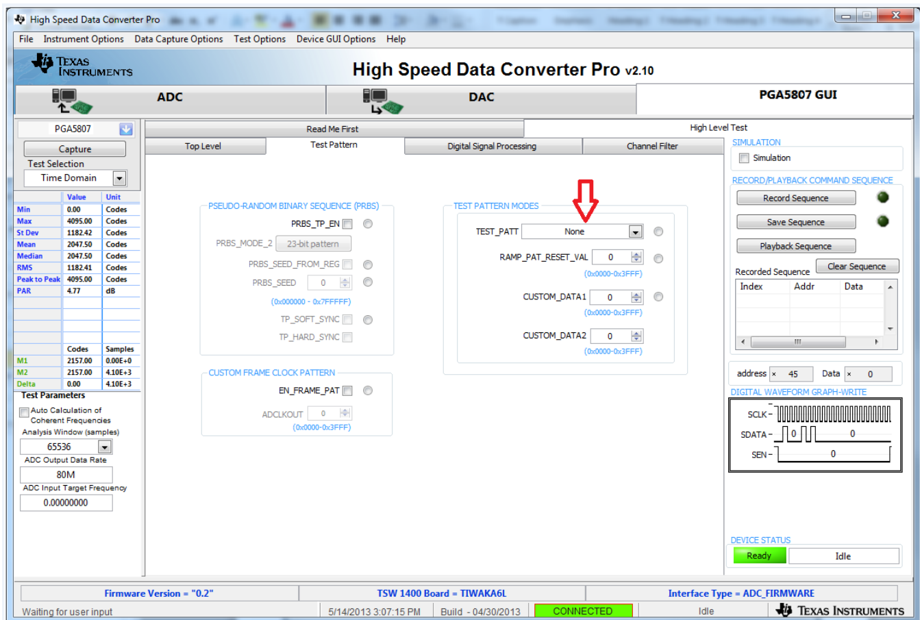
Figure 37. Turn off RAMP Test Pattern
