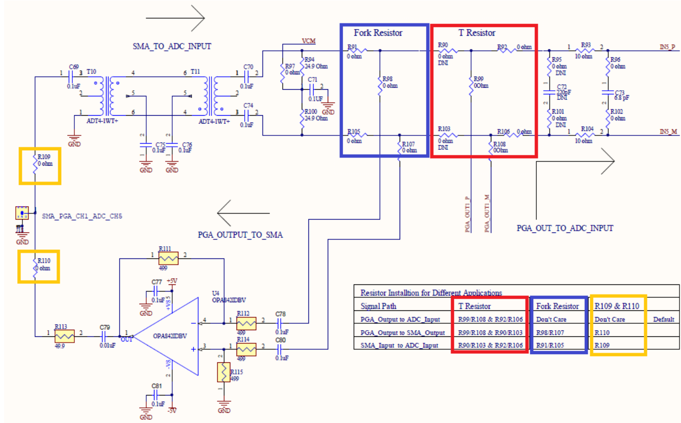
Figure 21. PGA5807 EVM Schematic 0-Ω JUMper Options
