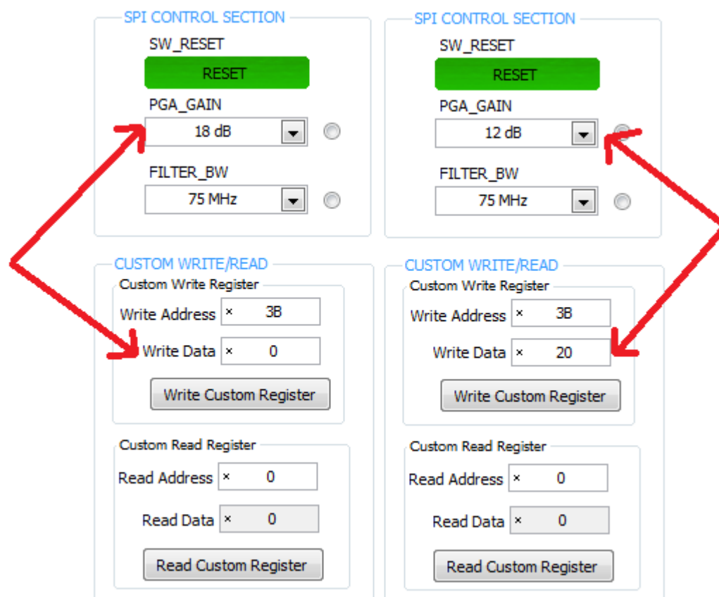
Figure 61. CUSTOM WRITE/READ
