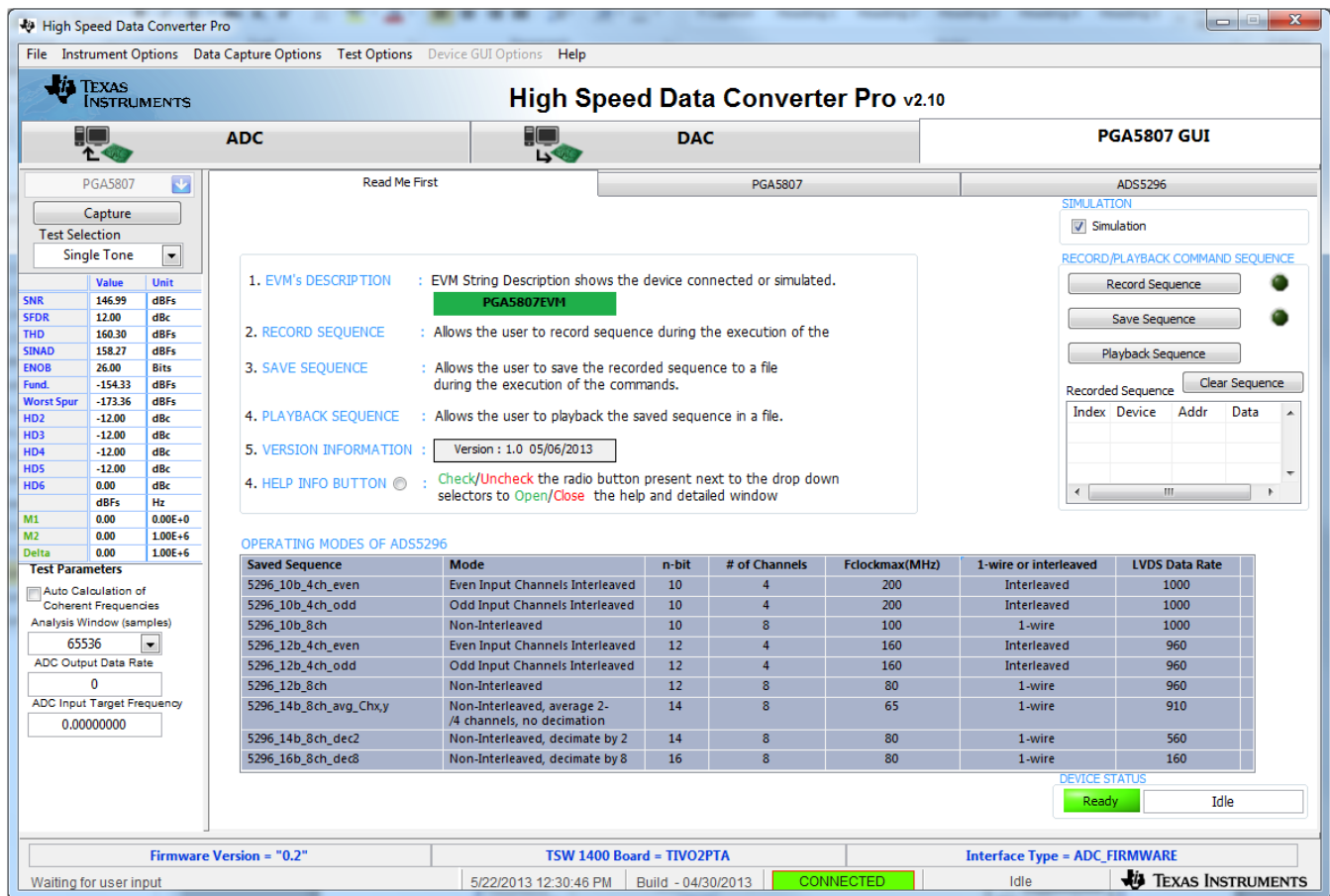
Figure 29. PGA5807 Plug-in GUI Setup (h)
