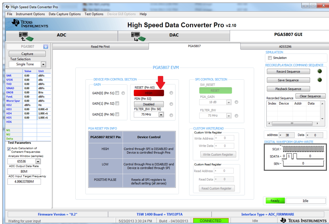
Figure 48. PGA5807 GUI Setup for PGA5807+ADS5296 Gain Test 3
