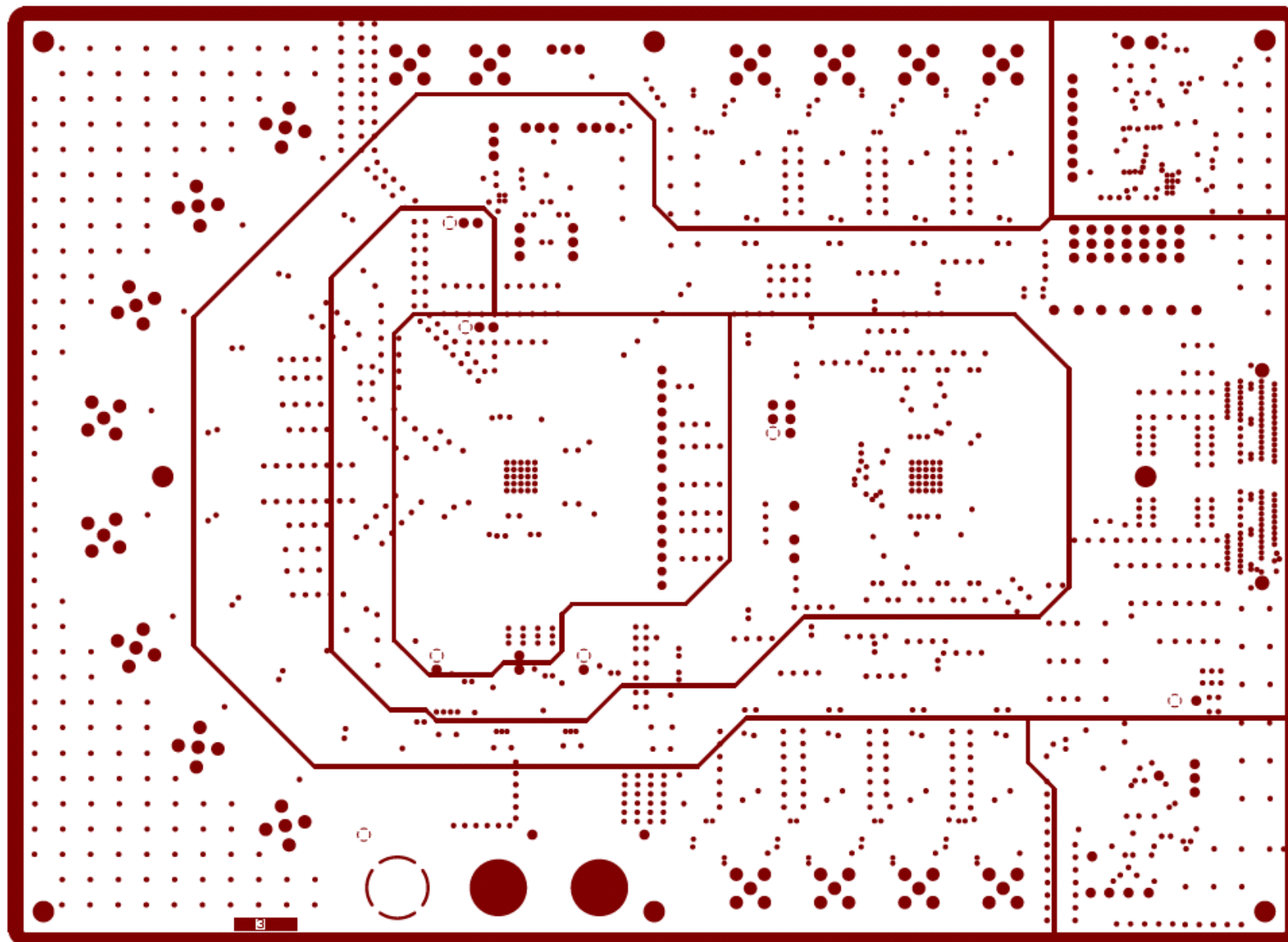
Figure 83. PGA5807 EVM Power Split Plane 1
