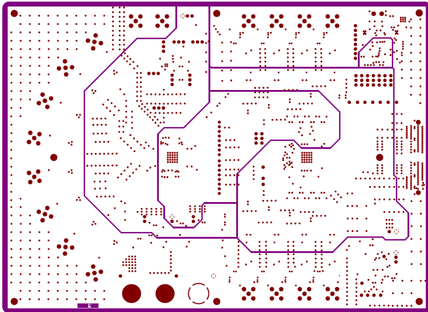
Figure 84. PGA5807 EVM Power Split Plane 2
