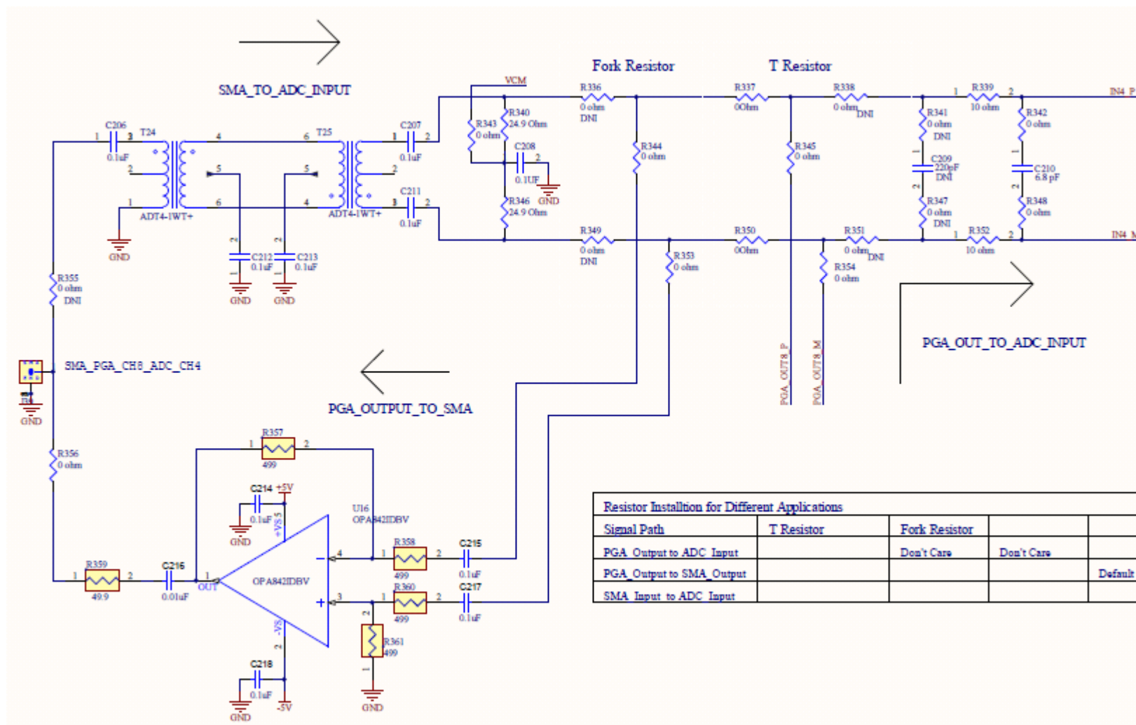
Figure 75. PGA5807 Schematic, (Sh. 13 of 16), PGA_CH8, ADC_CH4
