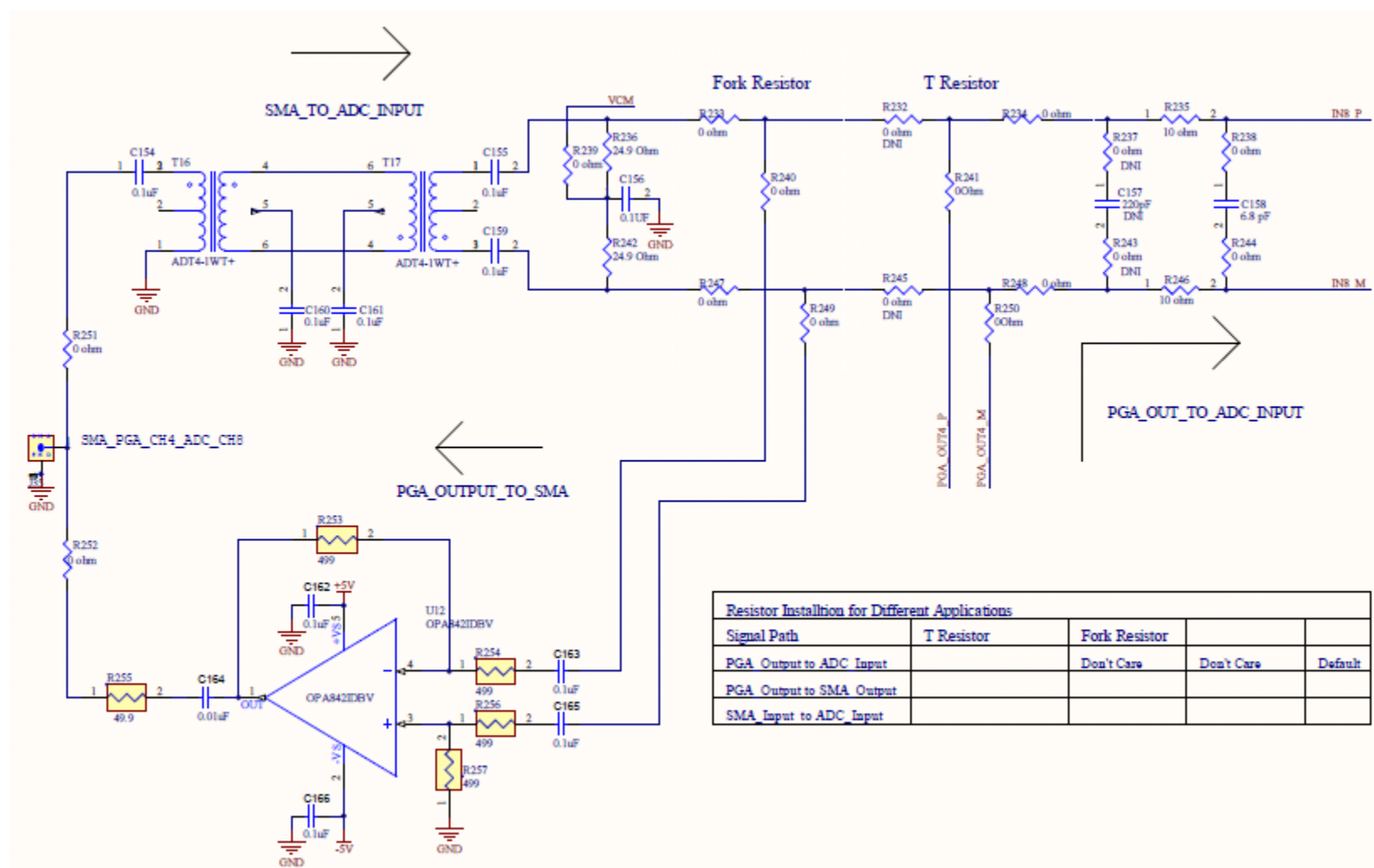
Figure 71. PGA5807 Schematic, (Sh. 9 of 16), PGA_CH4, ADC_CH8
