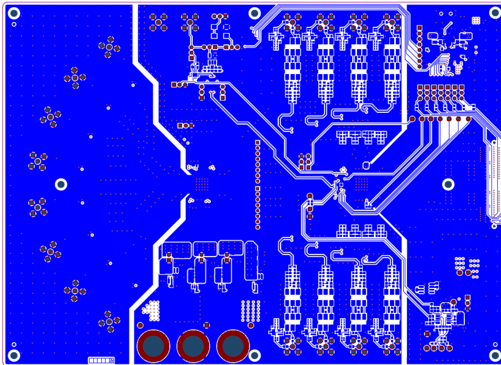
Figure 86. PGA5807 EVM Bottom Side
