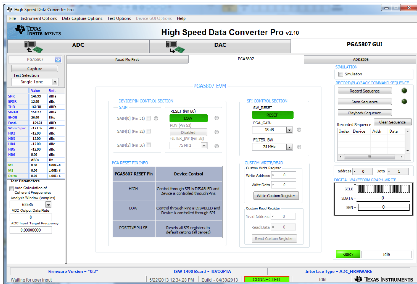
Figure 30. PGA5807 Tab in the PGA5807 GUI
