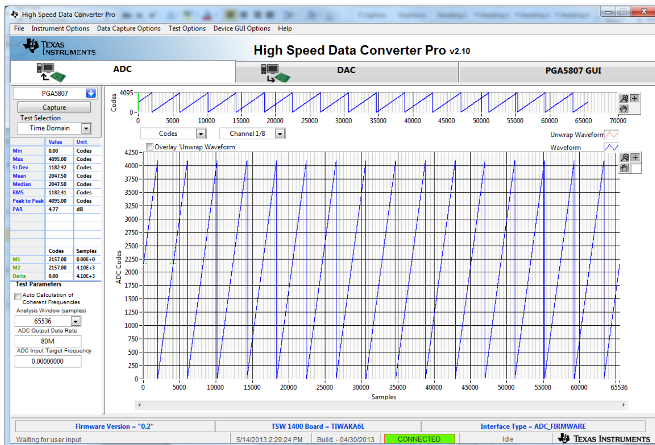
Figure 34. RAMP Capture
