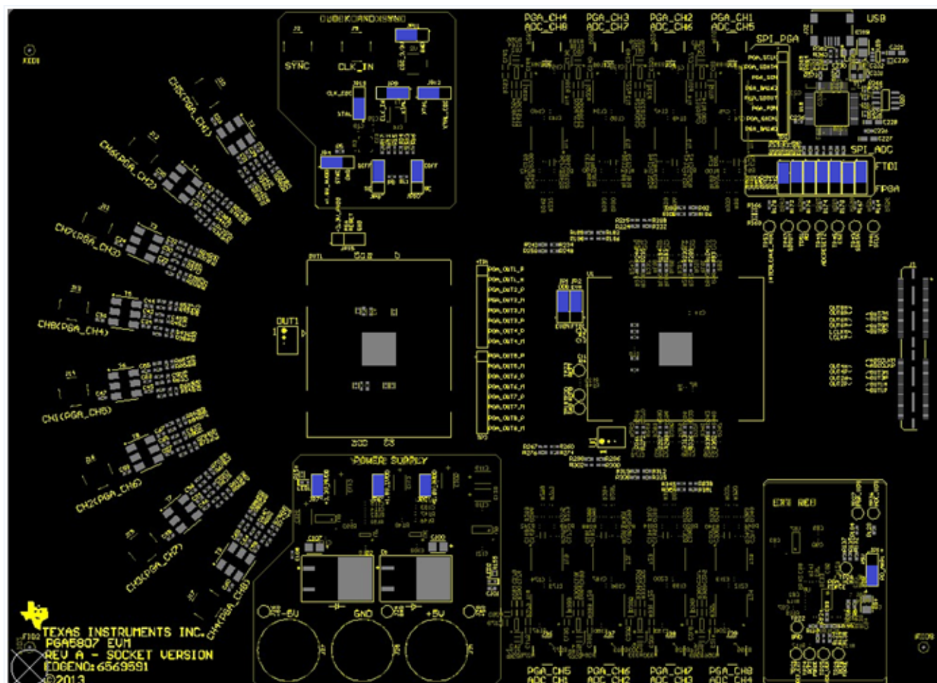
Figure 20. PGA5807 EVM Default Header Configuration
