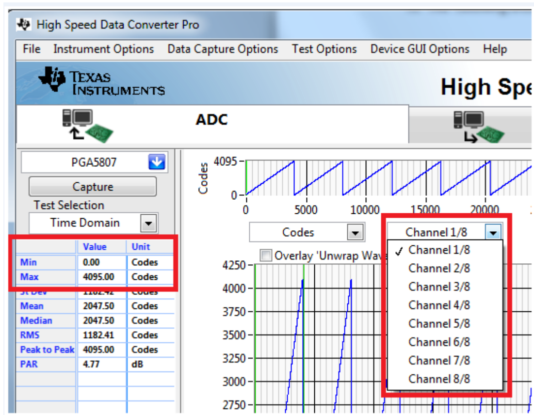
Figure 35. RAMP Capture by Channel
