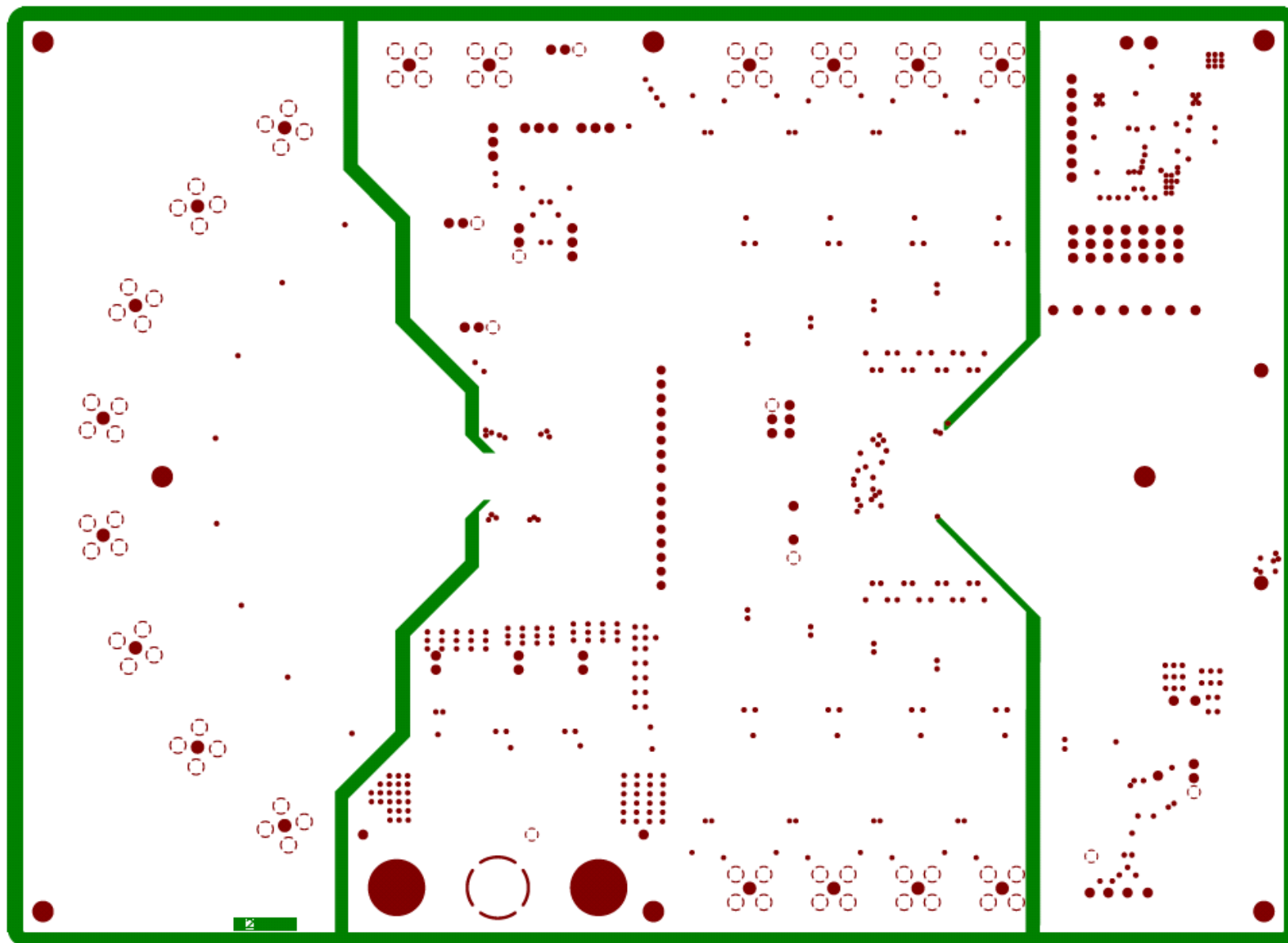
Figure 82. PGA5807 EVM Ground Plane 1
