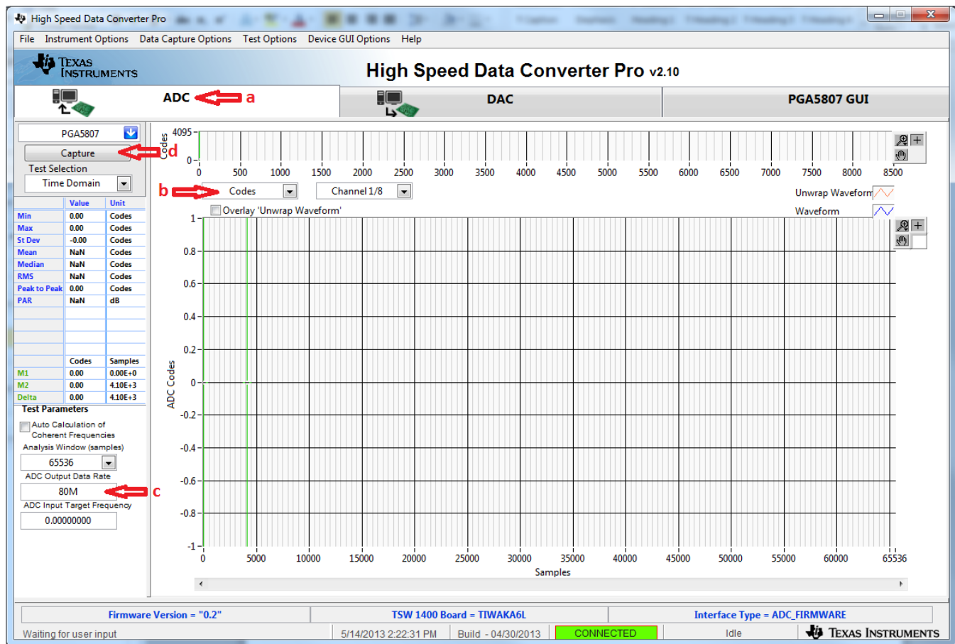
Figure 33. HSDCpro GUI Setup for RAMP Test
