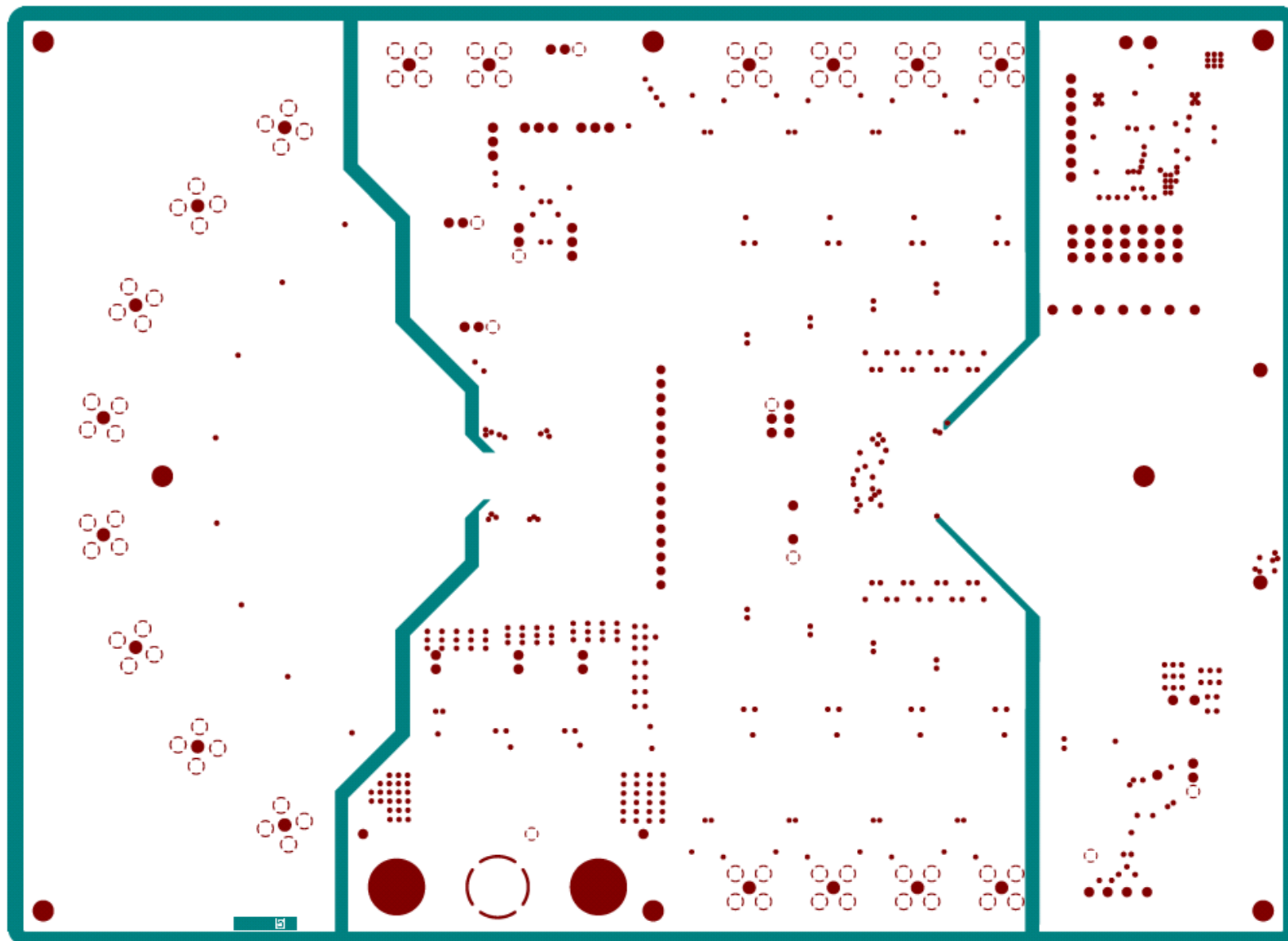
Figure 85. PGA5807 EVM GND Split Plane 2
