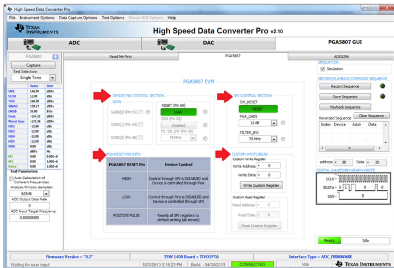
Figure 56. PGA5807 tab
