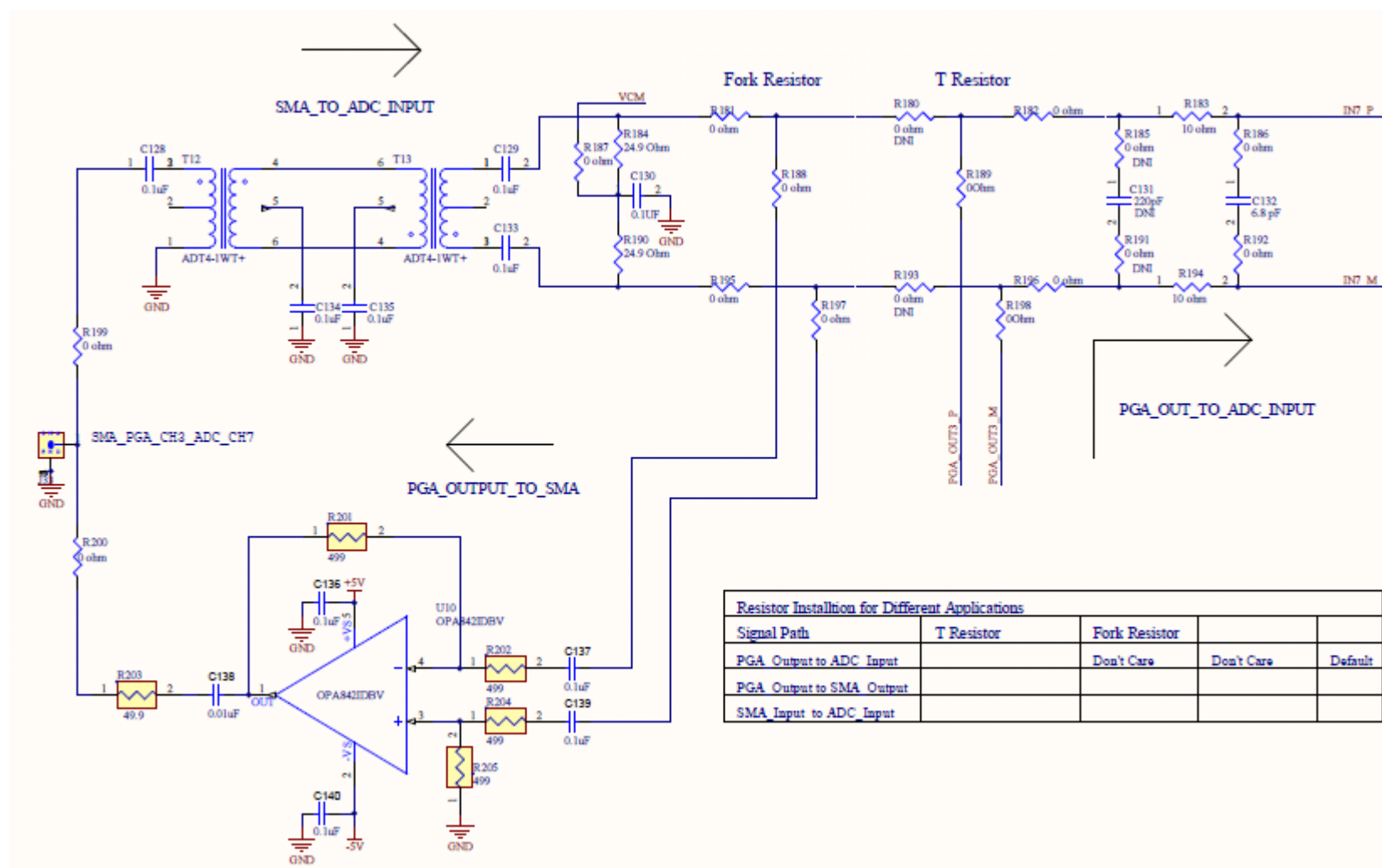
Figure 70. PGA5807 Schematic, (Sh. 8 of 16), PGA_CH3, ADC_CH7
