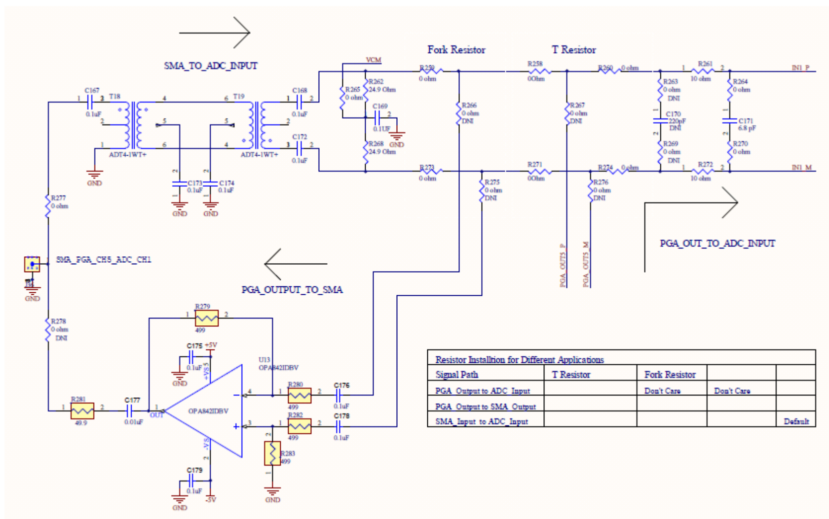
Figure 72. PGA5807 Schematic, (Sh. 10 of 16), PGA_CH5, ADC_CH1
