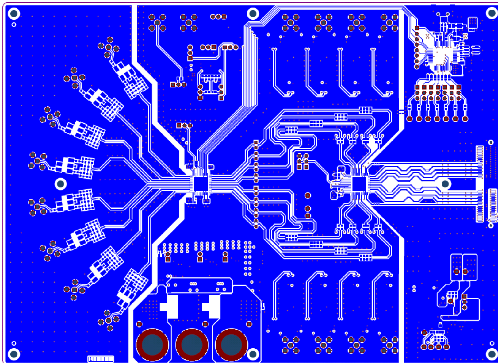
Figure 81. PGA5807 EVM Top Side
