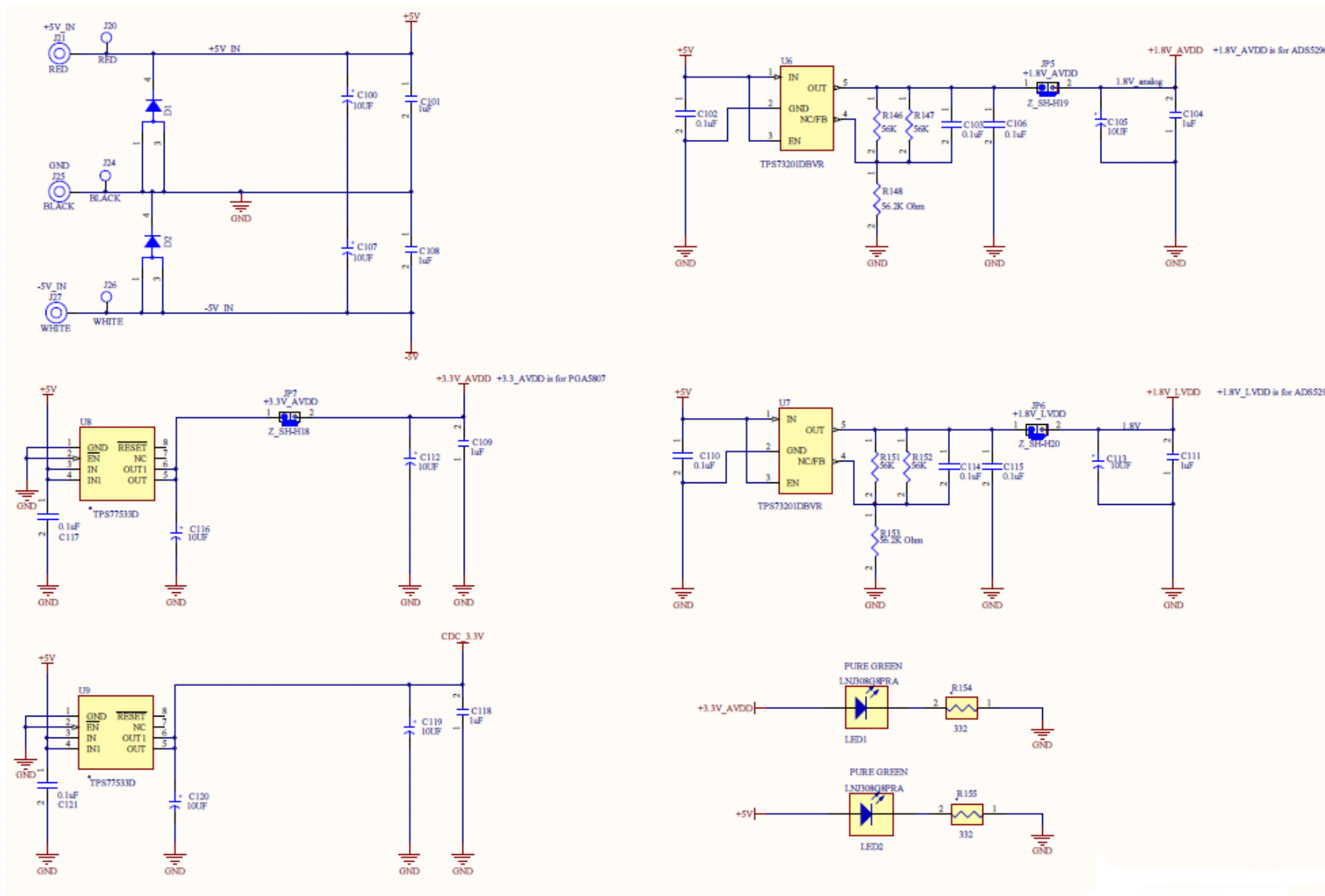
Figure 78. PGA5807 Schematic, (Sh. 16 of 16), Power Supply
