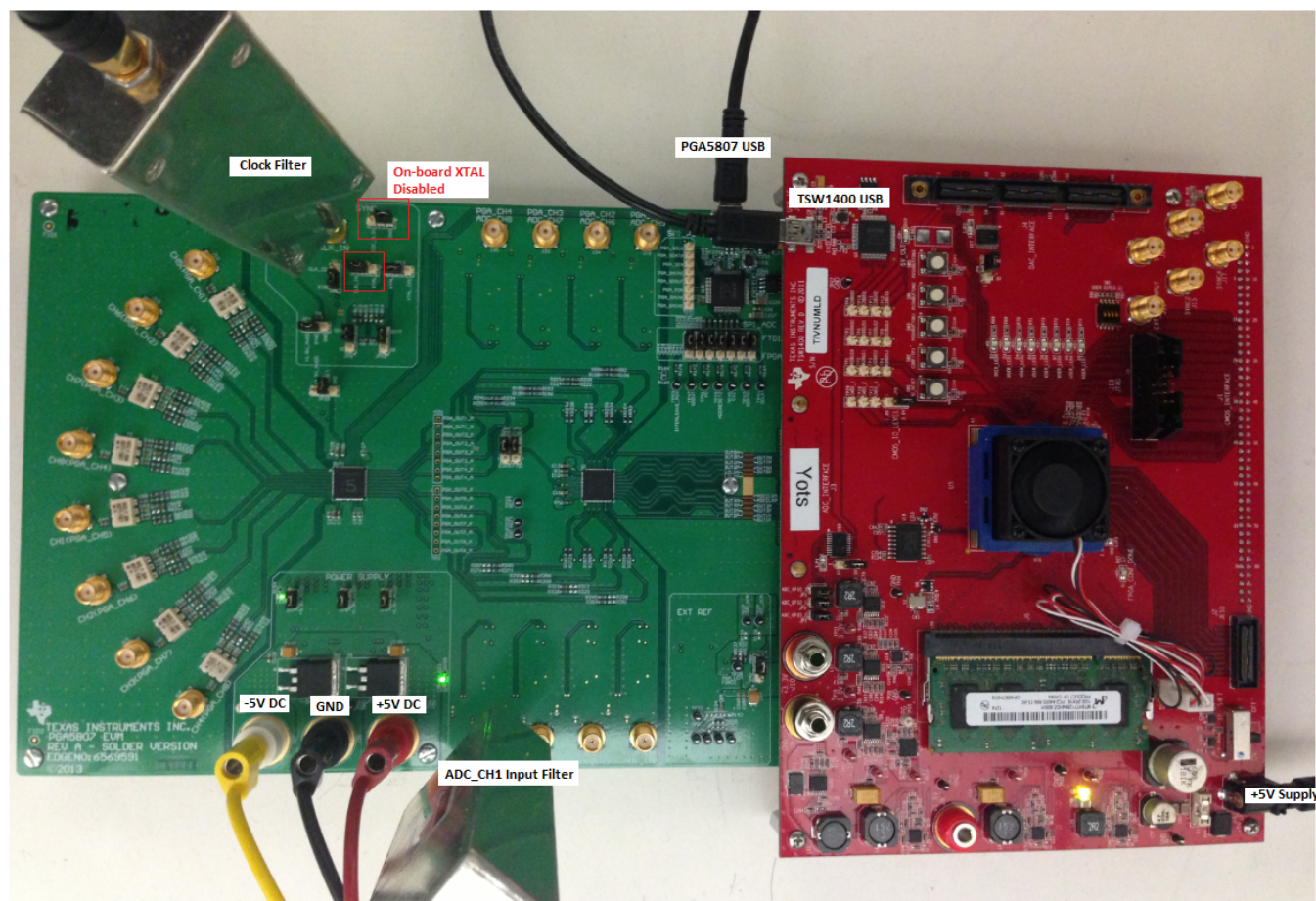
Figure 40. PGA5807 EVM Setup for ADS5296 Only Testing
