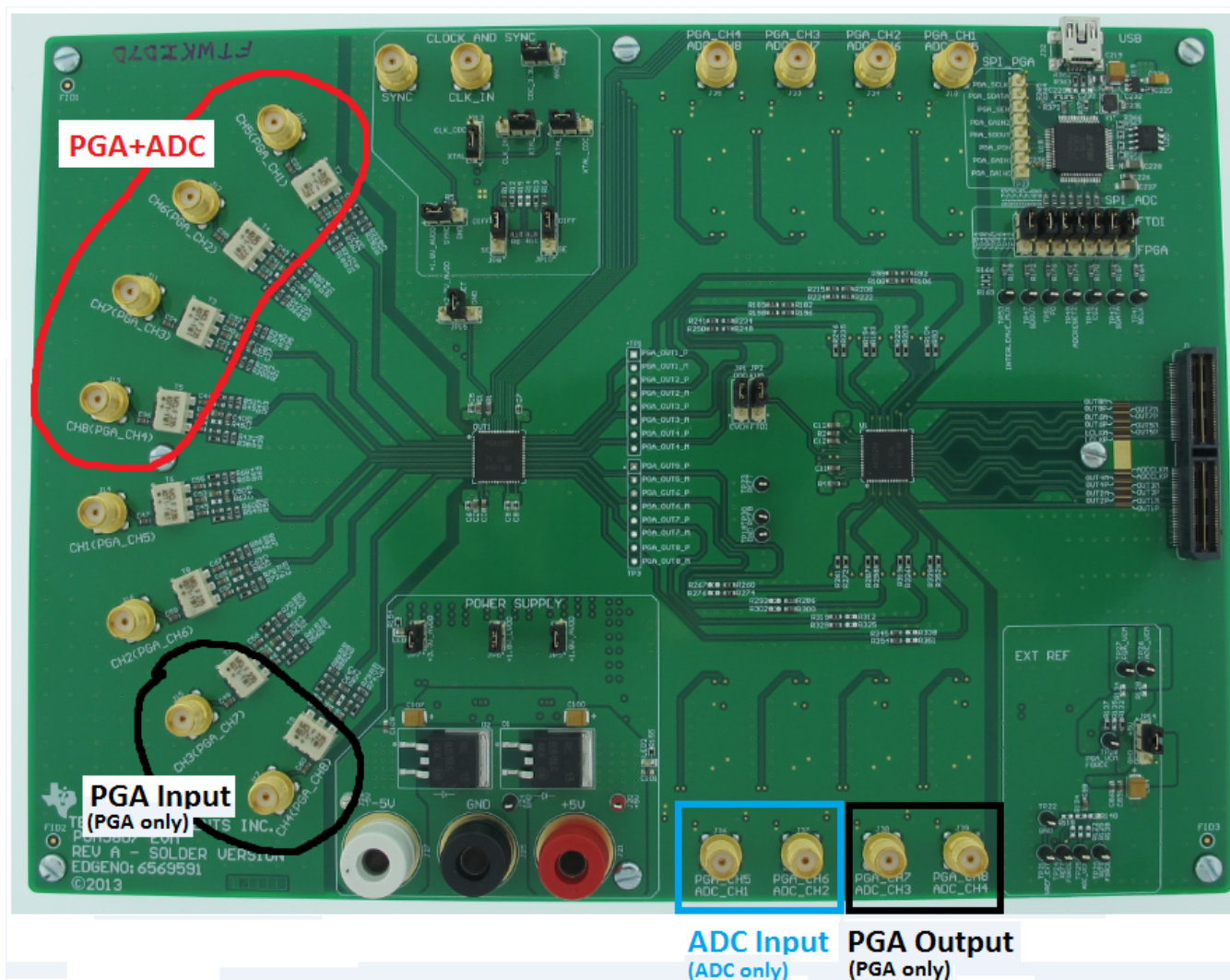
Figure 18. PGA5807 EVM Configuration
