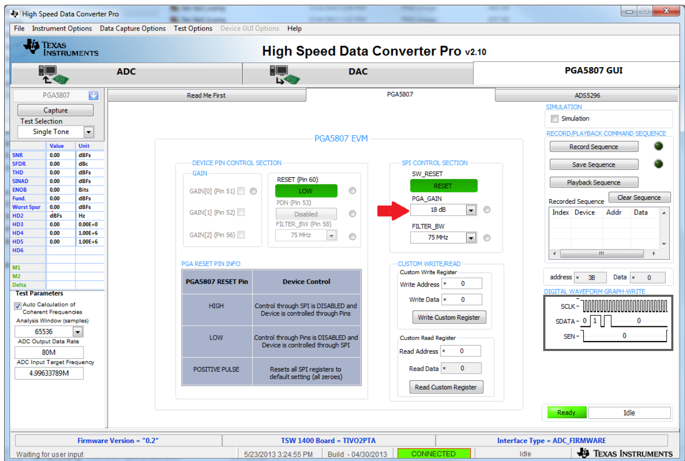
Figure 44. PGA5807 GUI Setup for PGA5807+ADS5296 1
