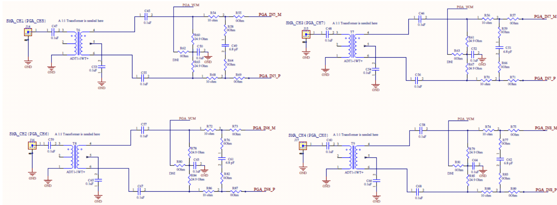
Figure 67. PGA5807 Schematic, (Sh. 5 of 16), PGA5807 Analog Inputs Ch5-8
