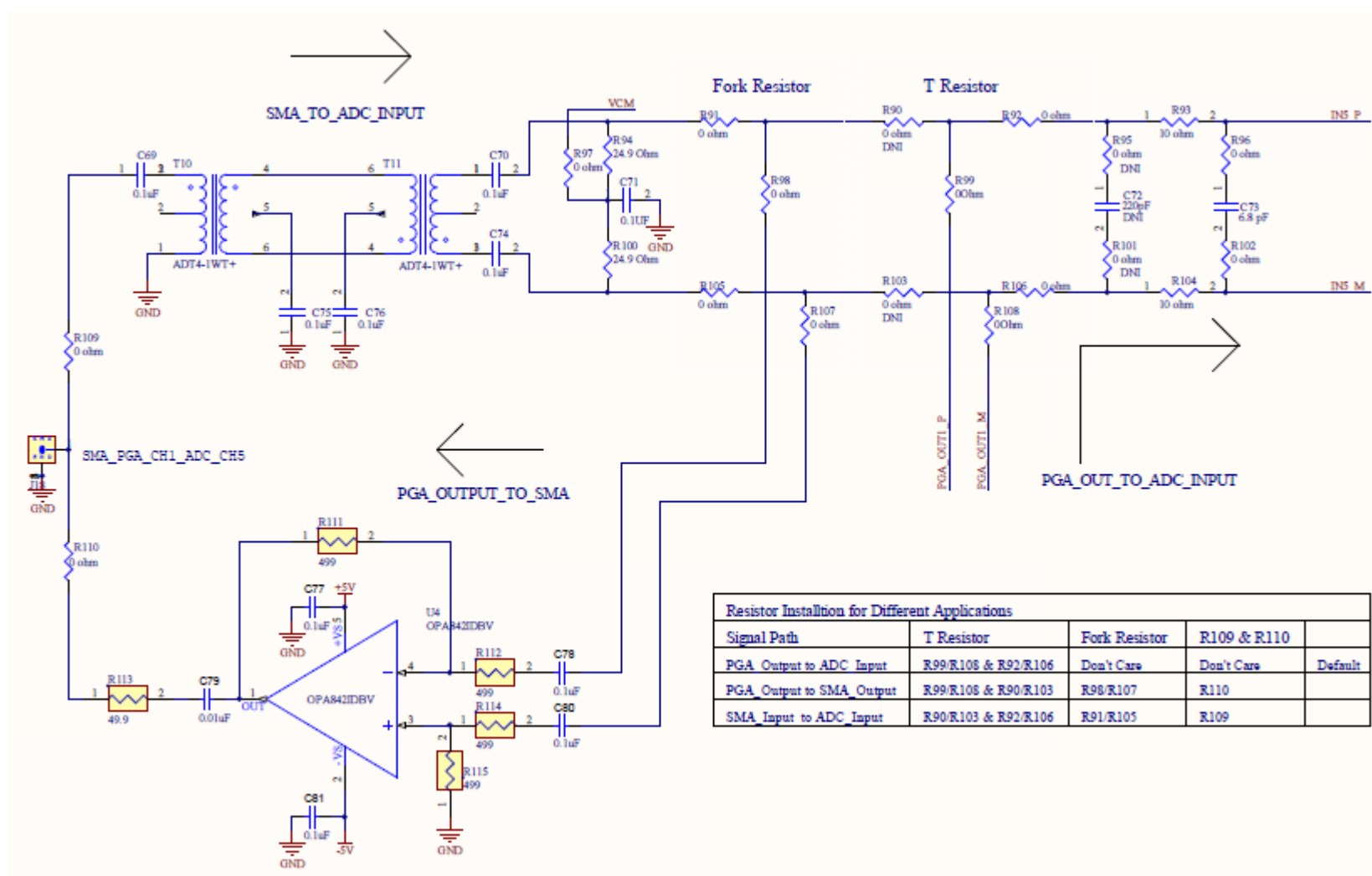
Figure 68. PGA5807 Schematic, (Sh. 6 of 16), PGA_CH1, ADC_CH5
