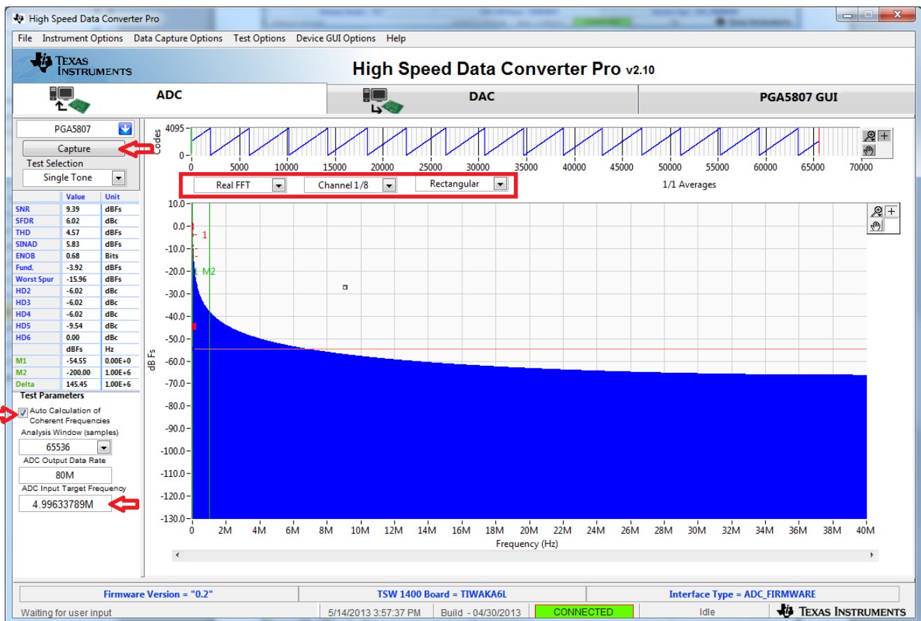
Figure 41. HSDCpro GUI Setup
