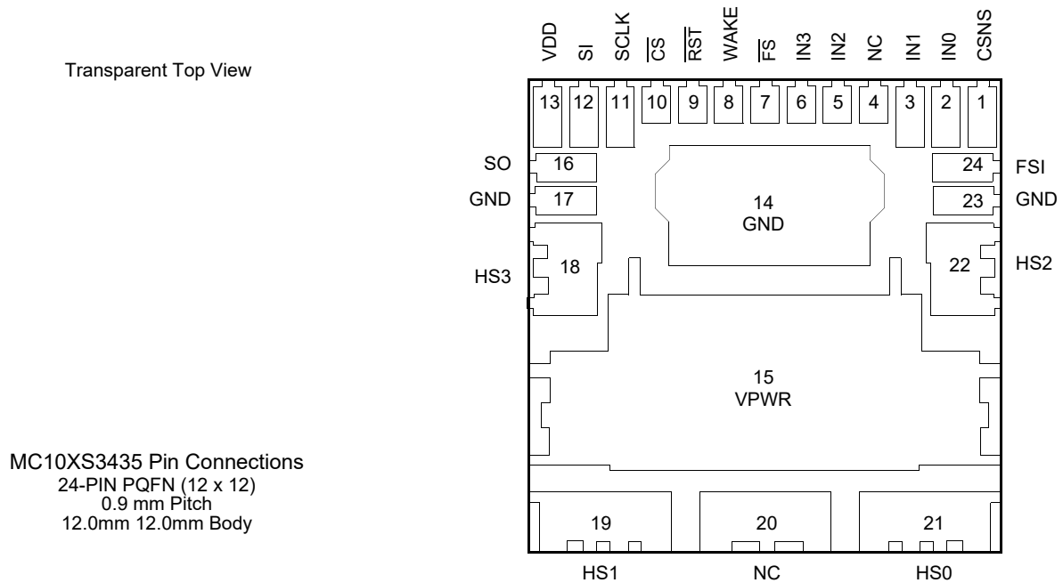
Figure 23. Pin connections
