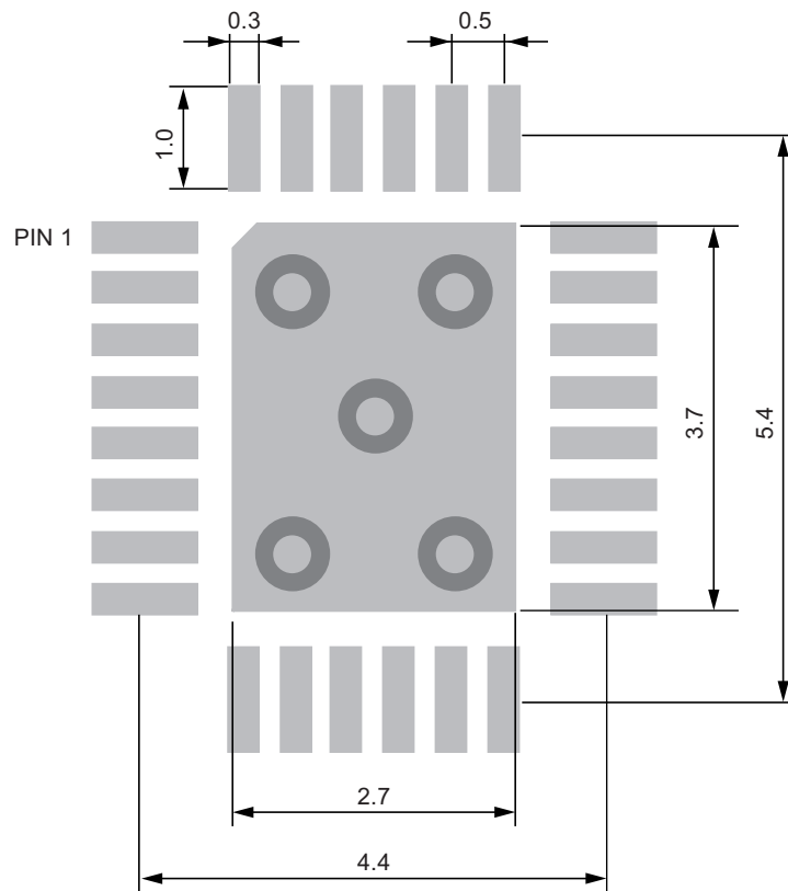
Figure 8-4. Recommended Footprint
