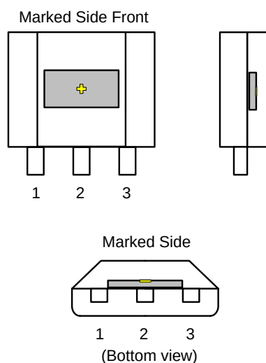
Figure 26. TO-92 (LPG, LPE) Package
