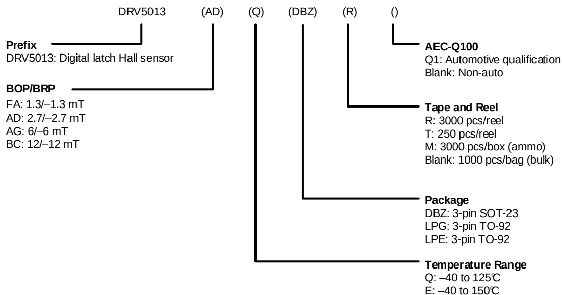
Figure 24. Device Nomenclature
