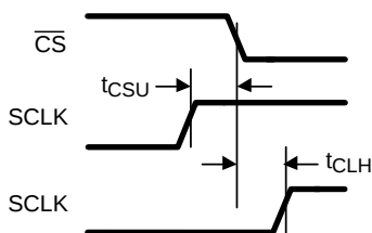
Figure 4. SCLK and \overline{\text{CS}} Timing Parameters
