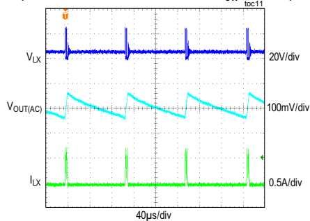
STEADY STATE (5V OUTPUT, PFM MODE, 20mA LOAD, f_{SW} = 400kHz )
