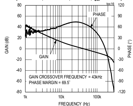
CLOSED-LOOP BODE PLOT (5V OUTPUT, PWM MODE, 2A LOAD, f_{SW} = 400kHz )
