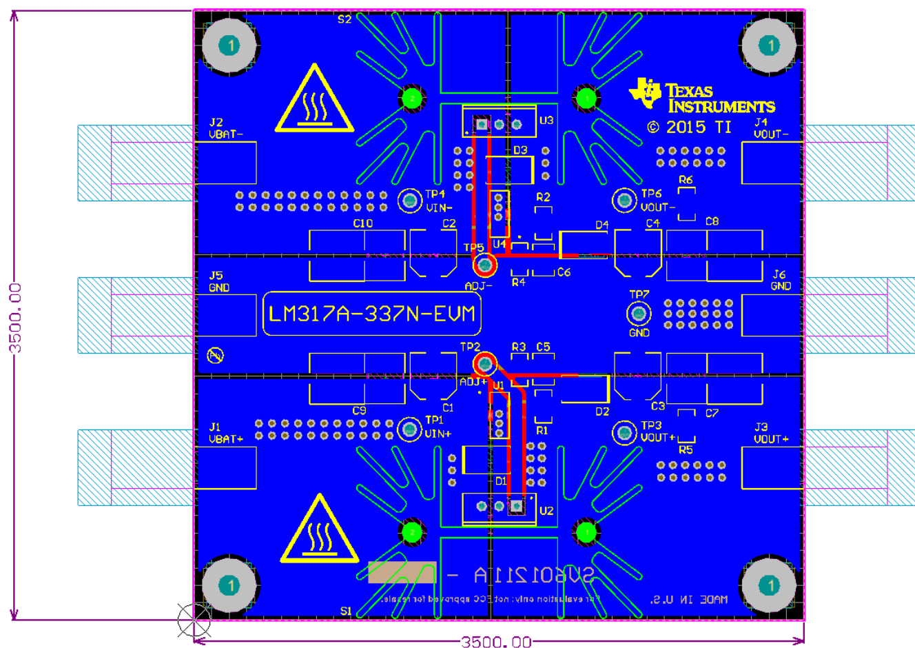
Figure 4-2. Bottom Layer Layout
