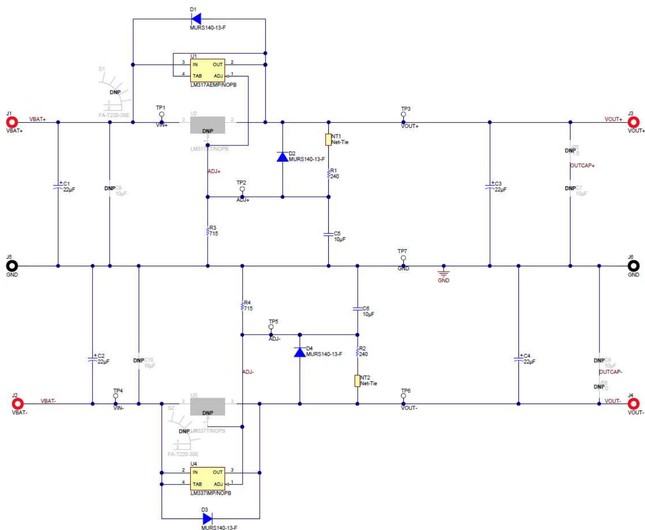
Figure 5-1. LM317N-LM337N10EVM Schematic
