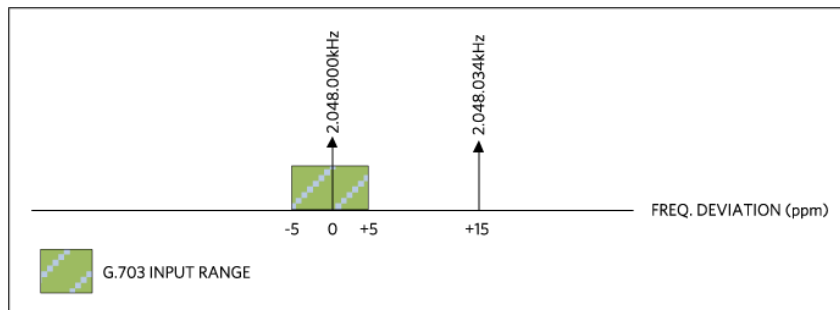
Figure 8. MCLK frequency selection according to input signal range can avoid wander on RCLK.
