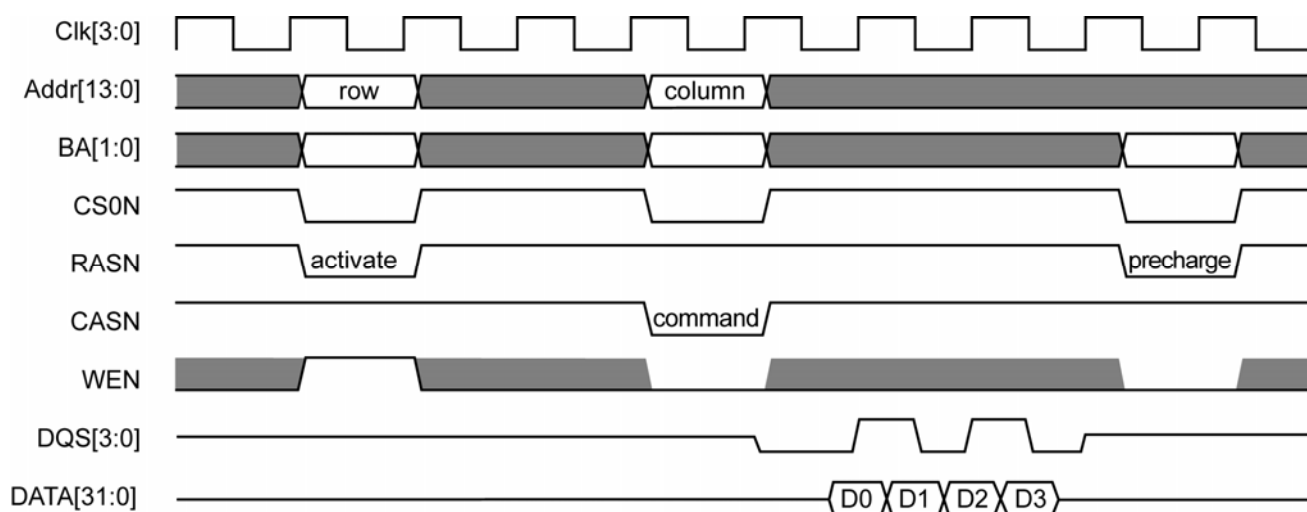
Figure 11. Burst DDR Write Timing
