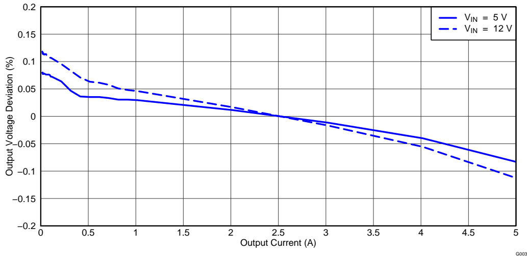
Figure 3. TPS54527EVM-052 Load Regulation, V_{IN} = 5V and V_{IN} = 12V .
