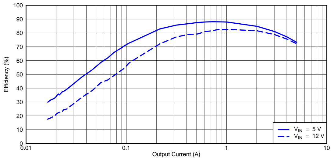
Figure 2. TPS54527EVM-052 Light-Load Efficiency
