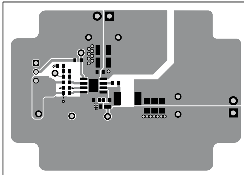
Figure 13. Top Layer
