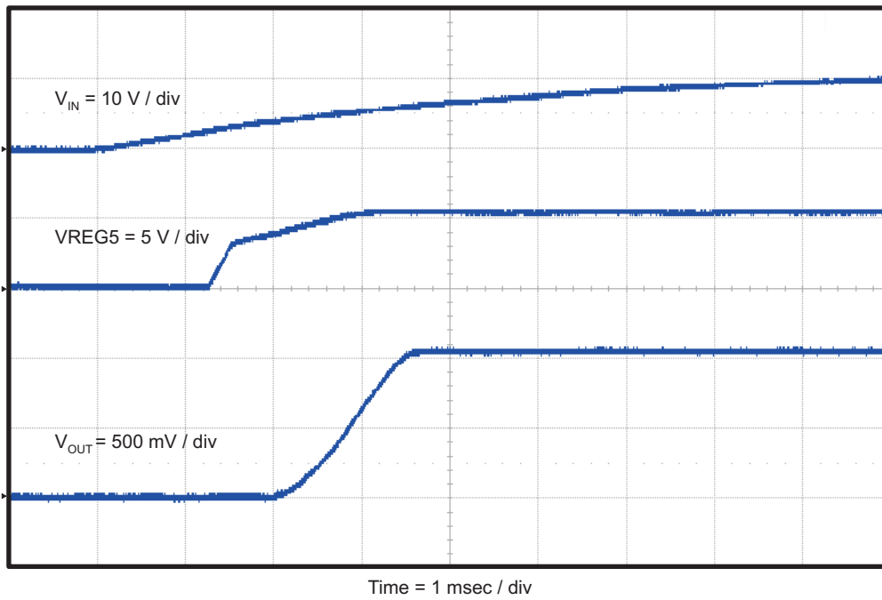
Figure 9. TPS54527EVM-052 Start-Up Relative to V_{IN} With VREG5
