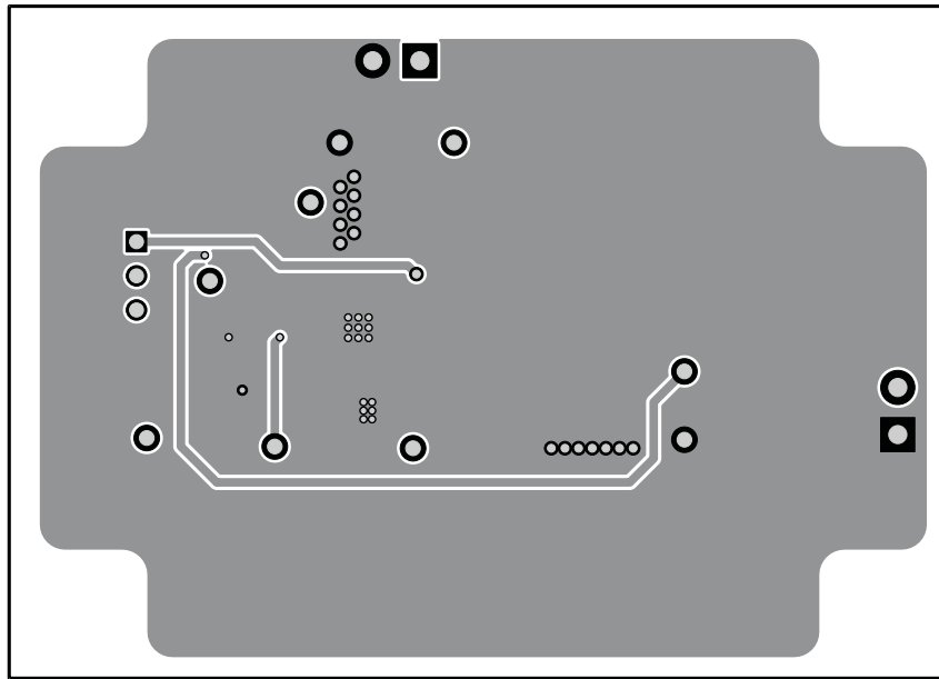
Figure 16. Bottom Layer
