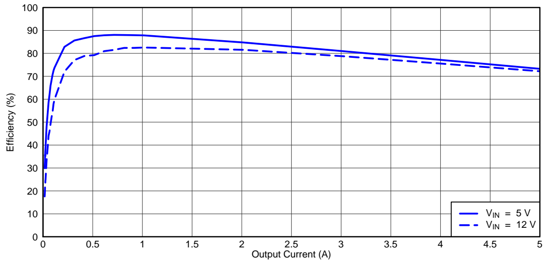
Figure 1. TPS54527EVM-052 Efficiency
