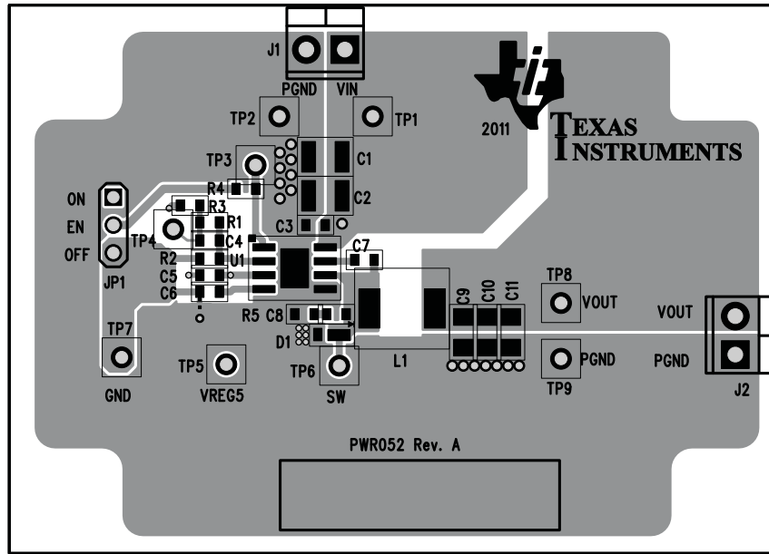
Figure 12. Top Assembly
