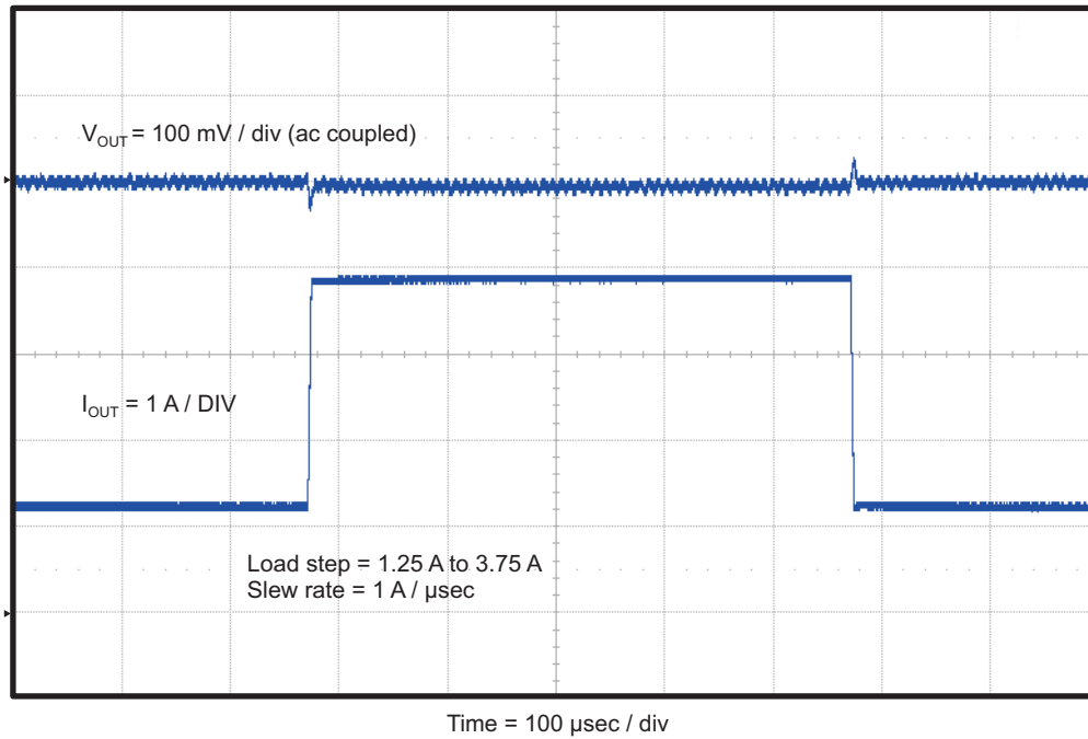
Figure 5. TPS54527EVM-052 Load Transient Response
