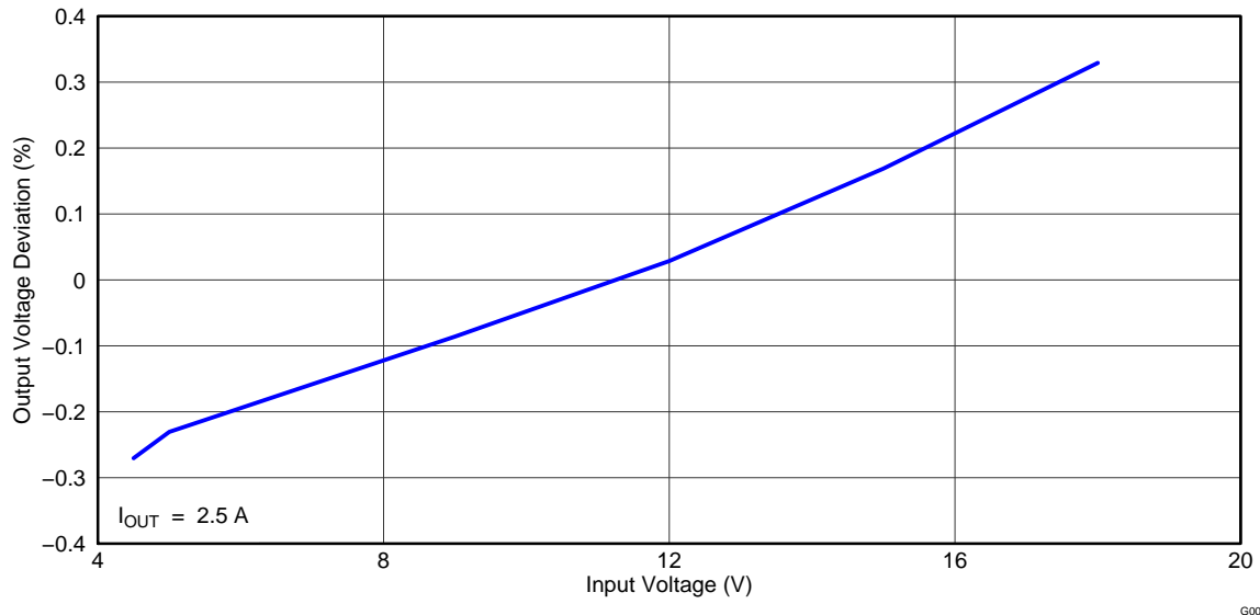
Figure 4. TPS54527EVM-052 Line Regulation
