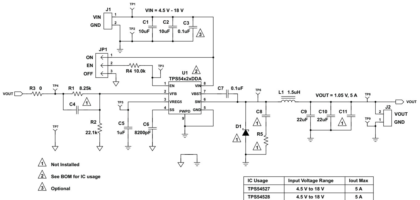
Figure 17. TPS54527EVM-052 Schematic Diagram
