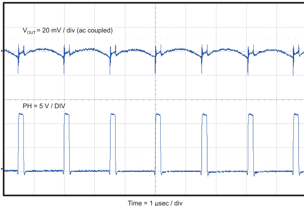
Figure 6. TPS54527EVM-052 Output Voltage Ripple
