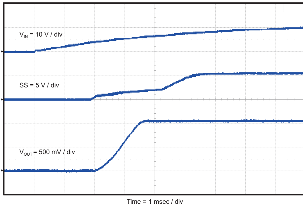
Figure 8. TPS54527EVM-052 Start-Up Relative to V_{IN} With SS
