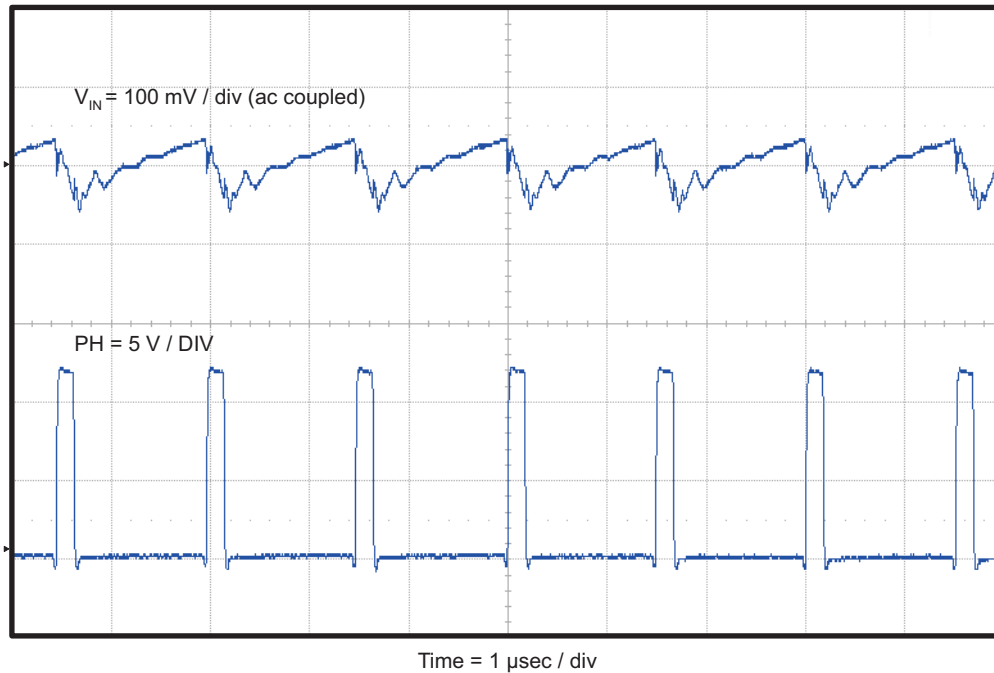
Figure 7. TPS54527EVM-052 Input Voltage Ripple
