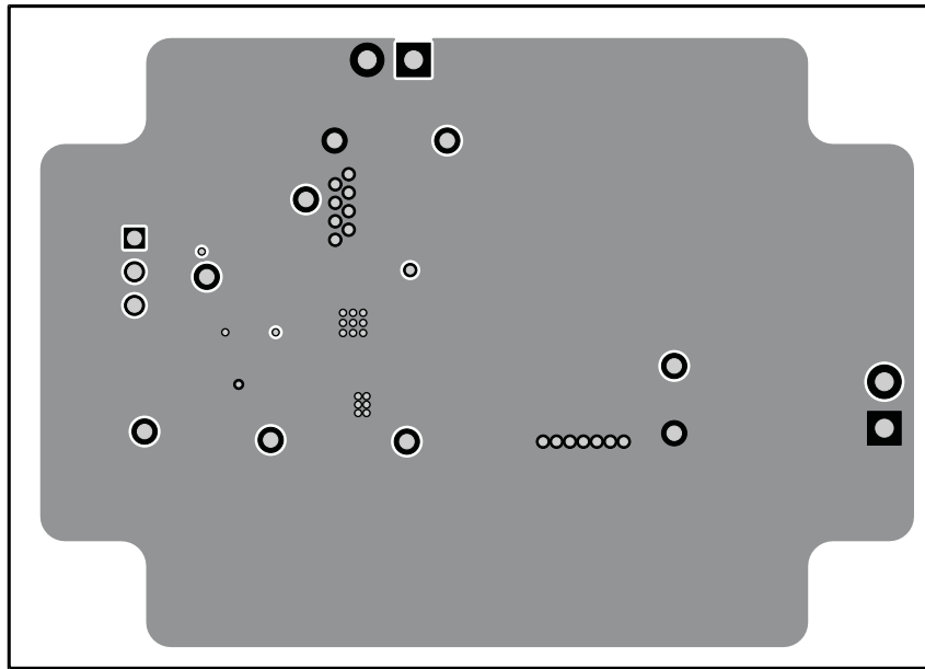
Figure 14. Internal Layer 1
