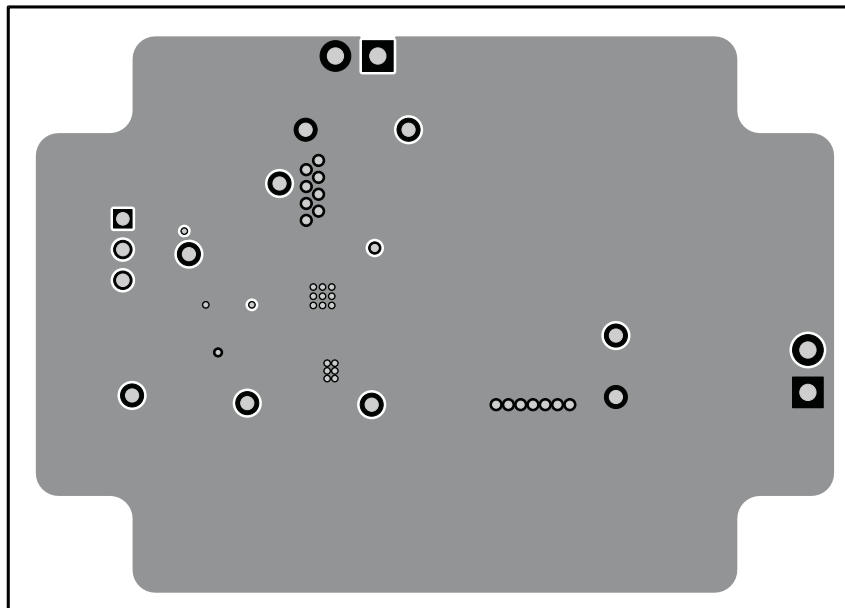
Figure 15. Internal Layer 2
