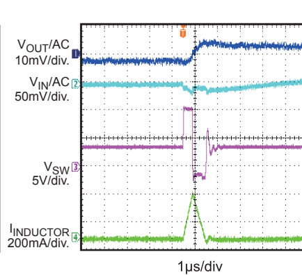
Input/Output Ripple I_{OUT}=0A
