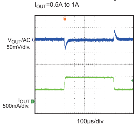
Load Transient Response I_{OUT}=0.5A to 1A
