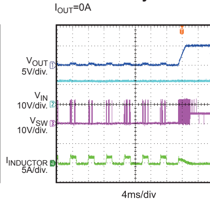
OCP Recovery I_{OUT}=0A
