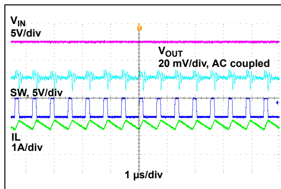
FIGURE 2-28: Switching Waveforms - I_{OUT} = 3A .
