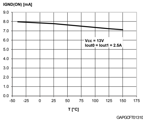
Figure 17: IGND(ON) vs. Iout
