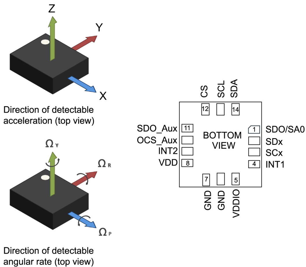
Figure 4. Pin connections
